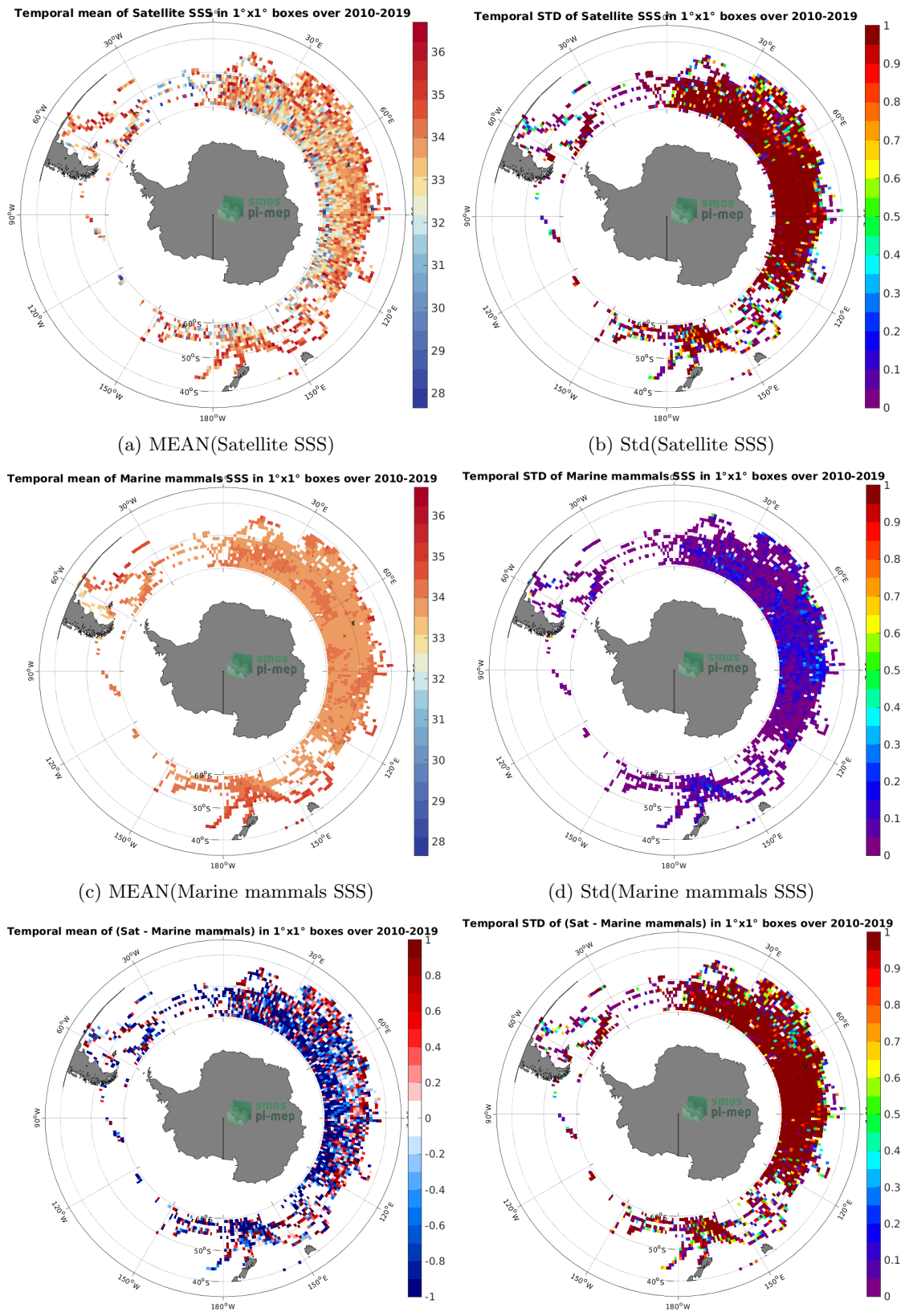
Figure 6: Temporal mean (left) and Std (right) of SSS from SMOS SSS L2 v700 (ESA) (top), Marine mammals (middle), and of \Delta SSS (Satellite - Marine mammals). Only match-up pairs are used to generate these maps.
