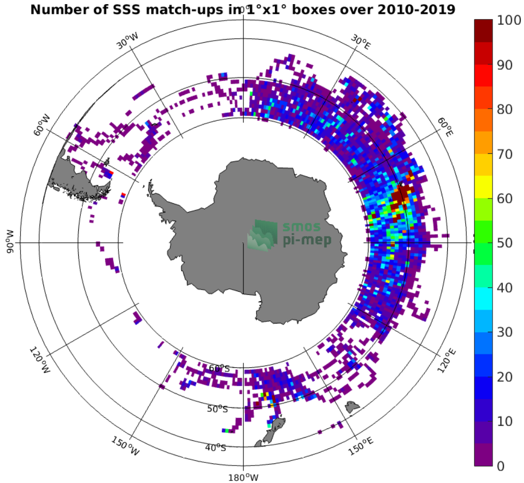
Figure 4: Number of SSS match-ups between Marine mammals SSS and the SMOS SSS L2 v700 (ESA) SSS product for the Roaring Forties and Furious Fifties Pi-MEP region over 1^\circ \times 1^\circ boxes and for the full satellite product period.
