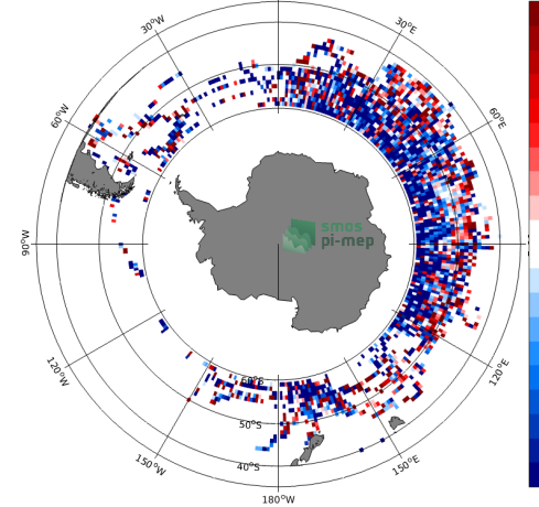
(e) MEAN( \Delta SSS) (Satellite - Marine mammals)
