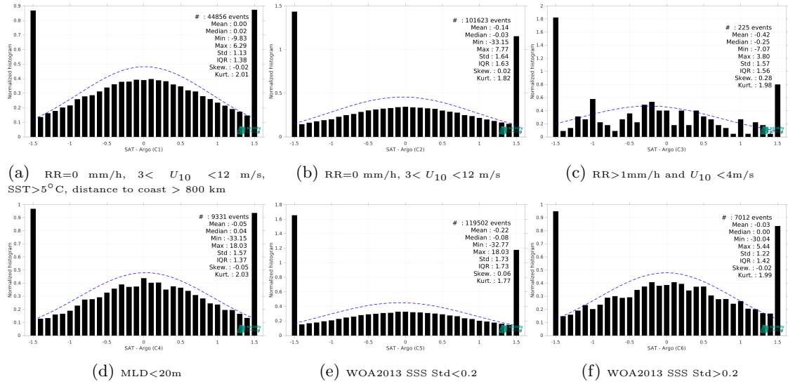
Figure 15: Normalized histogram of \Delta SSS (SMOS SSS L2 v700 (ESA) - Argo) for 6 different subdatasets corresponding to: RR=0 mm/h, 3 < U_{10} < 12 m/s, SST > 5°C, distance to coast > 800 km (a), RR=0 mm/h, 3 < U_{10} < 12 m/s (b), RR > 1mm/h and U_{10} < 4 m/s (c), MLD < 20m (d), WOA2013 SSS Std < 0.2 (e), WOA2013 SSS Std > 0.2 (f).
