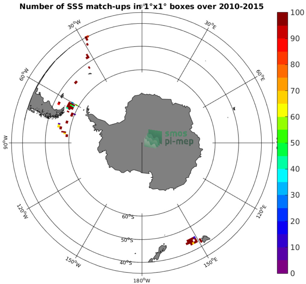
Figure 4: Number of SSS match-ups between TSG-SAMOS SSS and the SMOS-L2-DPGS-v662 SSS product for the Roaring Forties and Furious Fifties Pi-MEP region over 1°x1° boxes and for the full satellite product period.
