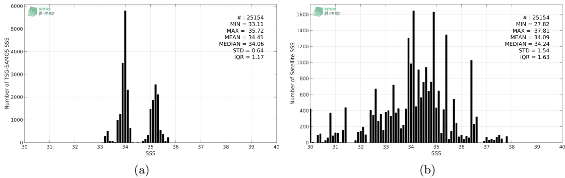
Figure 2: Histograms of SSS from TSG-SAMOS (a) and SMOS-L2-DPGS-v662 (b) considering all match-up pairs per bins of 0.1 over the Roaring Forties and Furious Fifties Pi-MEP region and for the full satellite product period.
