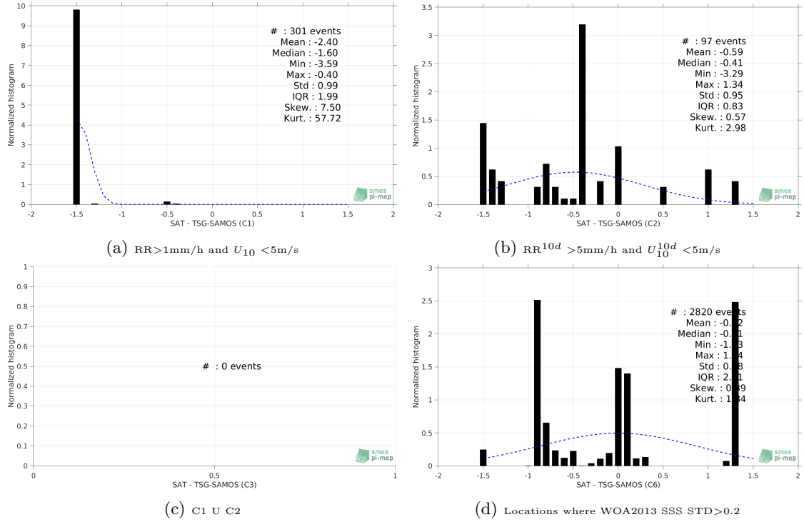
Figure 13: Normalized histogram of \Delta SSS (SMOS-L2-DPGS-v662 - TSG-SAMOS) for 6 different subdatasets corresponding to: RR > 1\text{mm/h} and U_{10} < 5\text{m/s} (a), RR^{10d} > 5\text{mm/h} and U_{10}^{10d} < 5\text{m/s} (b), C1 U C2 (c), Locations where WOA2013 SSS STD > 0.2 (d).
