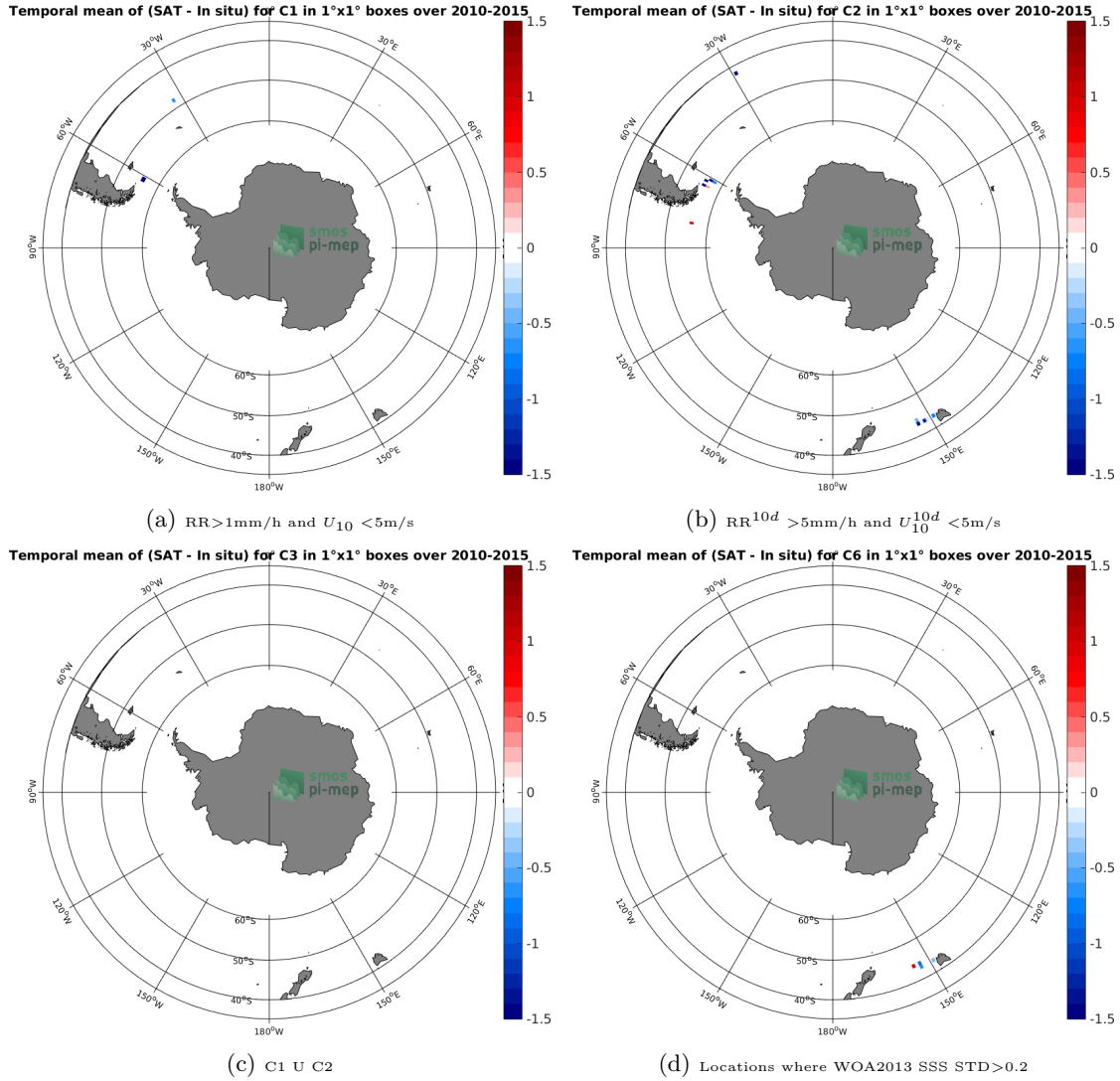
Figure 12: Temporal mean gridded over spatial boxes of size 1^\circ \times 1^\circ of \Delta SSS (SMOS-L2-DPGS-v662 - TSG-SAMOS) for 4 different subdatasets corresponding to: RR > 1\text{mm/h} and U_{10} < 5\text{m/s} (a), RR^{10d} > 5\text{mm/h} and U_{10}^{10d} < 5\text{m/s} (b), C1 U C2 (c), Locations where WOA2013 SSS STD > 0.2 (d).
