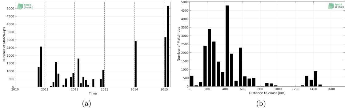
Figure 1: Number of match-ups between TSG-SAMOS and SMOS-L2-DPGS-v662 SSS as a function of time (a) and as function of the distance to coast (b) over the Roaring Forties and Furious Fifties Pi-MEP region and for the full satellite product period.
