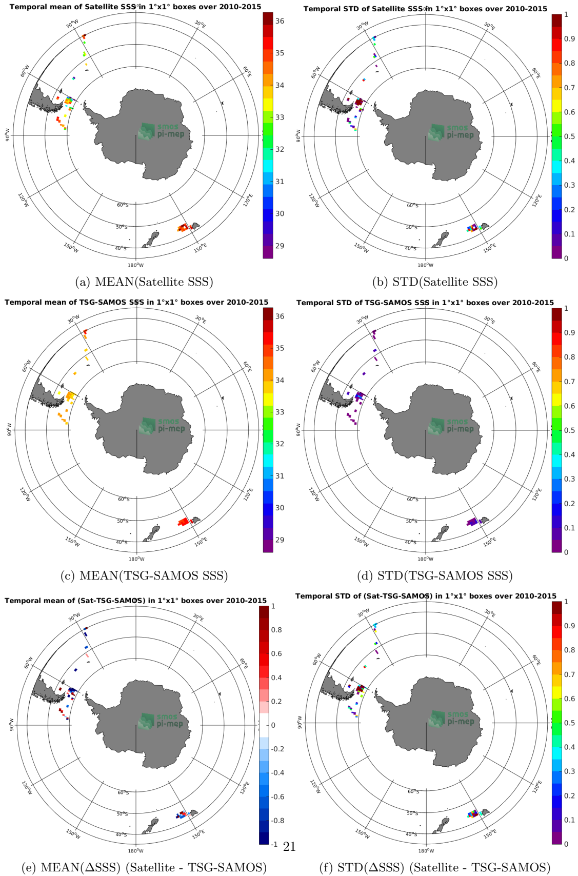
Figure 6: Temporal mean (left) and STD (right) of SSS from SMOS-L2-DPGS-v662 (top), TSG-SAMOS (middle), and of \Delta SSS (Satellite - TSG-SAMOS). Only match-up pairs are used to generate these maps.
