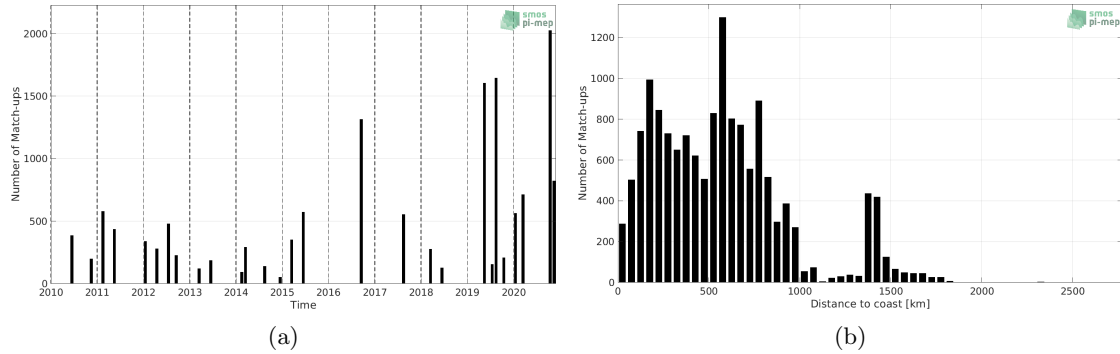
Figure 1: Number of match-ups between TSG (LEGOS-DM) and SMOS SSS L2 v662 (ESA) SSS as a function of time (a) and as function of the distance to coast (b) over the Roaring Forties and Furious Fifties Pi-MEP region and for the full satellite product period.
