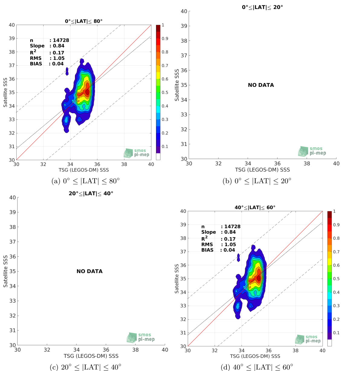
Figure 9: Contour maps of the concentration of SMOS SSS L2 v662 (ESA) SSS (y-axis) versus TSG (LEGOS-DM) SSS (x-axis) at match-up pairs for different latitude bands. For each plot, the red line shows x=y . The black thin and dashed lines indicate a linear fit through the data cloud and the \pm 95\% confidence levels, respectively. The number match-up pairs n , the slope and R^2 coefficient of the linear fit, the root mean square (RMS) and the mean bias between satellite and in situ data are indicated for each latitude band in each plots.
