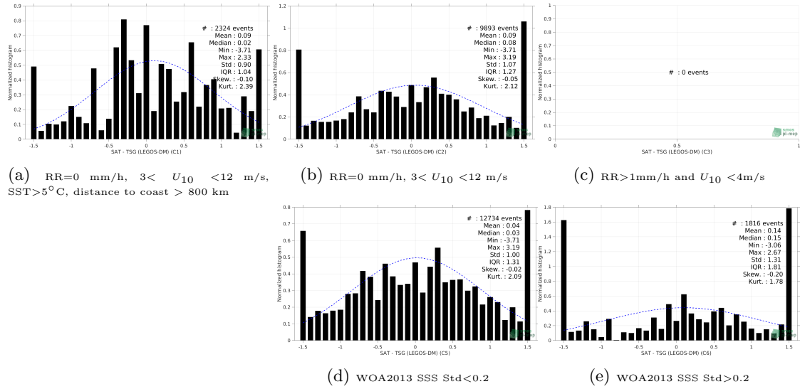
Figure 13: Normalized histogram of \Delta SSS (SMOS SSS L2 v662 (ESA) - TSG (LEGOS-DM)) for 5 different subdatasets corresponding to: RR=0 mm/h, 3 < U_{10} < 12 m/s, SST > 5°C, distance to coast > 800 km (a), RR=0 mm/h, 3 < U_{10} < 12 m/s (b), RR > 1mm/h and U_{10} < 4 m/s (c), WOA2013 SSS Std < 0.2 (d), WOA2013 SSS Std > 0.2 (e).
