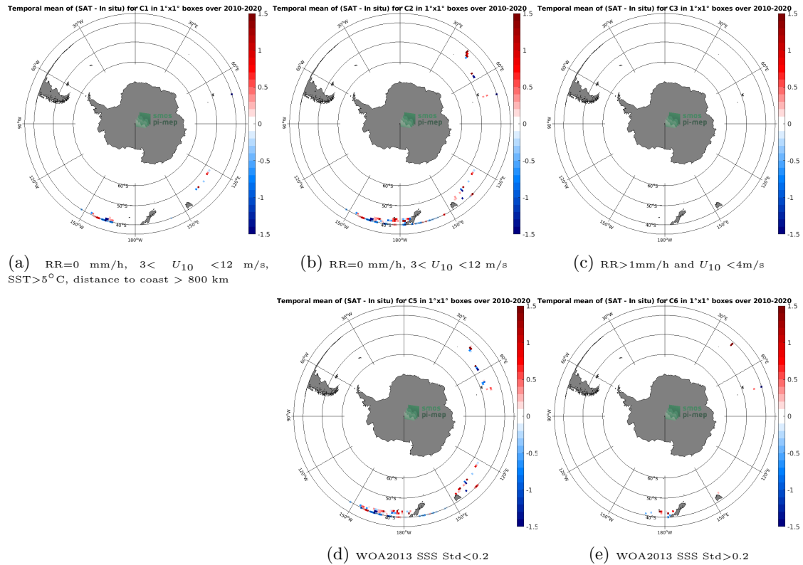
Figure 12: Temporal mean gridded over spatial boxes of size 1^{\circ}\times 1^{\circ} of \Delta\text{SSS} (SMOS SSS L2 v662 (ESA) - TSG (LEGOS-DM)) for 5 different subdatasets corresponding to:RR=0 mm/h, 3 < U_{10} < 12 m/s, SST >5^{\circ}\text{C} , distance to coast > 800 km (a), RR=0 mm/h, 3 < U_{10} < 12 m/s (b), RR >1 mm/h and U_{10} < 4 m/s (c), WOA2013 SSS Std <0.2 (d), WOA2013 SSS Std >0.2 (e).
