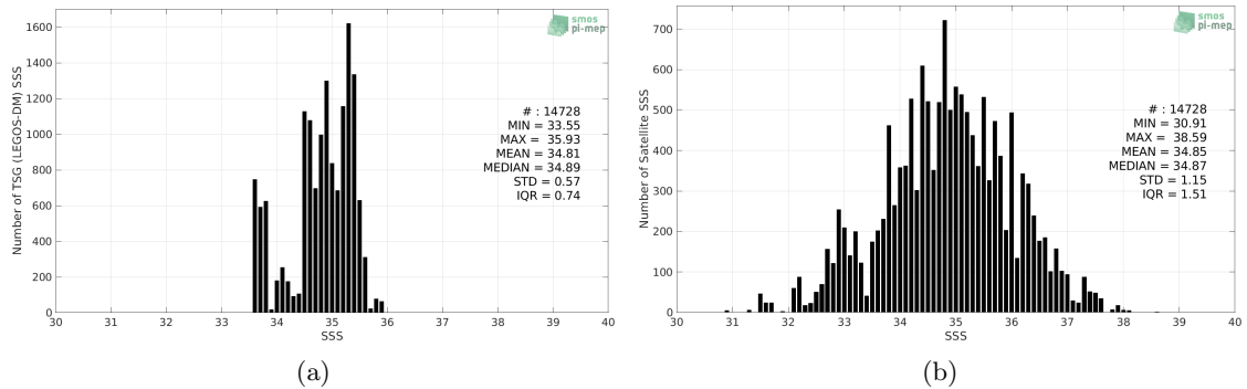
Figure 2: Histograms of SSS from TSG (LEGOS-DM) (a) and SMOS SSS L2 v662 (ESA) (b) considering all match-up pairs per bins of 0.1 over the Roaring Forties and Furious Fifties Pi-MEP region and for the full satellite product period.
