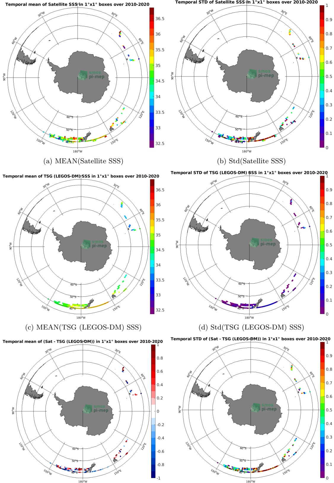
Figure 6: Temporal mean (left) and Std (right) of SSS from SMOS SSS L2 v662 (ESA) (top), TSG (LEGOS-DM) (middle), and of \Delta SSS (Satellite - TSG (LEGOS-DM)). Only match-up pairs are used to generate these maps.
