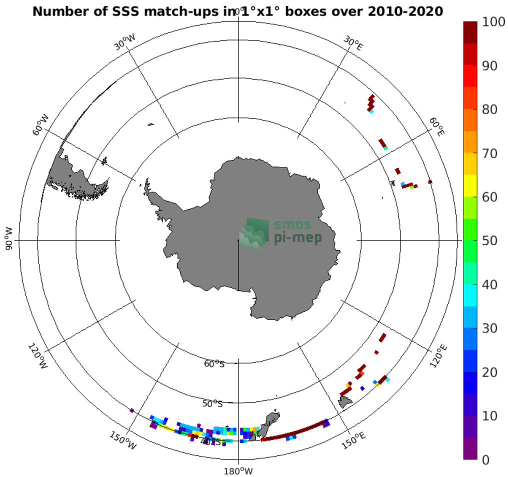
Figure 4: Number of SSS match-ups between TSG (LEGOS-DM) SSS and the SMOS SSS L2 v662 (ESA) SSS product for the Roaring Forties and Furious Fifties Pi-MEP region over 1^\circ \times 1^\circ boxes and for the full satellite product period.
