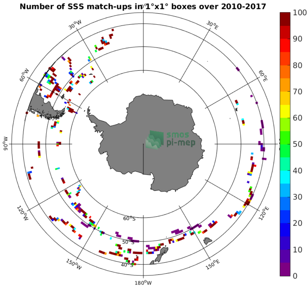
Figure 4: Number of SSS match-ups between TSG (GOSUD-Sailing-ship) SSS and the SMOS SSS L2 v662 (ESA) SSS product for the Roaring Forties and Furious Fifties Pi-MEP region over 1^\circ \times 1^\circ boxes and for the full satellite product period.
