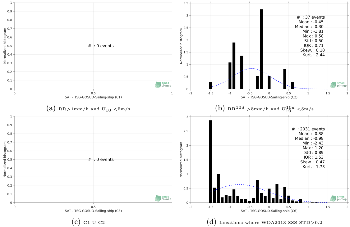
Figure 13: Normalized histogram of \Delta\text{SSS} (SMOS-L2-DPGS-v662 - TSG-GOSUD-Sailing-ship) for 6 different subdatasets corresponding to: RR > 1\text{mm/h} and U_{10} < 5\text{m/s} (a), RR^{10d} > 5\text{mm/h} and U_{10}^{10d} < 5\text{m/s} (b), C1 \cup C2 (c), Locations where WOA2013 SSS STD > 0.2 (d).
