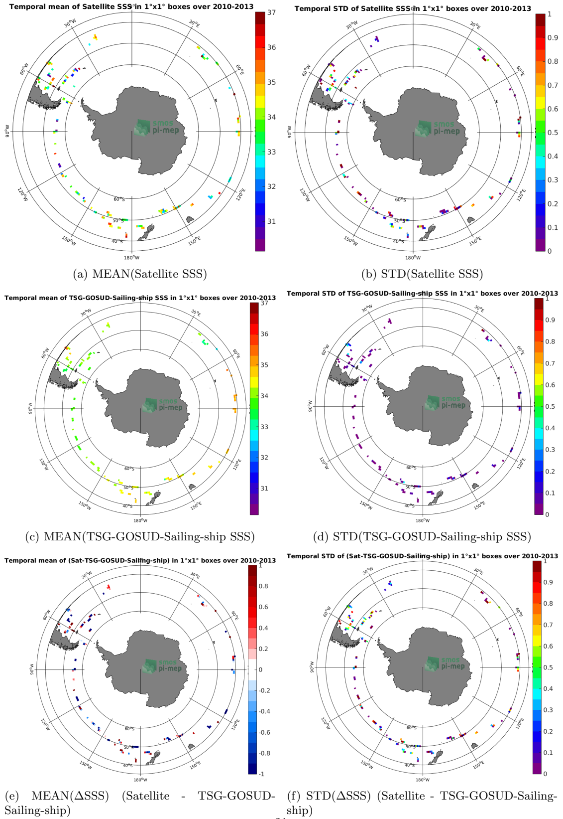
Figure 6: Temporal mean (left) and STD (right) of SSS from SMOS-L2-DPGS-v662 (top), TSG-GOSUD-Sailing-ship (middle), and of \Delta SSS (Satellite - TSG-GOSUD-Sailing-ship). Only match-up pairs are used to generate these maps.
