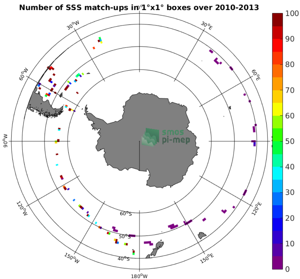
Figure 4: Number of SSS match-ups between TSG-GOSUD-Sailing-ship SSS and the SMOS-L2-DPGS-v662 SSS product for the Roaring Forties and Furious Fifties Pi-MEP region over 1°x1° boxes and for the full satellite product period.
