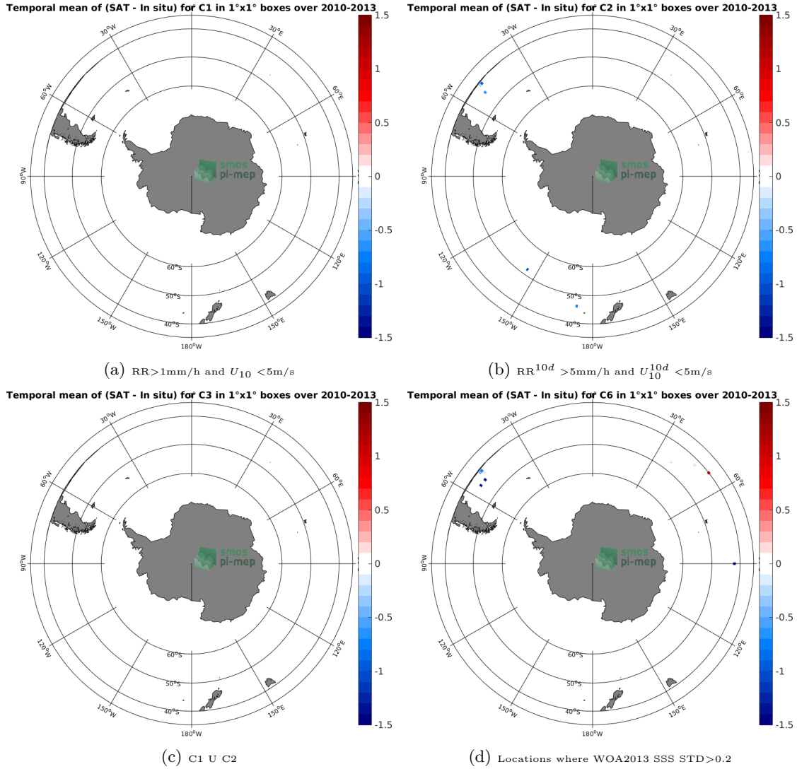
Figure 12: Temporal mean gridded over spatial boxes of size 1^\circ \times 1^\circ of \Delta SSS (SMOS-L2-DPGS-v662 - TSG-GOSUD-Sailing-ship) for 4 different subdatasets corresponding to: RR > 1\text{mm/h} and U_{10} < 5\text{m/s} (a), RR^{10d} > 5\text{mm/h} and U_{10}^{10d} < 5\text{m/s} (b), C1 U C2 (c), Locations where WOA2013 SSS STD > 0.2 (d).
