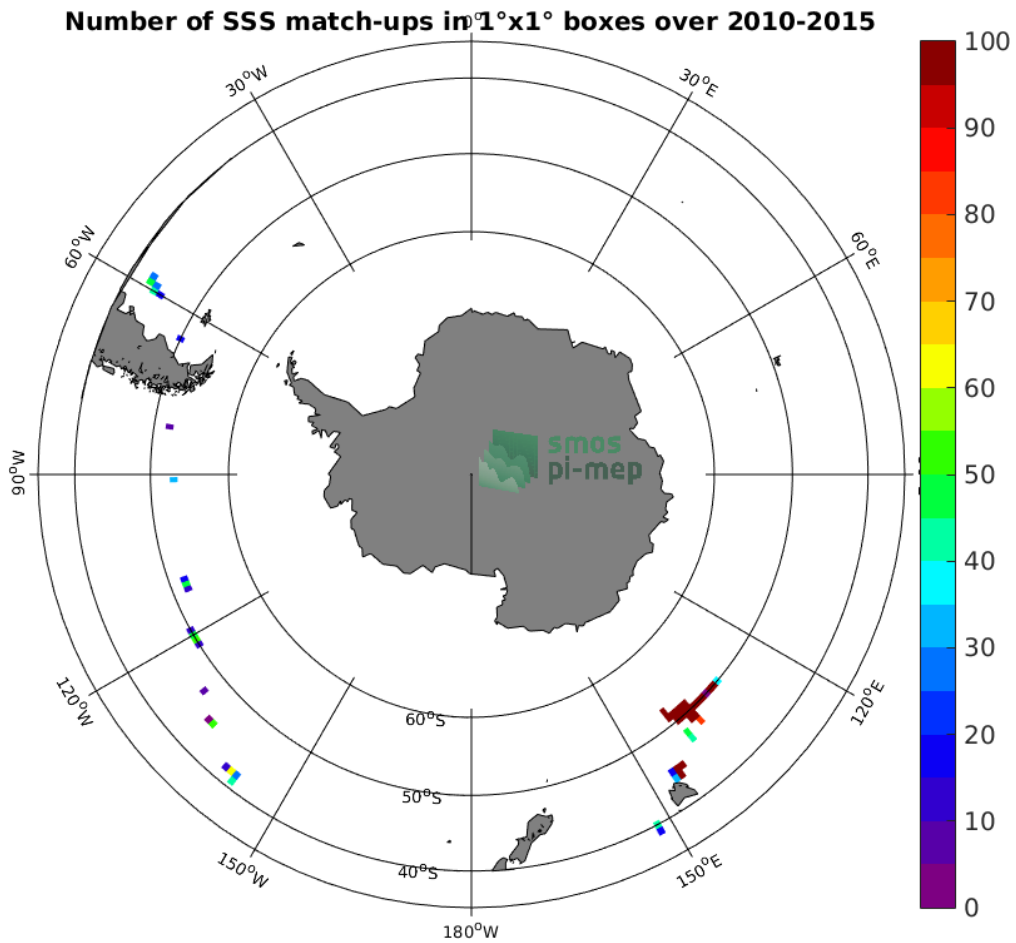
Figure 4: Number of SSS match-ups between TSG-GOSUD-Research-vessel SSS and the SMOS-L2-DPGS-v662 SSS product for the Roaring Forties and Furious Fifties Pi-MEP region over 1°x1° boxes and for the full satellite product period.
