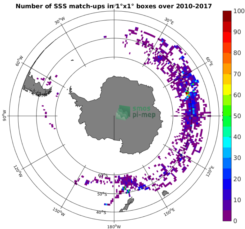
Figure 4: Number of SSS match-ups between Sea mammals SSS and the SMOS-L2-DPGS-v662 SSS product for the Roaring Forties and Furious Fifties Pi-MEP region over 1°x1° boxes and for the full satellite product period.
