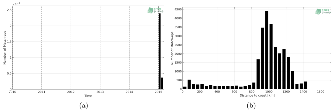
Figure 1: Number of match-ups between TSG (GOSUD-Research-vessel) and SMAP SSS L4 OI v1 - 7 Days (IPRC) SSS as a function of time (a) and as function of the distance to coast (b) over the Roaring Forties and Furious Fifties Pi-MEP region and for the full satellite product period.
