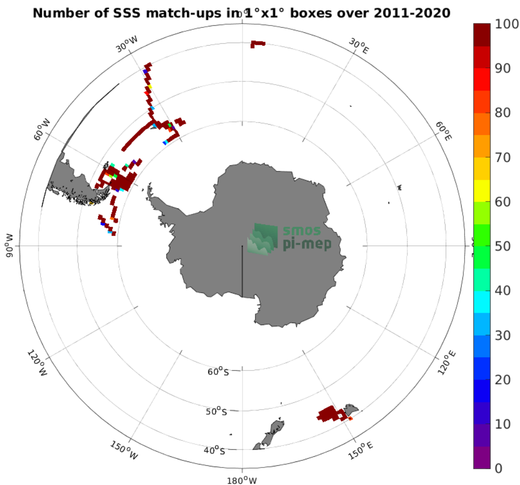
Figure 4: Number of SSS match-ups between TSG (SAMOS) SSS and the SMAP SSS L4 OI v1 - Monthly (IPRC) SSS product for the Roaring Forties and Furious Fifties Pi-MEP region over 1^\circ \times 1^\circ boxes and for the full satellite product period.
