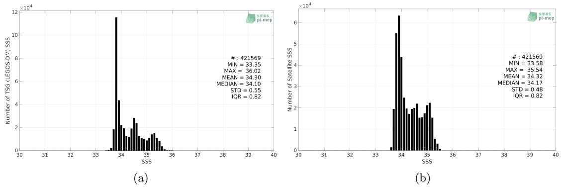
Figure 2: Histograms of SSS from TSG (LEGOS-DM) (a) and SMAP SSS L4 OI v1 - Monthly (IPRC) (b) considering all match-up pairs per bins of 0.1 over the Roaring Forties and Furious Fifties Pi-MEP region and for the full satellite product period.
