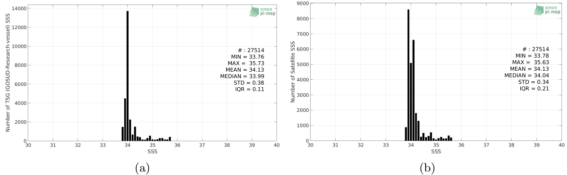
Figure 2: Histograms of SSS from TSG (GOSUD-Research-vessel) (a) and SMAP SSS L4 OI v1 - Monthly (IPRC) (b) considering all match-up pairs per bins of 0.1 over the Roaring Forties and Furious Fifties Pi-MEP region and for the full satellite product period.
