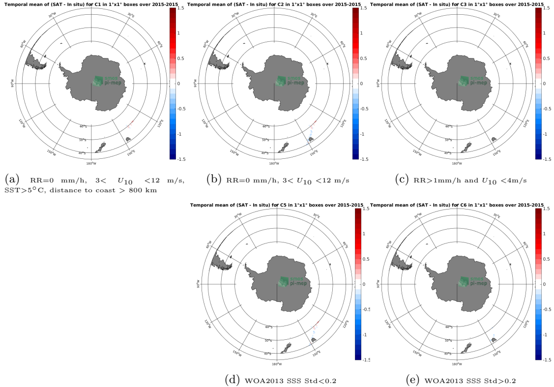
Figure 12: Temporal mean gridded over spatial boxes of size 1^\circ \times 1^\circ of \Delta SSS (SMAP SSS L4 OI v1 - Monthly (IPRC) - TSG (GOSUD-Research-vessel)) for 5 different subdatasets corresponding to: RR=0 mm/h, 3 < U_{10} < 12 m/s, SST > 5°C, distance to coast > 800 km (a), RR=0 mm/h, 3 < U_{10} < 12 m/s (b), RR > 1mm/h and U_{10} < 4 m/s (c), WOA2013 SSS Std < 0.2 (d), WOA2013 SSS Std > 0.2 (e).
