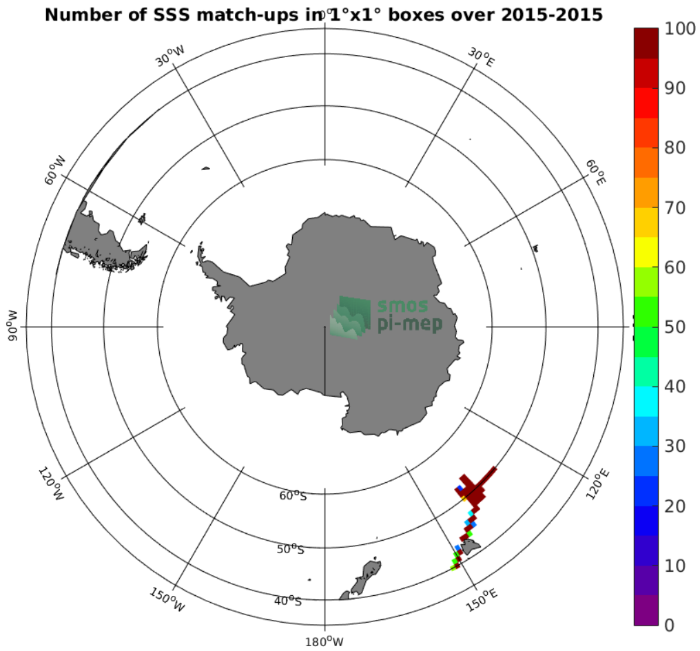
Figure 4: Number of SSS match-ups between TSG (GOSUD-Research-vessel) SSS and the SMAP SSS L4 OI v1 - Monthly (IPRC) SSS product for the Roaring Forties and Furious Fifties Pi-MEP region over 1^\circ \times 1^\circ boxes and for the full satellite product period.
