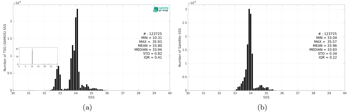
Figure 3: Histograms of SSS from TSG (SAMOS) (a) and SMAP SSS L4 OI v3 - Monthly (ESR) (b) considering all match-up pairs per bins of 0.1 over the Roaring Forties and Furious Fifties Pi-MEP region and for the full satellite product period.
