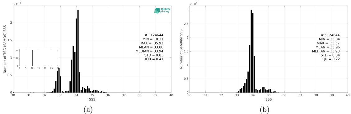
Figure 3: Histograms of SSS from TSG (SAMOS) (a) and SMAP SSS L4 OI v3 - Monthly (ESR) (b) considering all match-up pairs per bins of 0.1 over the Roaring Forties and Furious Fifties Pi-MEP region and for the full satellite product period.
