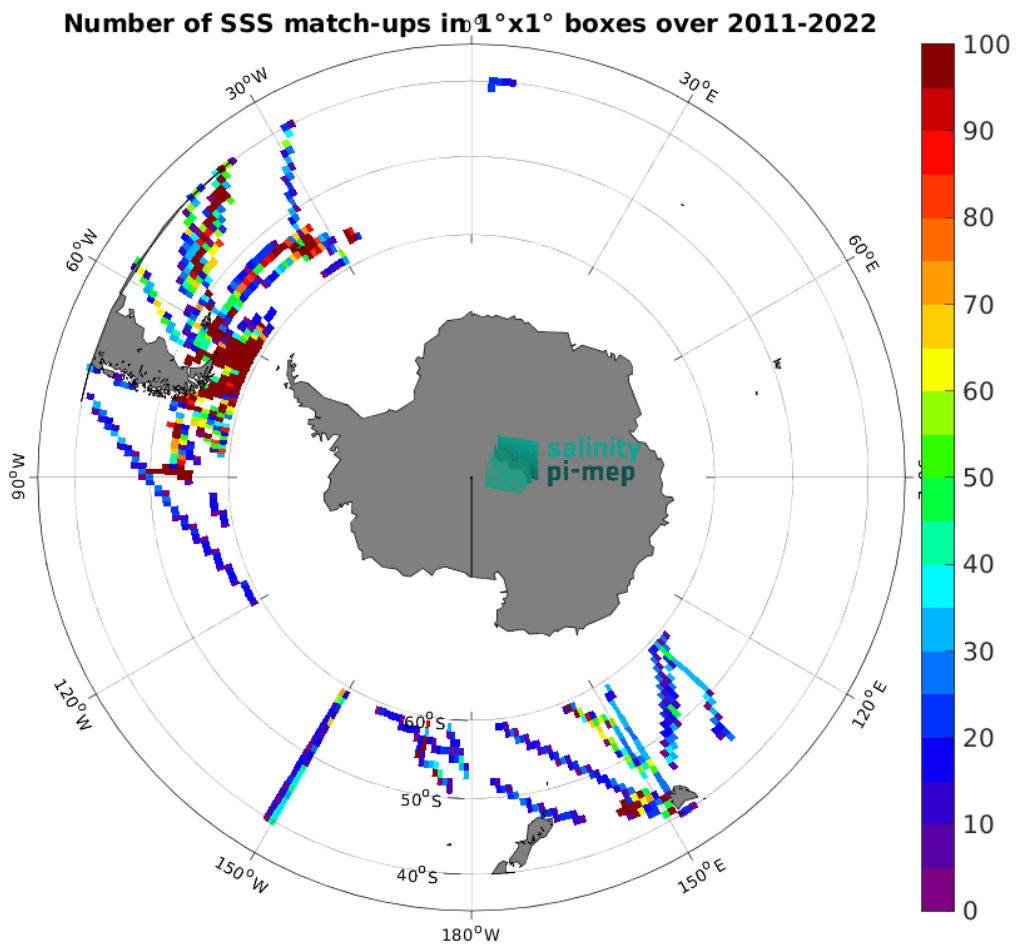
Figure 5: Number of SSS match-ups between TSG (SAMOS) SSS and the SMAP SSS L4 OI v3 - Monthly (ESR) SSS product for the Roaring Forties and Furious Fifties Pi-MEP region over 1^\circ \times 1^\circ boxes and for the full satellite product period.
