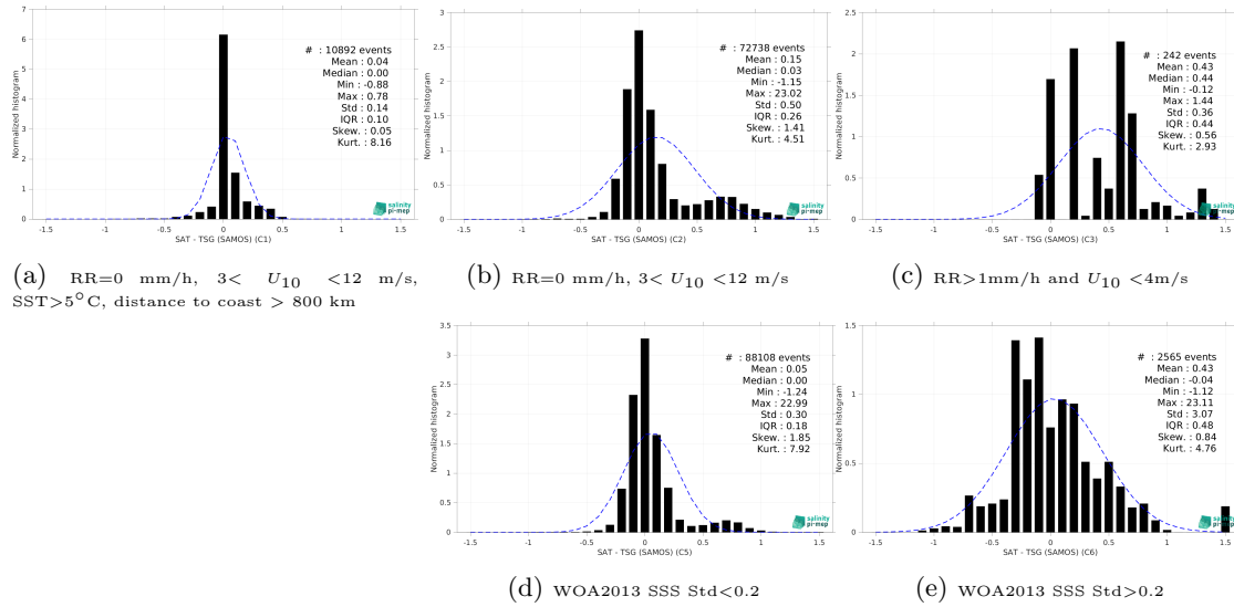
Figure 15: Normalized histogram of \Delta\text{SSS} (SMAP SSS L4 OI v3 - Monthly (ESR) - TSG (SAMOS)) for 5 different subdatasets corresponding to: RR=0 mm/h, 3 < U_{10} < 12 m/s, SST > 5^{\circ}\text{C} , distance to coast > 800 km (a), RR=0 mm/h, 3 < U_{10} < 12 m/s (b), RR > 1 mm/h and U_{10} < 4 m/s (c), WOA2013 SSS Std < 0.2 (d), WOA2013 SSS Std > 0.2 (e).
