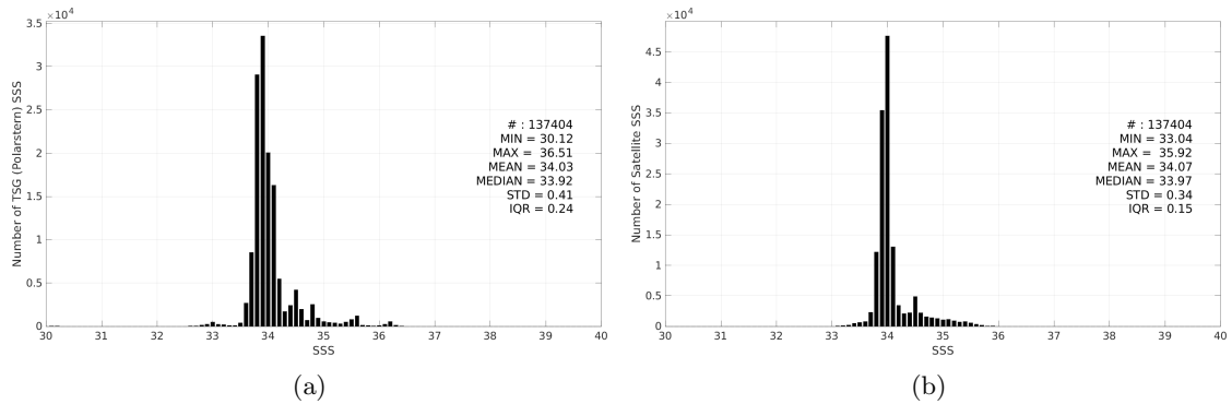
Figure 3: Histograms of SSS from TSG (Polarstern) (a) and SMAP SSS L4 OI v3 - Monthly (ESR) (b) considering all match-up pairs per bins of 0.1 over the Roaring Forties and Furious Fifties Pi-MEP region and for the full satellite product period.
