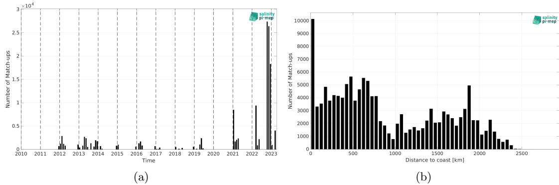
Figure 2: Number of match-ups between TSG (Polarstern) and SMAP SSS L4 OI v3 - Monthly (ESR) SSS as a function of time (a) and as function of the distance to coast (b) over the Roaring Forties and Furious Fifties Pi-MEP region and for the full satellite product period.
