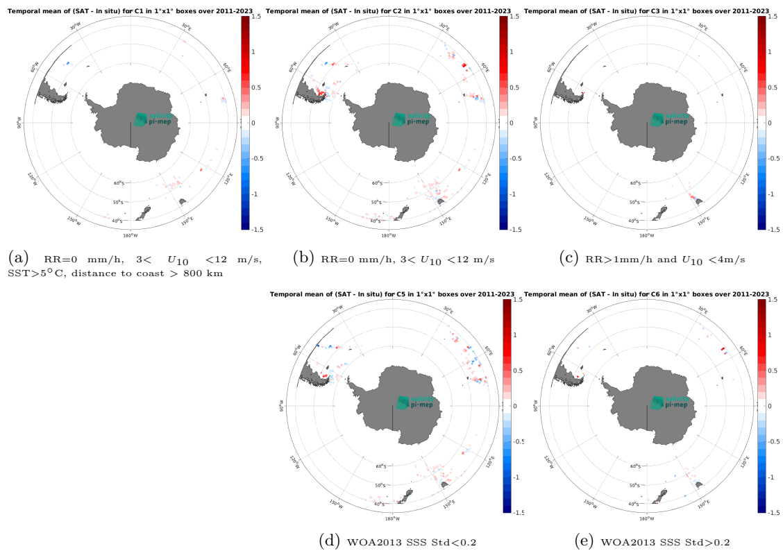
Figure 14: Temporal mean gridded over spatial boxes of size 1^\circ \times 1^\circ of \Delta\text{SSS} (SMAP SSS L4 OI v3 - Monthly (ESR) - TSG (LEGOS-DM)) for 5 different subdatasets corresponding to:RR=0 mm/h, 3 < U_{10} < 12 m/s, SST >5^\circ\text{C} , distance to coast > 800 km (a), RR=0 mm/h, 3 < U_{10} < 12 m/s (b), RR >1 mm/h and U_{10} < 4 m/s (c), WOA2013 SSS Std <0.2 (d), WOA2013 SSS Std >0.2 (e).
