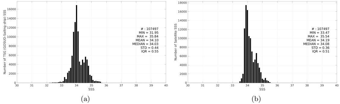
Figure 3: Histograms of SSS from TSG (GOSUD-Sailing-ship) (a) and SMAP SSS L4 OI v3 - Monthly (ESR) (b) considering all match-up pairs per bins of 0.1 over the Roaring Forties and Furious Fifties Pi-MEP region and for the full satellite product period.
