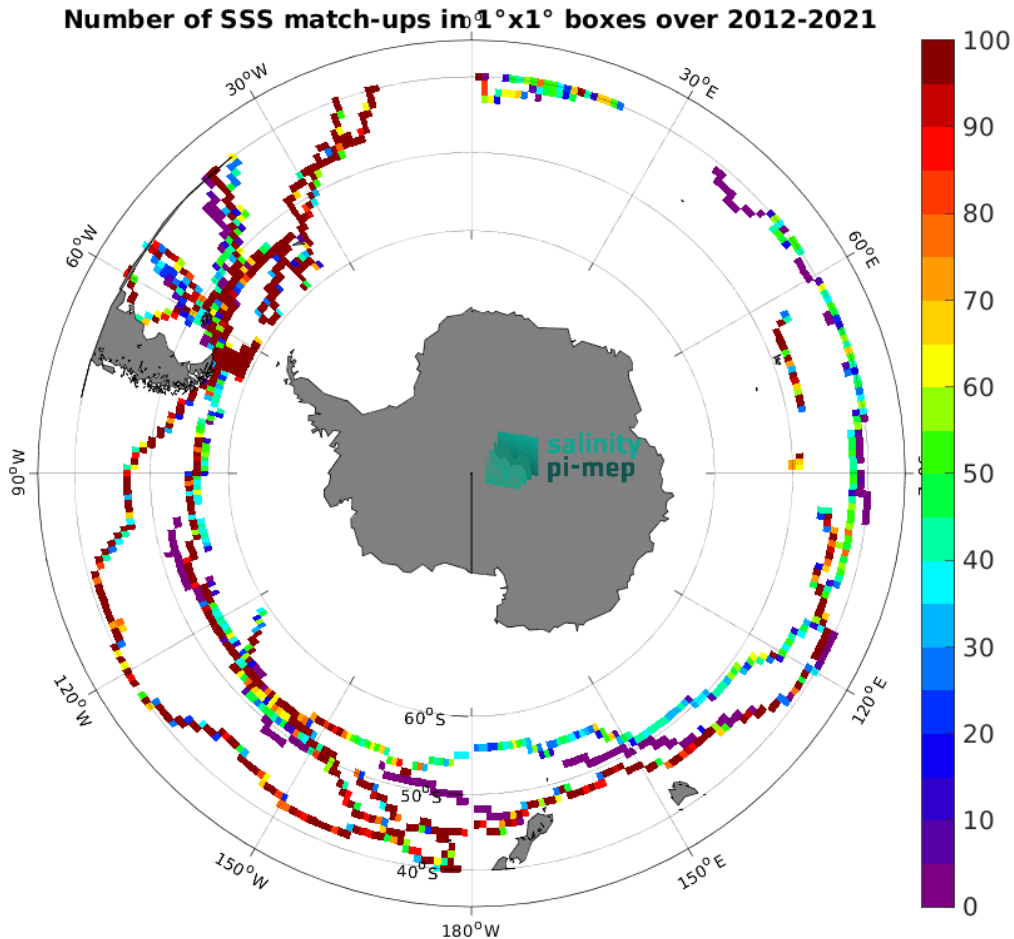
Figure 5: Number of SSS match-ups between TSG (GOSUD-Sailing-ship) SSS and the SMAP SSS L4 OI v3 - Monthly (ESR) SSS product for the Roaring Forties and Furious Fifties Pi-MEP region over 1^\circ \times 1^\circ boxes and for the full satellite product period.
