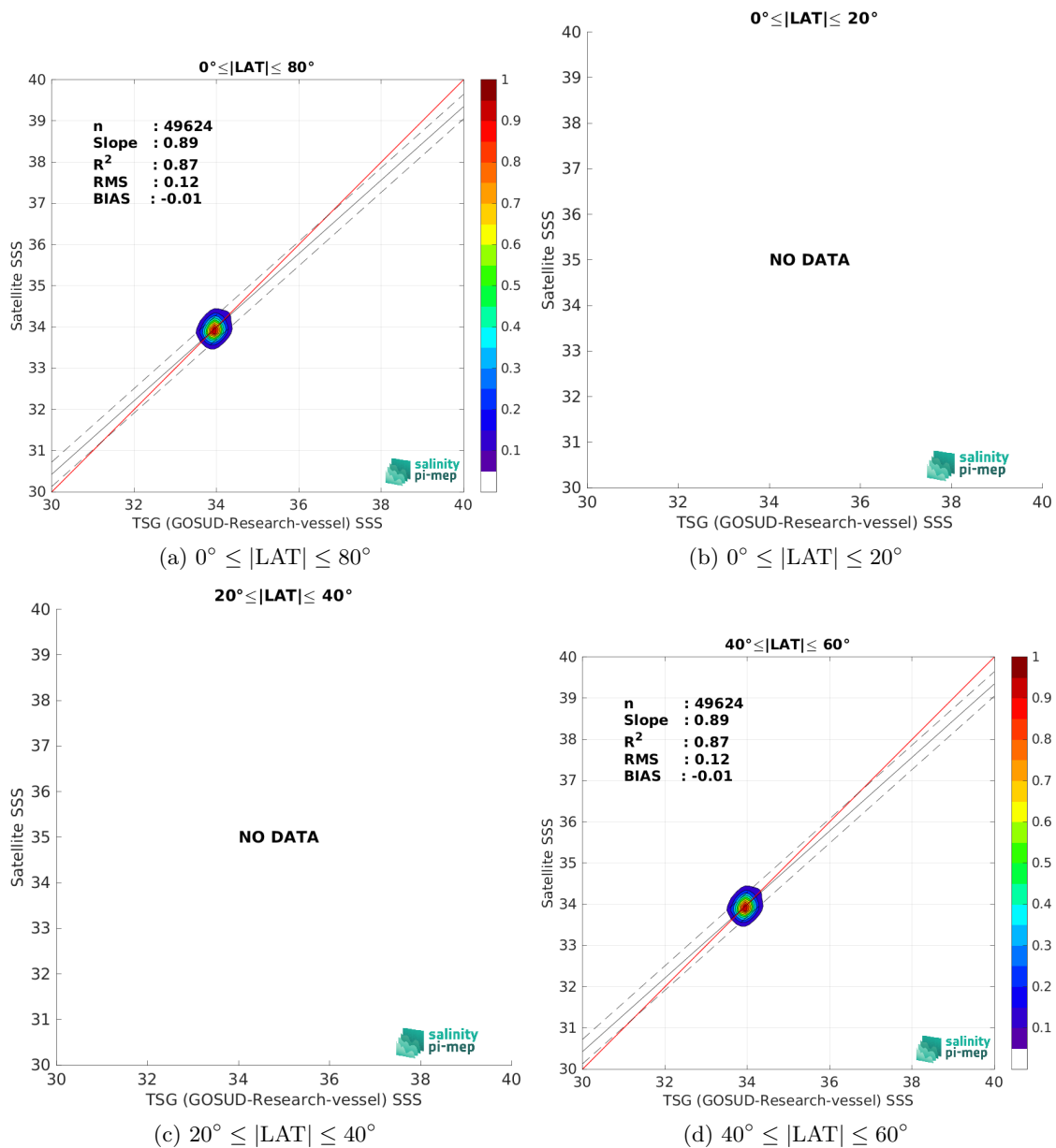
Figure 10: Contour maps of the concentration of SMAP SSS L4 OI v3 - Monthly (ESR) SSS (y-axis) versus TSG (GOSUD-Research-vessel) SSS (x-axis) at match-up pairs for different latitude bands. For each plot, the red line shows x=y . The black thin and dashed lines indicate a linear fit through the data cloud and the \pm 95\% confidence levels, respectively. The number match-up pairs n , the slope and R^2 coefficient of the linear fit, the root mean square (RMS) and the mean bias between satellite and in situ data are indicated for each latitude band in each plots.
