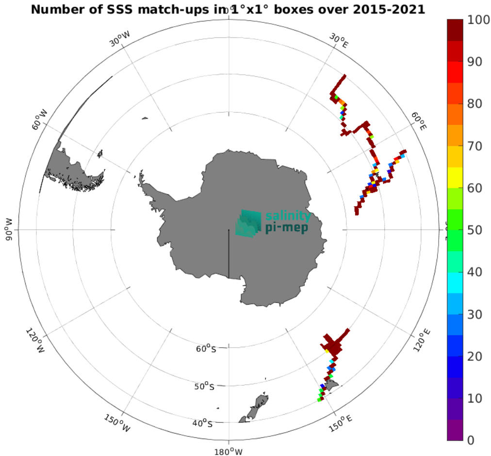
Figure 5: Number of SSS match-ups between TSG (GOSUD-Research-vessel) SSS and the SMAP SSS L4 OI v3 - Monthly (ESR) SSS product for the Roaring Forties and Furious Fifties Pi-MEP region over 1^\circ \times 1^\circ boxes and for the full satellite product period.
