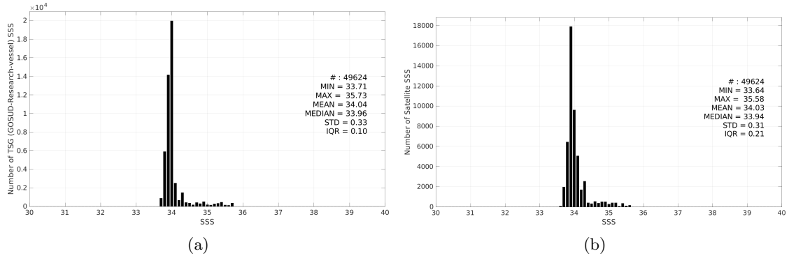
Figure 3: Histograms of SSS from TSG (GOSUD-Research-vessel) (a) and SMAP SSS L4 OI v3 - Monthly (ESR) (b) considering all match-up pairs per bins of 0.1 over the Roaring Forties and Furious Fifties Pi-MEP region and for the full satellite product period.
