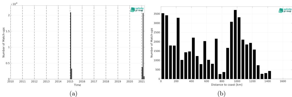
Figure 2: Number of match-ups between TSG (GOSUD-Research-vessel) and SMAP SSS L4 OI v3 - Monthly (ESR) SSS as a function of time (a) and as function of the distance to coast (b) over the Roaring Forties and Furious Fifties Pi-MEP region and for the full satellite product period.
