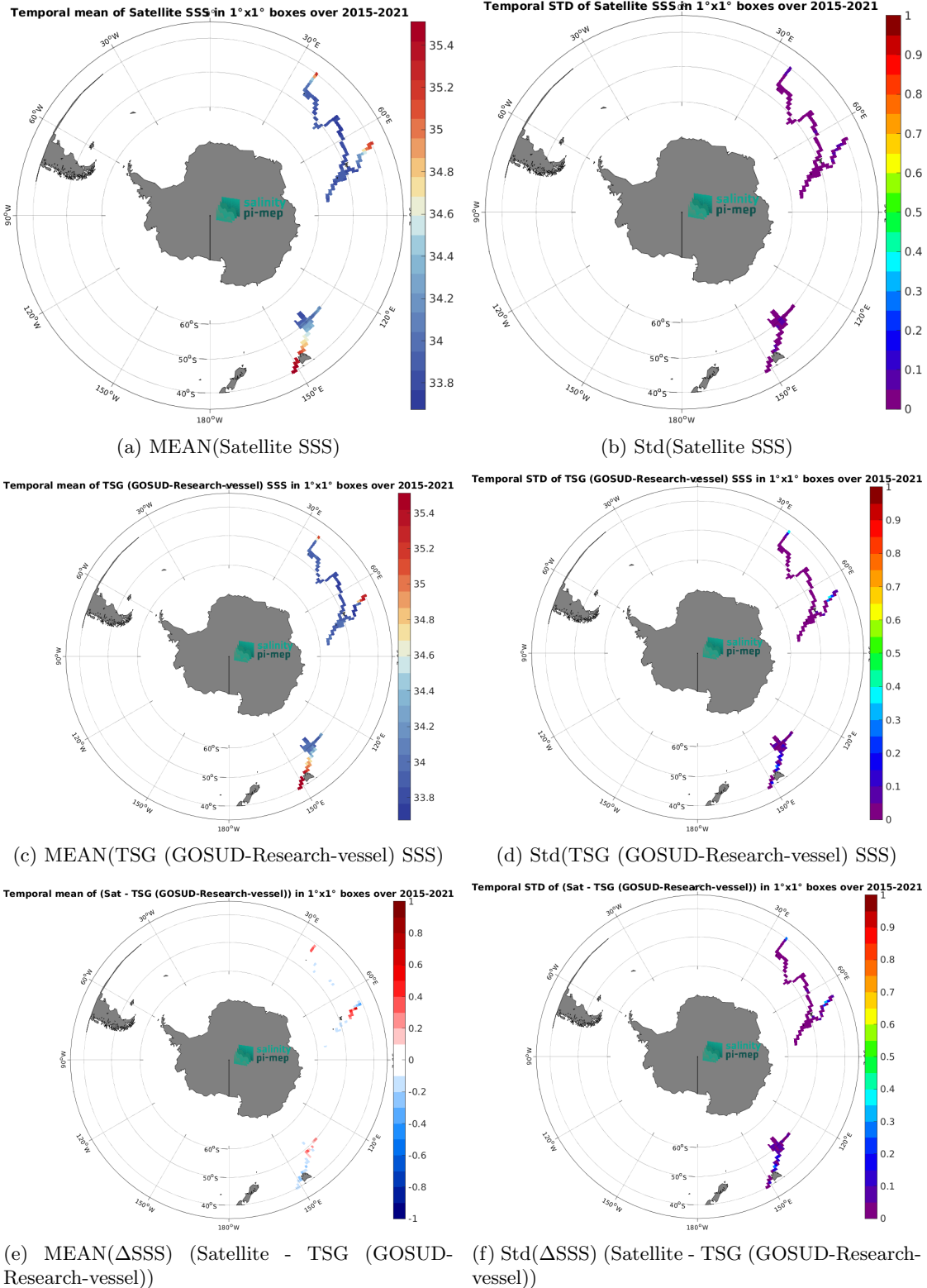
Figure 7: Temporal mean (left) and Std (right) of SSS from SMAP SSS L4 OI v3 - Monthly (ESR) (top), TSG (GOSUD-Research-vessel) (middle), and of \Delta SSS (Satellite - TSG (GOSUD-Research-vessel)). Only match-up pairs are used to generate these maps.
