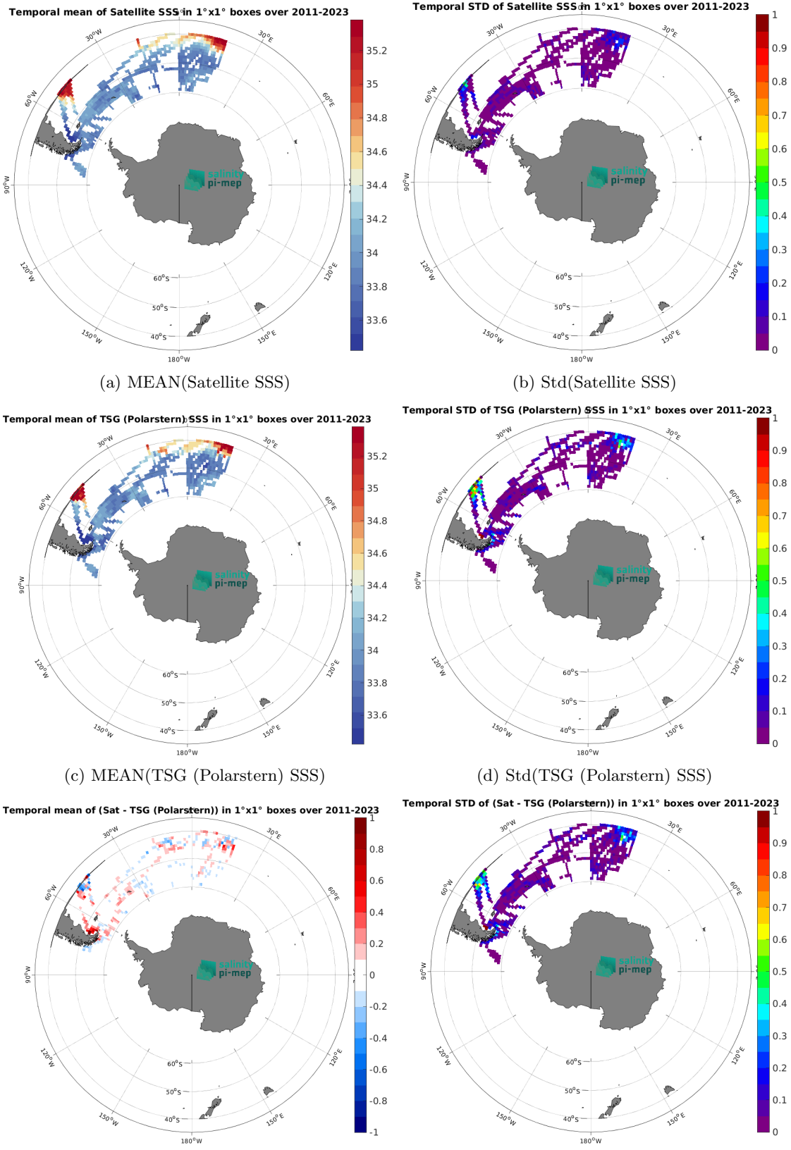
Figure 7: Temporal mean (left) and Std (right) of SSS from SMAP SSS L4 OI v3 - Daily (ESR) (top), TSG (Polarstern) (middle), and of \Delta SSS (Satellite - TSG (Polarstern)). Only match-up pairs are used to generate these maps.
