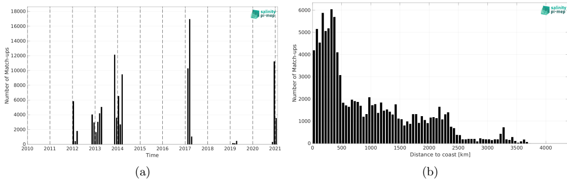
Figure 2: Number of match-ups between TSG (GOSUD-Sailing-ship) and SMAP SSS L4 OI v3 - Daily (ESR) SSS as a function of time (a) and as function of the distance to coast (b) over the Roaring Forties and Furious Fifties Pi-MEP region and for the full satellite product period.
