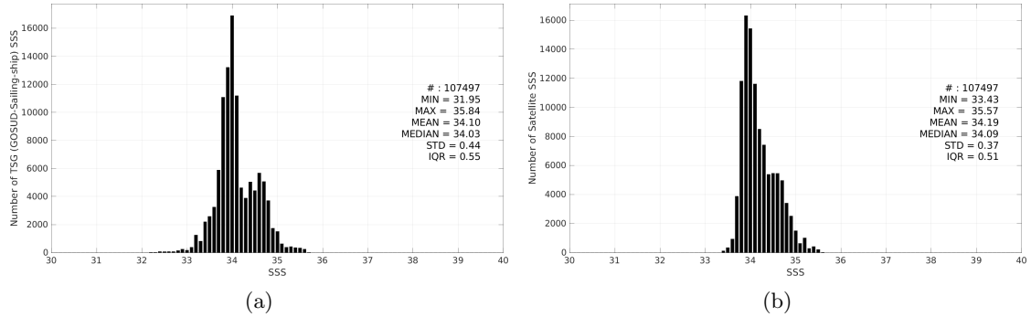
Figure 3: Histograms of SSS from TSG (GOSUD-Sailing-ship) (a) and SMAP SSS L4 OI v3 - Daily (ESR) (b) considering all match-up pairs per bins of 0.1 over the Roaring Forties and Furious Fifties Pi-MEP region and for the full satellite product period.
