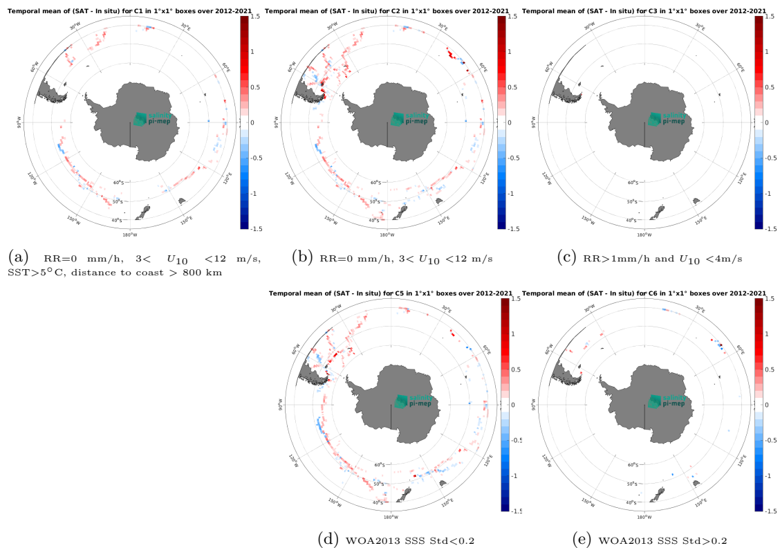
Figure 14: Temporal mean gridded over spatial boxes of size 1^\circ \times 1^\circ of \Delta\text{SSS} (SMAP SSS L4 OI v3 - Daily (ESR) - TSG (GOSUD-Sailing-ship)) for 5 different subdatasets corresponding to: RR=0 mm/h, 3 < U_{10} < 12 m/s, SST > 5°C, distance to coast > 800 km (a), RR=0 mm/h, 3 < U_{10} < 12 m/s (b), RR > 1mm/h and U_{10} < 4 m/s (c), WOA2013 SSS Std < 0.2 (d), WOA2013 SSS Std > 0.2 (e).
