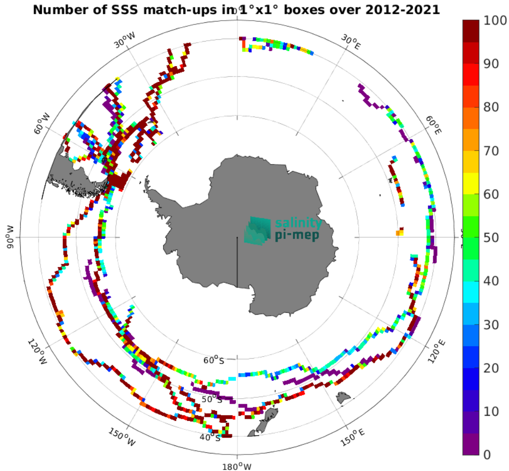
Figure 5: Number of SSS match-ups between TSG (GOSUD-Sailing-ship) SSS and the SMAP SSS L4 OI v3 - Daily (ESR) SSS product for the Roaring Forties and Furious Fifties Pi-MEP region over 1^\circ \times 1^\circ boxes and for the full satellite product period.
