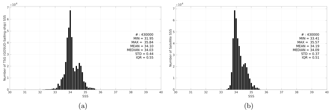
Figure 3: Histograms of SSS from TSG (GOSUD-Sailing-ship) (a) and SMAP SSS L4 OI v3 - Daily (ESR) (b) considering all match-up pairs per bins of 0.1 over the Roaring Forties and Furious Fifties Pi-MEP region and for the full satellite product period.
