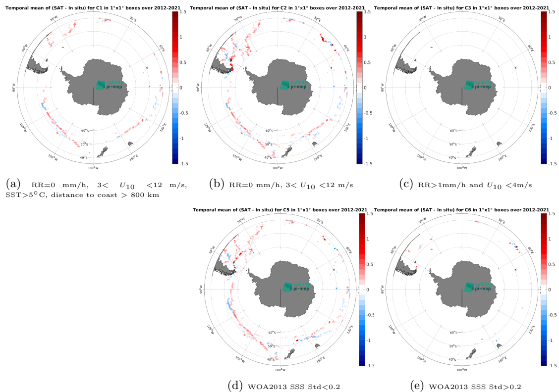
Figure 14: Temporal mean gridded over spatial boxes of size 1^\circ \times 1^\circ of \Delta SSS (SMAP SSS L4 OI v3 - Daily (ESR) - TSG (GOSUD-Sailing-ship)) for 5 different subdatasets corresponding to:RR=0 mm/h, 3 < U_{10} < 12 m/s, SST > 5^\circ\text{C} , distance to coast > 800 km (a), RR=0 mm/h, 3 < U_{10} < 12 m/s (b), RR > 1 mm/h and U_{10} < 4 m/s (c), WOA2013 SSS Std < 0.2 (d), WOA2013 SSS Std > 0.2 (e).
