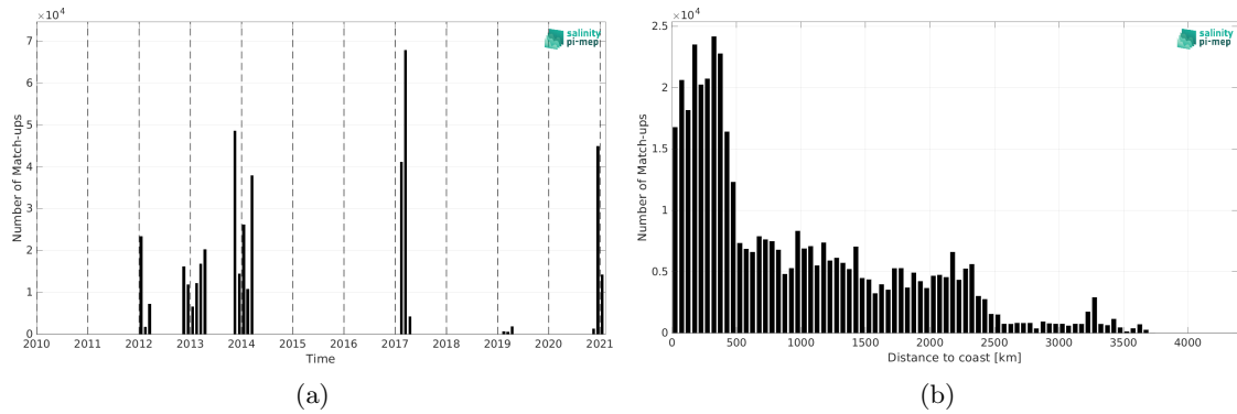
Figure 2: Number of match-ups between TSG (GOSUD-Sailing-ship) and SMAP SSS L4 OI v3 - Daily (ESR) SSS as a function of time (a) and as function of the distance to coast (b) over the Roaring Forties and Furious Fifties Pi-MEP region and for the full satellite product period.
