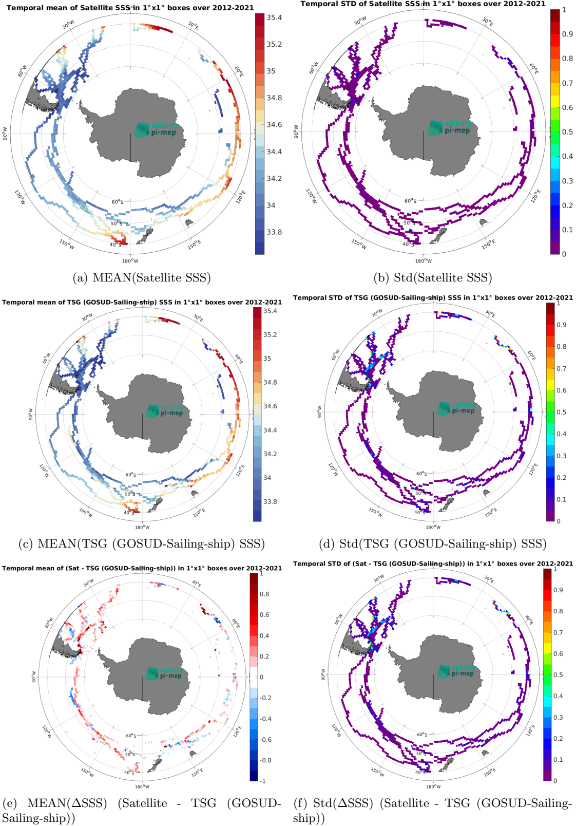
Figure 7: Temporal mean (left) and Std (right) of SSS from SMAP SSS L4 OI v3 - Daily (ESR) (top), TSG (GOSUD-Sailing-ship) (middle), and of \Delta SSS (Satellite - TSG (GOSUD-Sailing-ship)). Only match-up pairs are used to generate these maps.
