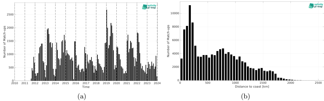
Figure 2: Number of match-ups between Marine mammals and SMAP SSS L4 OI v3 - Daily (ESR) SSS as a function of time (a) and as function of the distance to coast (b) over the Roaring Forties and Furious Fifties Pi-MEP region and for the full satellite product period.
