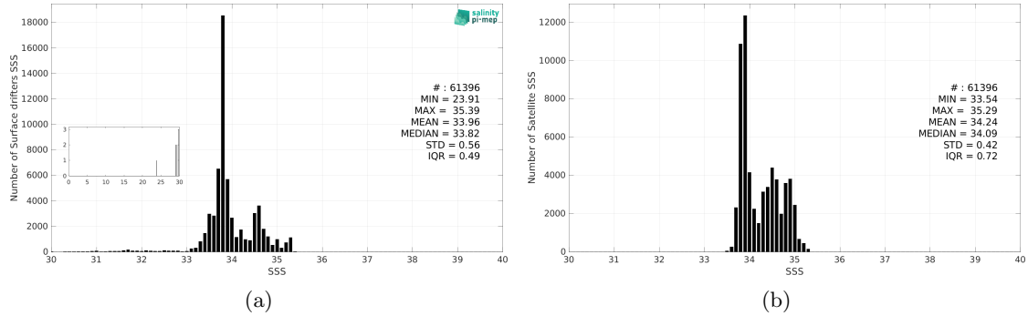
Figure 3: Histograms of SSS from Surface drifters (a) and SMAP SSS L4 OI v3 - Daily (ESR) (b) considering all match-up pairs per bins of 0.1 over the Roaring Forties and Furious Fifties Pi-MEP region and for the full satellite product period.
