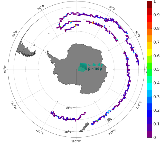
(e) MEAN( \Delta SSS) (Satellite - Surface drifters) 16
