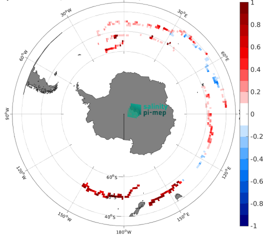
(e) MEAN( \Delta SSS) (Satellite - Surface drifters) 16
