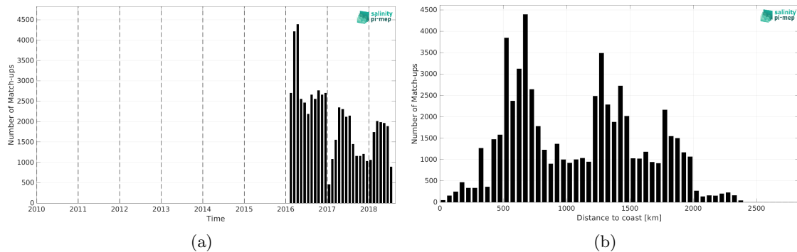
Figure 2: Number of match-ups between Surface drifters and SMAP SSS L4 OI v3 - Daily (ESR) SSS as a function of time (a) and as function of the distance to coast (b) over the Roaring Forties and Furious Fifties Pi-MEP region and for the full satellite product period.
