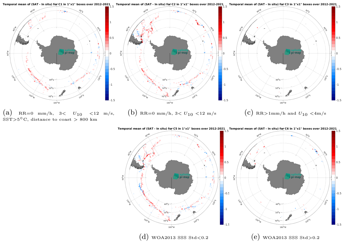
Figure 12: Temporal mean gridded over spatial boxes of size 1^\circ \times 1^\circ of \Delta SSS (SMAP SSS L4 OI v2 - 7 Days (ESR) - TSG (GOSUD-Sailing-ship)) for 5 different subdatasets corresponding to: RR=0 mm/h, 3 < U_{10} < 12 m/s, SST>5°C, distance to coast > 800 km (a), RR=0 mm/h, 3 < U_{10} < 12 m/s (b), RR>1mm/h and U_{10} < 4 m/s (c), WOA2013 SSS Std<0.2 (d), WOA2013 SSS Std>0.2 (e).
