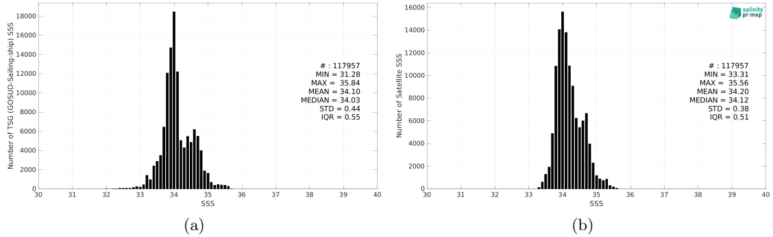
Figure 2: Histograms of SSS from TSG (GOSUD-Sailing-ship) (a) and SMAP SSS L4 OI v2 - 7 Days (ESR) (b) considering all match-up pairs per bins of 0.1 over the Roaring Forties and Furious Fifties Pi-MEP region and for the full satellite product period.
