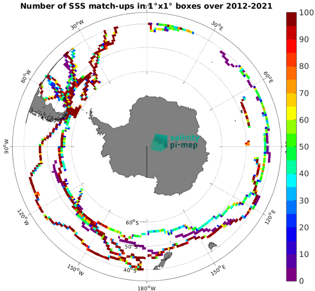
Figure 4: Number of SSS match-ups between TSG (GOSUD-Sailing-ship) SSS and the SMAP SSS L4 OI v2 - 7 Days (ESR) SSS product for the Roaring Forties and Furious Fifties Pi-MEP region over 1^\circ \times 1^\circ boxes and for the full satellite product period.
