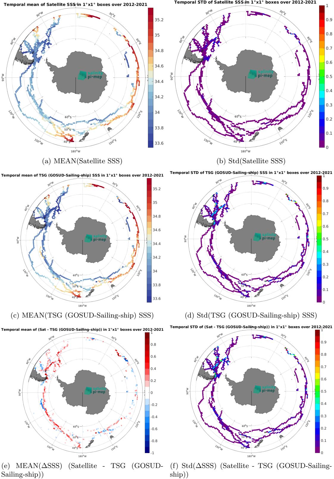
Figure 6: Temporal mean (left) and Std (right) of SSS from SMAP SSS L4 OI v2 - 7 Days (ESR) (top), TSG (GOSUD-Sailing-ship) (middle), and of \Delta SSS (Satellite - TSG (GOSUD-Sailing-ship)). Only match-up pairs are used to generate these maps.
