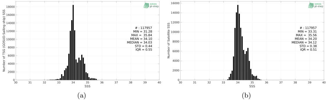
Figure 2: Histograms of SSS from TSG (GOSUD-Sailing-ship) (a) and SMAP SSS L4 OI v2 - 7 Days (ESR) (b) considering all match-up pairs per bins of 0.1 over the Roaring Forties and Furious Fifties Pi-MEP region and for the full satellite product period.
