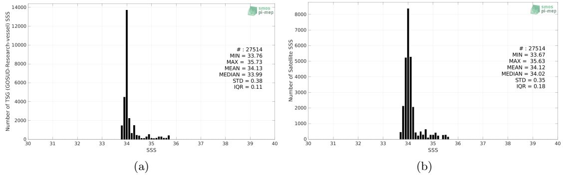
Figure 2: Histograms of SSS from TSG (GOSUD-Research-vessel) (a) and SMAP SSS L4 OI v2 - 7 Days (ESR) (b) considering all match-up pairs per bins of 0.1 over the Roaring Forties and Furious Fifties Pi-MEP region and for the full satellite product period.
