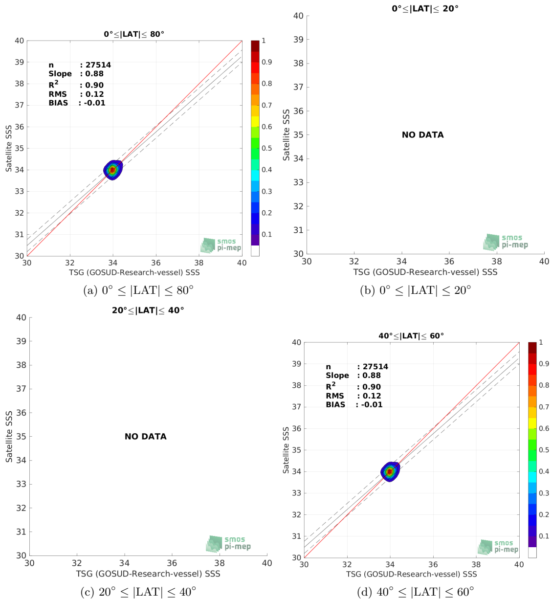
Figure 9: Contour maps of the concentration of SMAP SSS L4 OI v2 - 7 Days (ESR) SSS (y-axis) versus TSG (GOSUD-Research-vessel) SSS (x-axis) at match-up pairs for different latitude bands. For each plot, the red line shows x=y . The black thin and dashed lines indicate a linear fit through the data cloud and the \pm 95\% confidence levels, respectively. The number match-up pairs n , the slope and R^2 coefficient of the linear fit, the root mean square (RMS) and the mean bias between satellite and in situ data are indicated for each latitude band in each plots.
