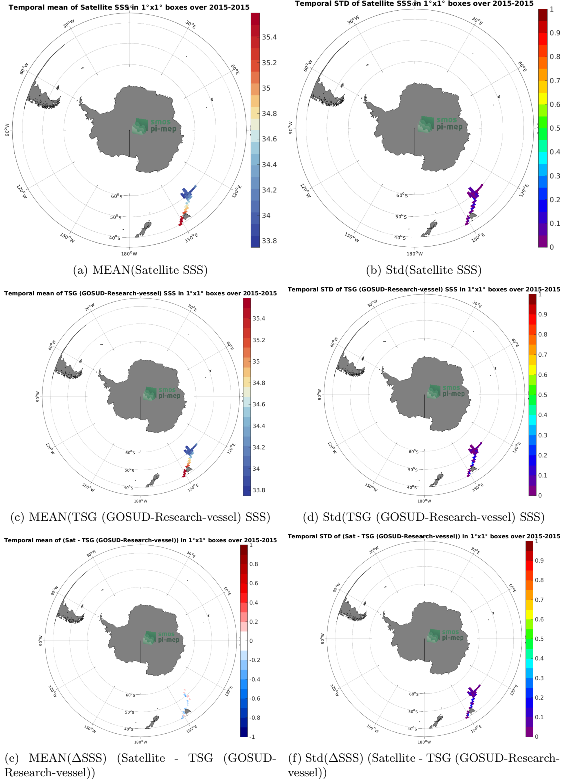
Figure 6: Temporal mean (left) and Std (right) of SSS from SMAP SSS L4 OI v2 - 7 Days (ESR) (top), TSG (GOSUD-Research-vessel) (middle), and of \Delta SSS (Satellite - TSG (GOSUD-Research-vessel)). Only match-up pairs are used to generate these maps.
