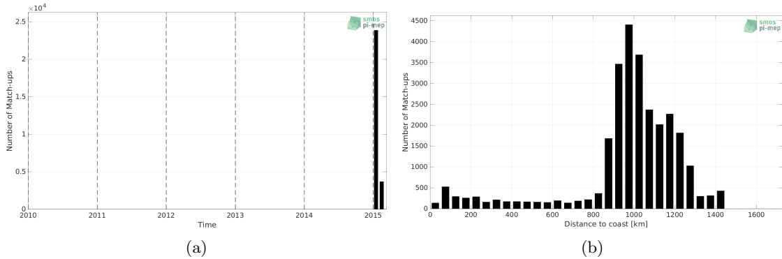
Figure 1: Number of match-ups between TSG (GOSUD-Research-vessel) and SMAP SSS L4 OI v2 - 7 Days (ESR) SSS as a function of time (a) and as function of the distance to coast (b) over the Roaring Forties and Furious Fifties Pi-MEP region and for the full satellite product period.
