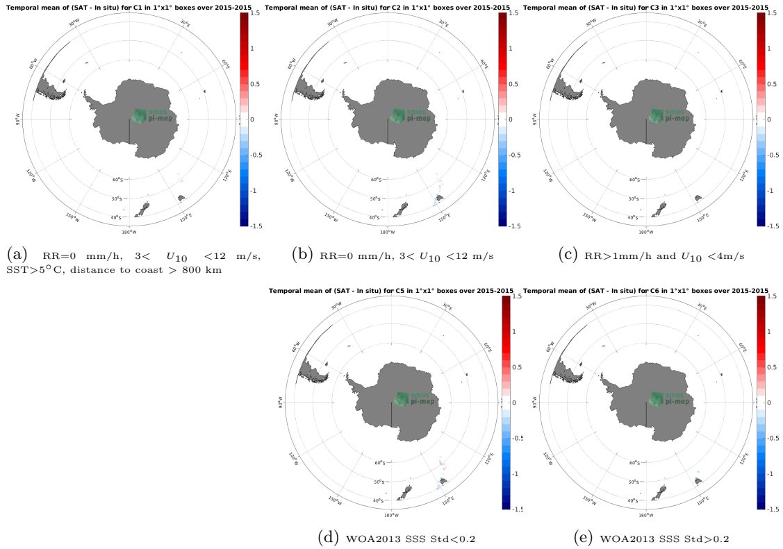
Figure 12: Temporal mean gridded over spatial boxes of size 1^\circ \times 1^\circ of \Delta SSS (SMAP SSS L4 OI v2 - 7 Days (ESR) - TSG (GOSUD-Research-vessel)) for 5 different subdatasets corresponding to: RR=0 mm/h, 3 < U_{10} < 12 m/s, SST>5°C, distance to coast > 800 km (a), RR=0 mm/h, 3 < U_{10} < 12 m/s (b), RR>1mm/h and U_{10} < 4 m/s (c), WOA2013 SSS Std<0.2 (d), WOA2013 SSS Std>0.2 (e).
