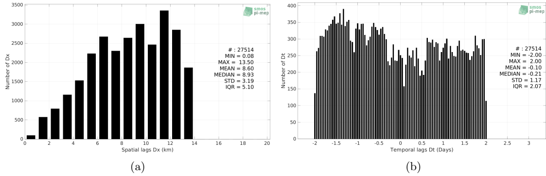
Figure 5: Histograms of the spatial (a) and temporal (b) lags between the location/time of the TSG (GOSUD-Research-vessel) measurement and the date of the corresponding SMAP SSS L4 OI v2 - 7 Days (ESR) SSS pixel.
