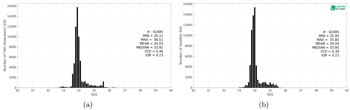
Figure 2: Histograms of SSS from TSG (Polarstern) (a) and SMAP SSS L4 OI v2 - Monthly (IPRC) (b) considering all match-up pairs per bins of 0.1 over the Roaring Forties and Furious Fifties Pi-MEP region and for the full satellite product period.
