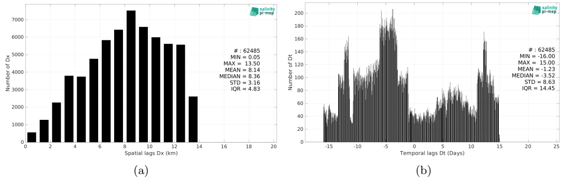
Figure 5: Histograms of the spatial (a) and temporal (b) lags between the location/time of the TSG (Polarstern) measurement and the date of the corresponding SMAP SSS L4 OI v2 - Monthly (IPRC) SSS pixel.
