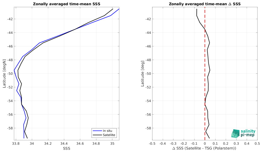
Figure 8: Left panel: Zonal mean SSS from SMAP SSS L4 OI v2 - Monthly (IPRC) satellite product (black) and from TSG (Polarstern) (blue). Right panel: Zonal mean of \Delta SSS (Satellite - TSG (Polarstern)) for all the collected Pi-MEP match-up pairs estimated over the full satellite product period.
