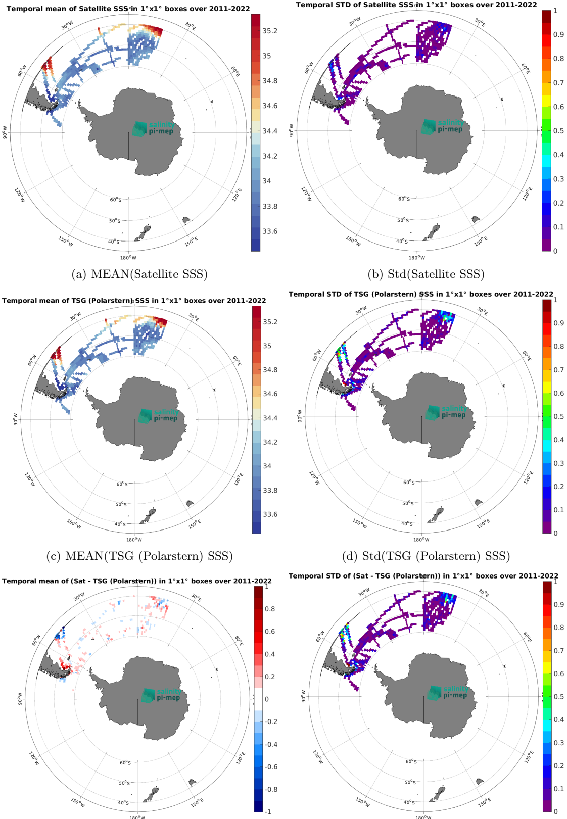
Figure 6: Temporal mean (left) and Std (right) of SSS from SMAP SSS L4 OI v2 - Monthly (IPRC) (top), TSG (Polarstern) (middle), and of \Delta SSS (Satellite - TSG (Polarstern)). Only match-up pairs are used to generate these maps.
