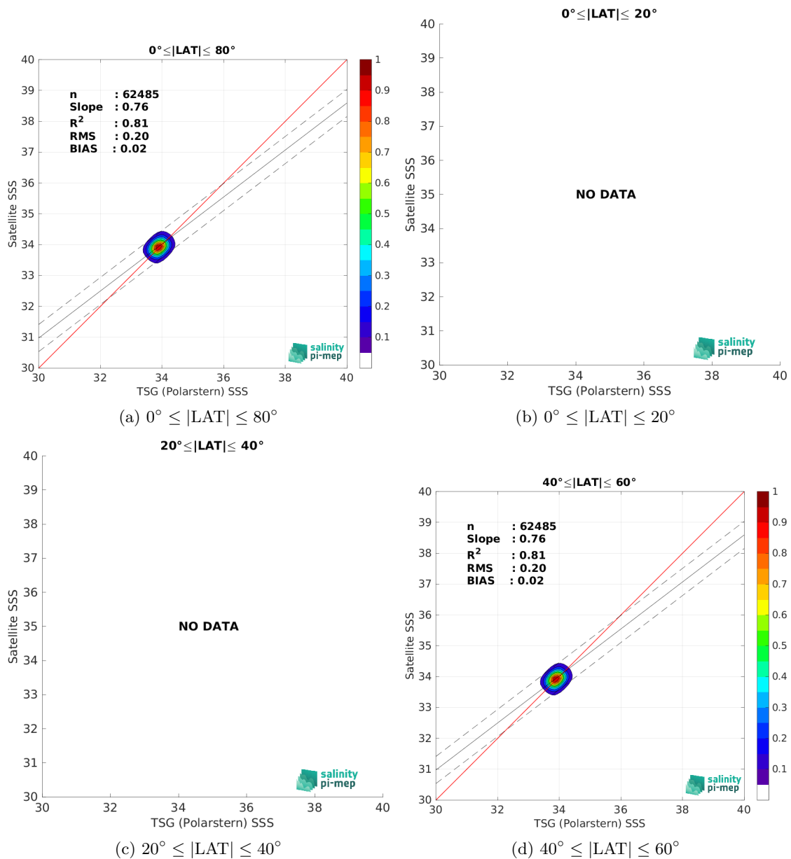
Figure 9: Contour maps of the concentration of SMAP SSS L4 OI v2 - Monthly (IPRC) SSS (y-axis) versus TSG (Polarstern) SSS (x-axis) at match-up pairs for different latitude bands. For each plot, the red line shows x=y . The black thin and dashed lines indicate a linear fit through the data cloud and the \pm 95\% confidence levels, respectively. The number match-up pairs n , the slope and R^2 coefficient of the linear fit, the root mean square (RMS) and the mean bias between satellite and in situ data are indicated for each latitude band in each plots.
