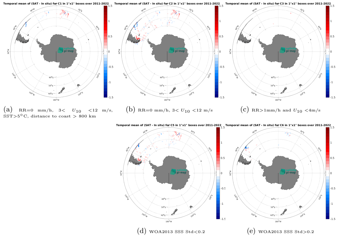
Figure 12: Temporal mean gridded over spatial boxes of size 1^{\circ}\times 1^{\circ} of \Delta\text{SSS} (SMAP SSS L4 OI v2 - Monthly (IPRC) - TSG (Polarstern)) for 5 different subdatasets corresponding to:RR=0 mm/h, 3 < U_{10} < 12 m/s, SST >5^{\circ}\text{C} , distance to coast > 800 km (a), RR=0 mm/h, 3 < U_{10} < 12 m/s (b), RR >1 mm/h and U_{10} < 4 m/s (c), WOA2013 SSS Std <0.2 (d), WOA2013 SSS Std >0.2 (e).
