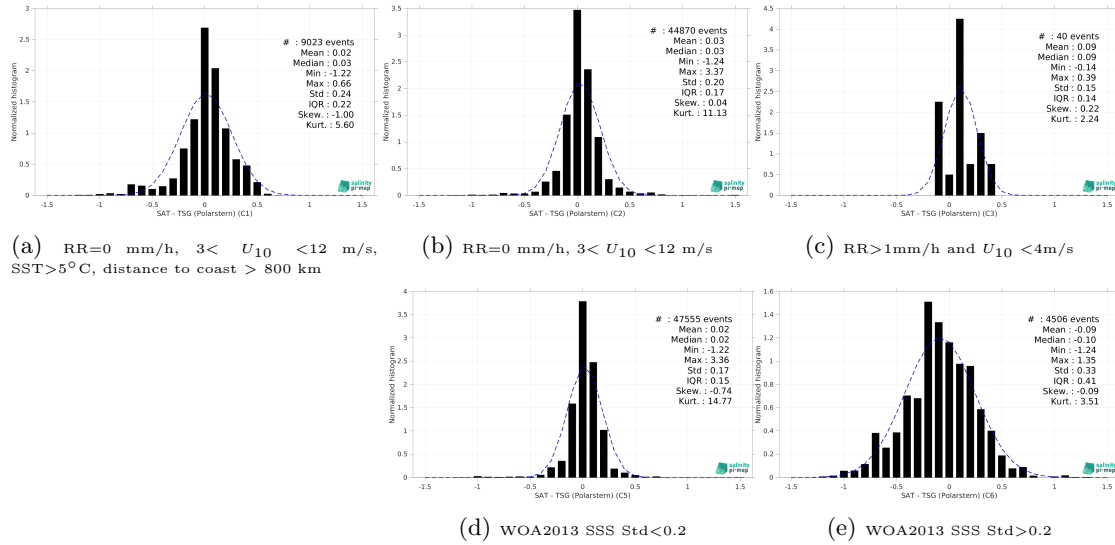
Figure 13: Normalized histogram of \Delta SSS (SMAP SSS L4 OI v2 - Monthly (IPRC) - TSG (Polarstern)) for 5 different subdatasets corresponding to: RR=0 mm/h, 3 < U_{10} < 12 m/s, SST>5°C, distance to coast > 800 km (a), RR=0 mm/h, 3 < U_{10} < 12 m/s (b), RR>1mm/h and U_{10} < 4 m/s (c), WOA2013 SSS Std<0.2 (d), WOA2013 SSS Std>0.2 (e).
