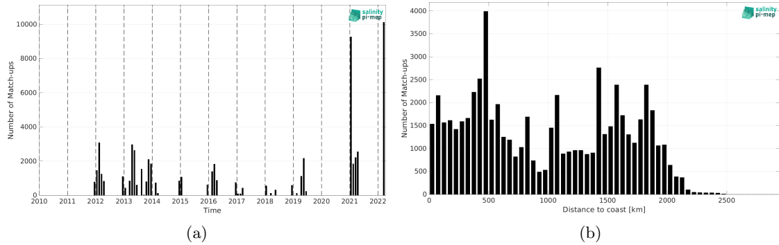
Figure 1: Number of match-ups between TSG (Polarstern) and SMAP SSS L4 OI v2 - Monthly (IPRC) SSS as a function of time (a) and as function of the distance to coast (b) over the Roaring Forties and Furious Fifties Pi-MEP region and for the full satellite product period.
