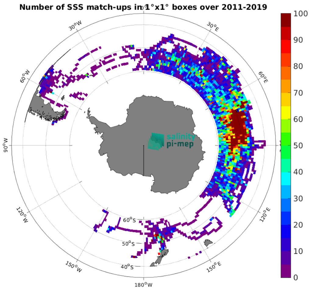
Figure 4: Number of SSS match-ups between Marine mammals SSS and the SMAP SSS L4 OI v2 - Monthly (IPRC) SSS product for the Roaring Forties and Furious Fifties Pi-MEP region over 1^{\circ} \times 1^{\circ} boxes and for the full satellite product period.
