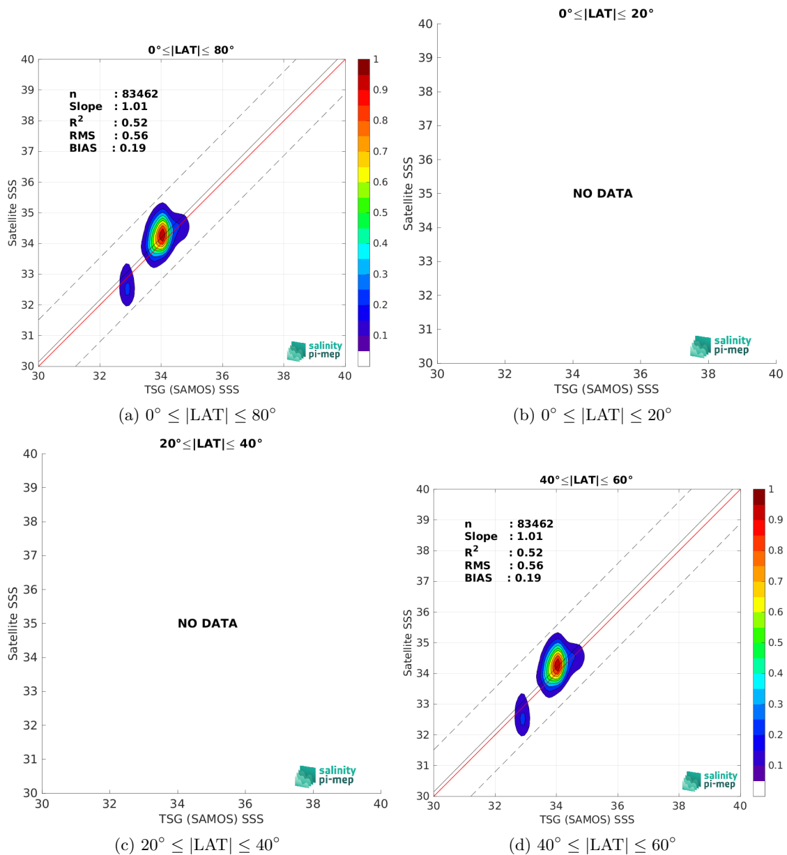
Figure 10: Contour maps of the concentration of SMAP SSS L3 v6 - 8-Day running (RSS) SSS (y-axis) versus TSG (SAMOS) SSS (x-axis) at match-up pairs for different latitude bands. For each plot, the red line shows x=y . The black thin and dashed lines indicate a linear fit through the data cloud and the \pm 95\% confidence levels, respectively. The number match-up pairs n , the slope and R^2 coefficient of the linear fit, the root mean square (RMS) and the mean bias between satellite and in situ data are indicated for each latitude band in each plots.
