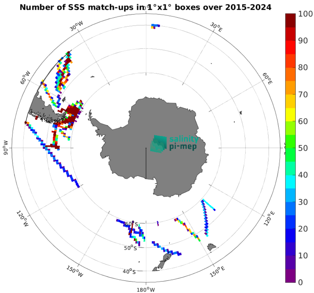
Figure 5: Number of SSS match-ups between TSG (SAMOS) SSS and the SMAP SSS L3 v6 - 8-Day running (RSS) SSS product for the Roaring Forties and Furious Fifties Pi-MEP region over 1^\circ \times 1^\circ boxes and for the full satellite product period.
