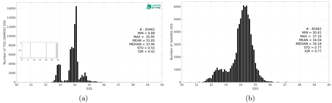
Figure 3: Histograms of SSS from TSG (SAMOS) (a) and SMAP SSS L3 v6 - 8-Day running (RSS) (b) considering all match-up pairs per bins of 0.1 over the Roaring Forties and Furious Fifties Pi-MEP region and for the full satellite product period.
