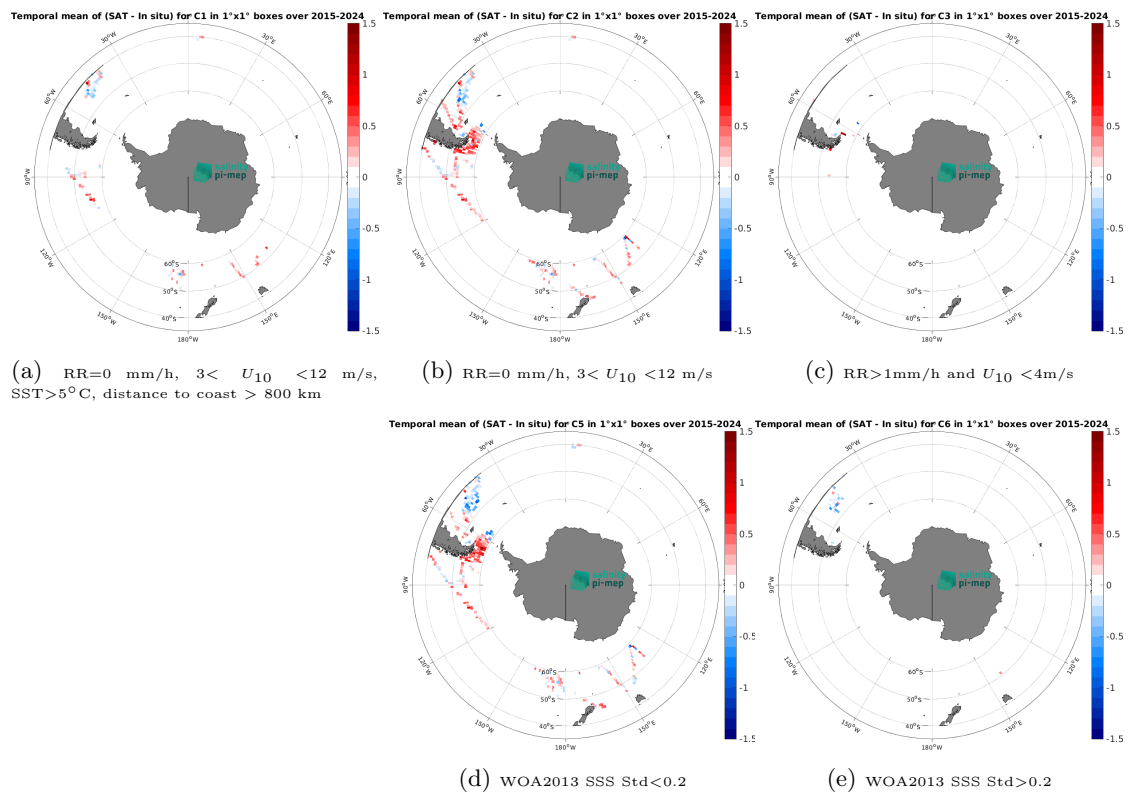
Figure 14: Temporal mean gridded over spatial boxes of size 1^\circ \times 1^\circ of \Delta SSS (SMAP SSS L3 v6 - 8-Day running (RSS) - TSG (SAMOS)) for 5 different subdatasets corresponding to:RR=0 mm/h, 3 < U_{10} < 12 m/s, SST >5^\circ C, distance to coast > 800 km (a), RR=0 mm/h, 3 < U_{10} < 12 m/s (b), RR >1 mm/h and U_{10} < 4 m/s (c), WOA2013 SSS Std <0.2 (d), WOA2013 SSS Std >0.2 (e).
