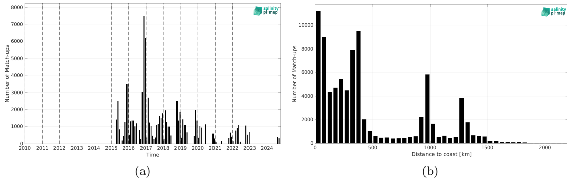
Figure 2: Number of match-ups between TSG (SAMOS) and SMAP SSS L3 v6 - 8-Day running (RSS) SSS as a function of time (a) and as function of the distance to coast (b) over the Roaring Forties and Furious Fifties Pi-MEP region and for the full satellite product period.
