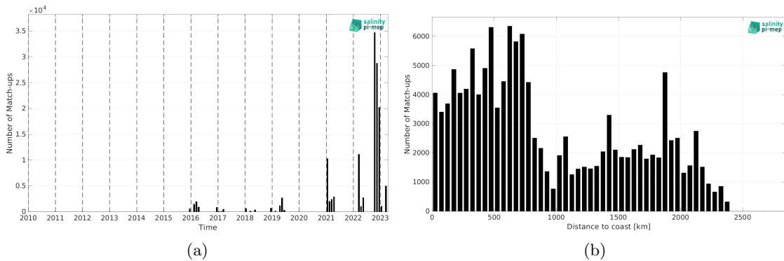
Figure 2: Number of match-ups between TSG (Polarstern) and SMAP SSS L3 v6 - 8-Day running (RSS) SSS as a function of time (a) and as function of the distance to coast (b) over the Roaring Forties and Furious Fifties Pi-MEP region and for the full satellite product period.
