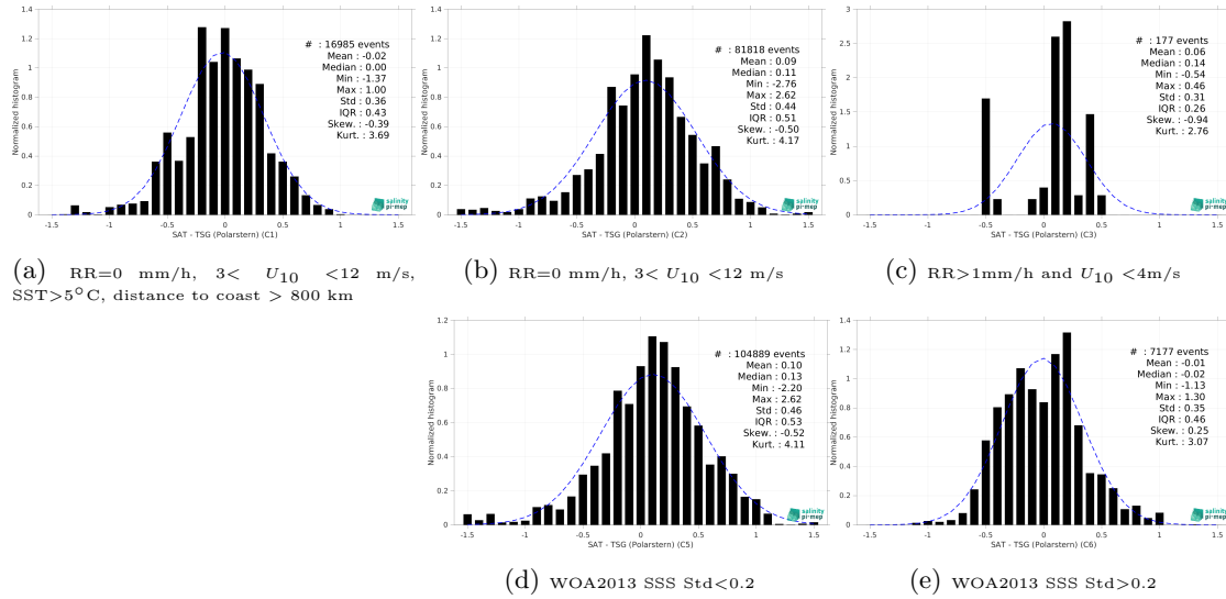
Figure 15: Normalized histogram of \Delta\text{SSS} (SMAP SSS L3 v6 - 8-Day running (RSS) - TSG (Polarstern)) for 5 different subdatasets corresponding to: RR=0 mm/h, 3 < U_{10} < 12 m/s, SST>5°C, distance to coast > 800 km (a), RR=0 mm/h, 3 < U_{10} < 12 m/s (b), RR>1mm/h and U_{10} < 4 m/s (c), WOA2013 SSS Std<0.2 (d), WOA2013 SSS Std>0.2 (e).
