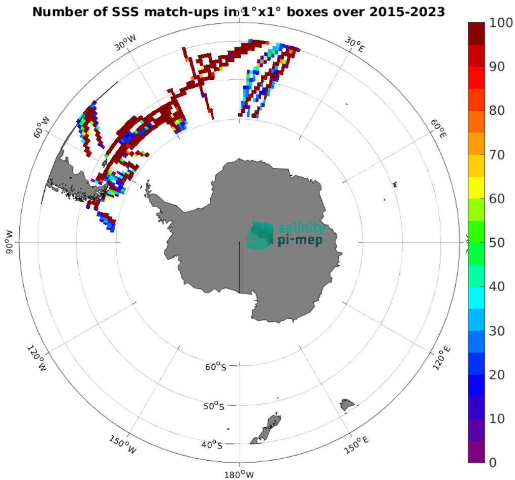
Figure 5: Number of SSS match-ups between TSG (Polarstern) SSS and the SMAP SSS L3 v6 - 8-Day running (RSS) SSS product for the Roaring Forties and Furious Fifties Pi-MEP region over 1^\circ \times 1^\circ boxes and for the full satellite product period.
