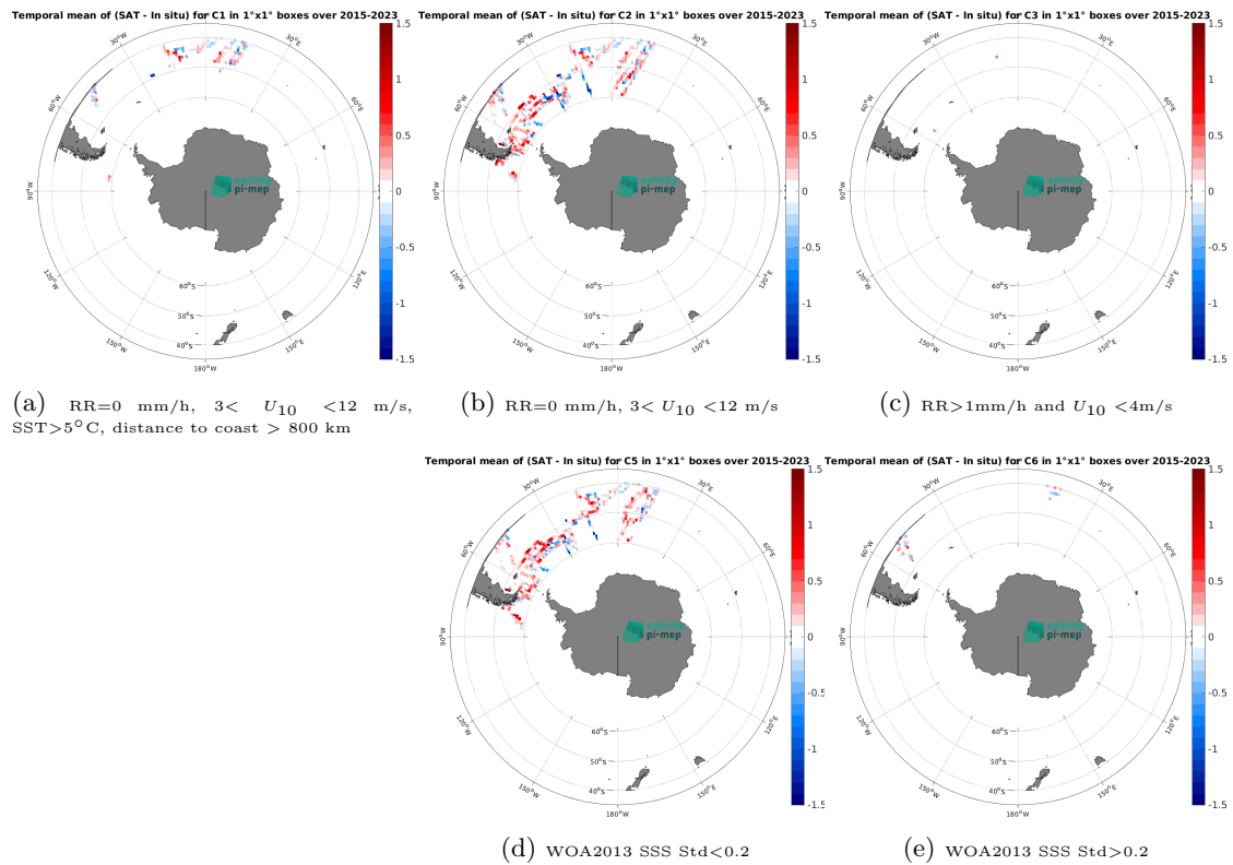
Figure 14: Temporal mean gridded over spatial boxes of size 1^\circ \times 1^\circ of \Delta SSS (SMAP SSS L3 v6 - 8-Day running (RSS) - TSG (Polarstern)) for 5 different subdatasets corresponding to: RR=0 mm/h, 3 < U_{10} < 12 m/s, SST > 5^\circ\text{C} , distance to coast > 800 km (a), RR=0 mm/h, 3 < U_{10} < 12 m/s (b), RR > 1 mm/h and U_{10} < 4 m/s (c), WOA2013 SSS Std < 0.2 (d), WOA2013 SSS Std > 0.2 (e).
