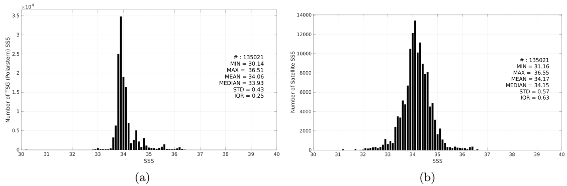
Figure 3: Histograms of SSS from TSG (Polarstern) (a) and SMAP SSS L3 v6 - 8-Day running (RSS) (b) considering all match-up pairs per bins of 0.1 over the Roaring Forties and Furious Fifties Pi-MEP region and for the full satellite product period.
