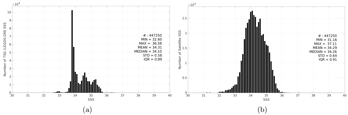
Figure 3: Histograms of SSS from TSG (LEGOS-DM) (a) and SMAP SSS L3 v6 - 8-Day running (RSS) (b) considering all match-up pairs per bins of 0.1 over the Roaring Forties and Furious Fifties Pi-MEP region and for the full satellite product period.
