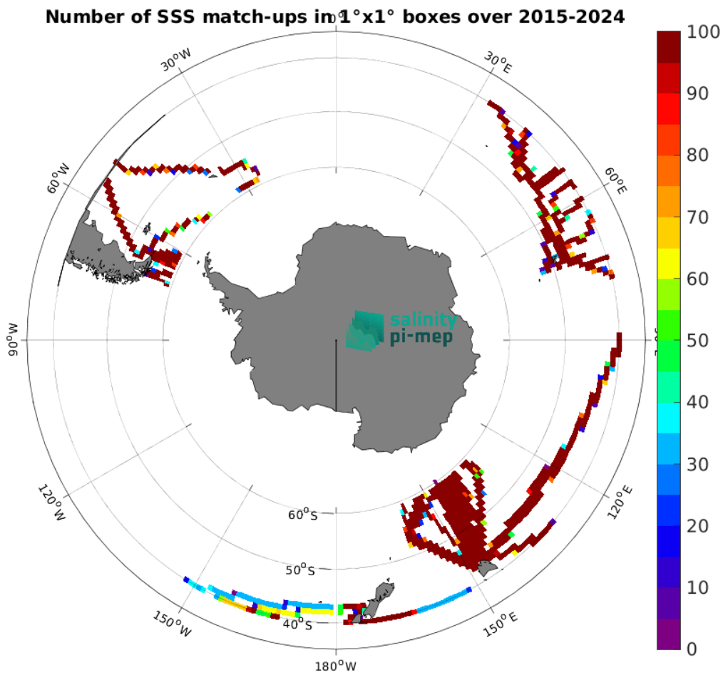
Figure 5: Number of SSS match-ups between TSG (LEGOS-DM) SSS and the SMAP SSS L3 v6 - 8-Day running (RSS) SSS product for the Roaring Forties and Furious Fifties Pi-MEP region over 1^{\circ} \times 1^{\circ} boxes and for the full satellite product period.
