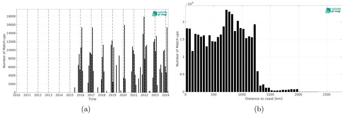
Figure 2: Number of match-ups between TSG (LEGOS-DM) and SMAP SSS L3 v6 - 8-Day running (RSS) SSS as a function of time (a) and as function of the distance to coast (b) over the Roaring Forties and Furious Fifties Pi-MEP region and for the full satellite product period.
