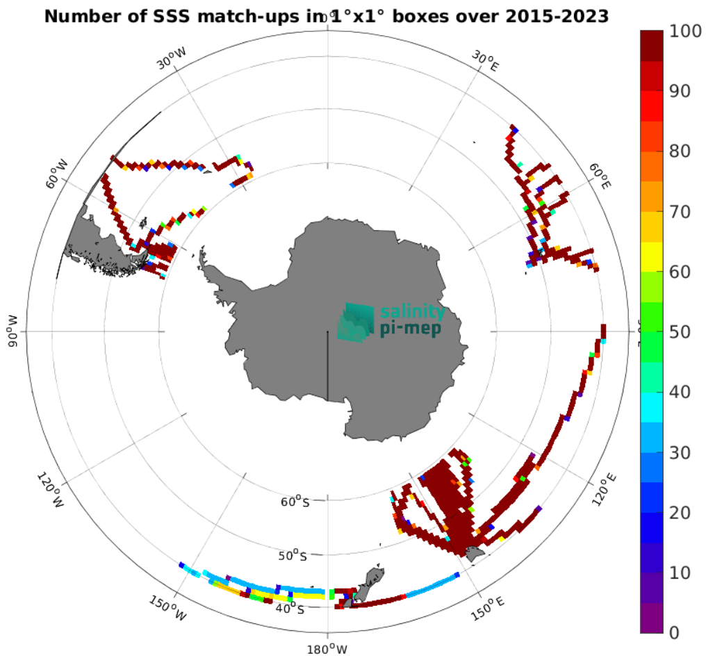
Figure 5: Number of SSS match-ups between TSG (LEGOS-DM) SSS and the SMAP SSS L3 v6 - 8-Day running (RSS) SSS product for the Roaring Forties and Furious Fifties Pi-MEP region over 1^\circ \times 1^\circ boxes and for the full satellite product period.
