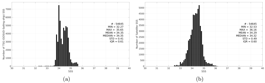
Figure 3: Histograms of SSS from TSG (GOSUD-Sailing-ship) (a) and SMAP SSS L3 v6 - 8-Day running (RSS) (b) considering all match-up pairs per bins of 0.1 over the Roaring Forties and Furious Fifties Pi-MEP region and for the full satellite product period.
