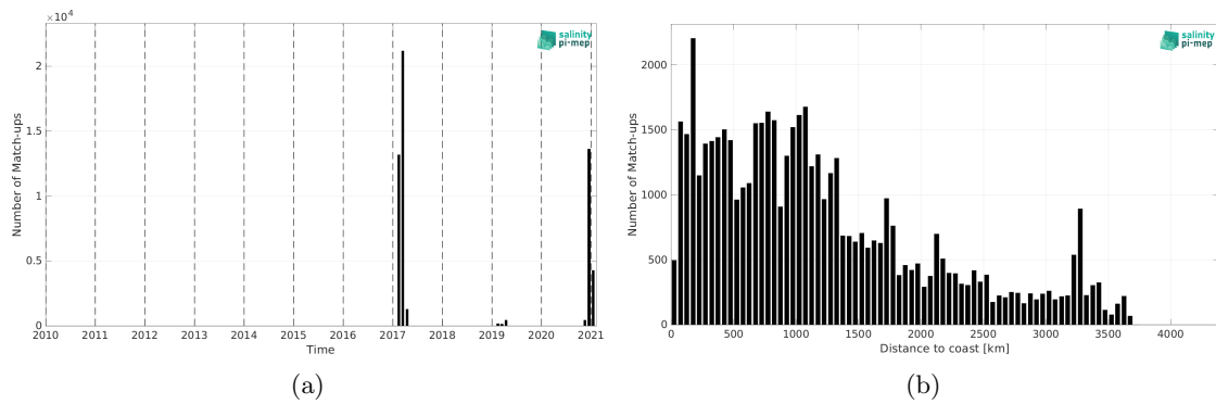
Figure 2: Number of match-ups between TSG (GOSUD-Sailing-ship) and SMAP SSS L3 v6 - 8-Day running (RSS) SSS as a function of time (a) and as function of the distance to coast (b) over the Roaring Forties and Furious Fifties Pi-MEP region and for the full satellite product period.
