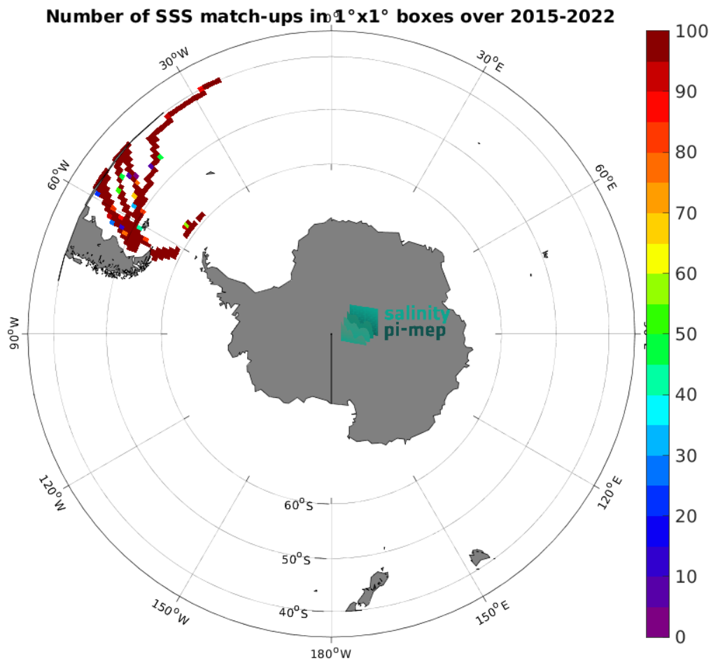
Figure 5: Number of SSS match-ups between TSG (CSIC-UTM) SSS and the SMAP SSS L3 v6 - 8-Day running (RSS) SSS product for the Roaring Forties and Furious Fifties Pi-MEP region over 1^\circ \times 1^\circ boxes and for the full satellite product period.
