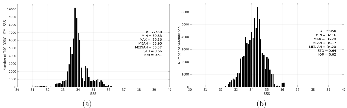
Figure 3: Histograms of SSS from TSG (CSIC-UTM) (a) and SMAP SSS L3 v6 - 8-Day running (RSS) (b) considering all match-up pairs per bins of 0.1 over the Roaring Forties and Furious Fifties Pi-MEP region and for the full satellite product period.
