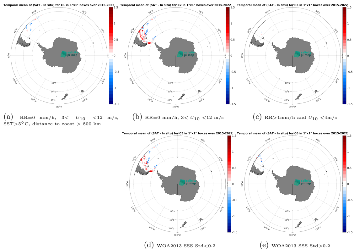
Figure 14: Temporal mean gridded over spatial boxes of size 1^\circ \times 1^\circ of \Delta SSS (SMAP SSS L3 v6 - 8-Day running (RSS) - TSG (CSIC-UTM)) for 5 different subdatasets corresponding to:RR=0 mm/h, 3 < U_{10} < 12 m/s, SST > 5^\circ\text{C} , distance to coast > 800 km (a), RR=0 mm/h, 3 < U_{10} < 12 m/s (b), RR > 1 mm/h and U_{10} < 4 m/s (c), WOA2013 SSS Std < 0.2 (d), WOA2013 SSS Std > 0.2 (e).
