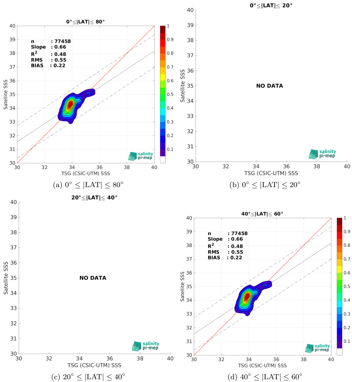
Figure 10: Contour maps of the concentration of SMAP SSS L3 v6 - 8-Day running (RSS) SSS (y-axis) versus TSG (CSIC-UTM) SSS (x-axis) at match-up pairs for different latitude bands. For each plot, the red line shows x=y . The black thin and dashed lines indicate a linear fit through the data cloud and the \pm 95\% confidence levels, respectively. The number match-up pairs n , the slope and R^2 coefficient of the linear fit, the root mean square (RMS) and the mean bias between satellite and in situ data are indicated for each latitude band in each plots.
