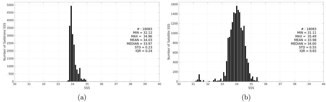
Figure 3: Histograms of SSS from Saildrone (a) and SMAP SSS L3 v6 - 8-Day running (RSS) (b) considering all match-up pairs per bins of 0.1 over the Roaring Forties and Furious Fifties Pi-MEP region and for the full satellite product period.
