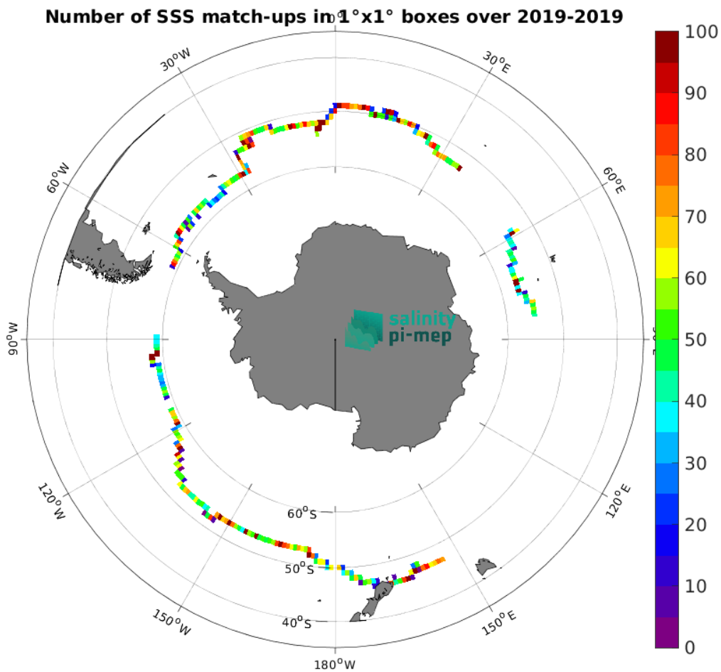
Figure 5: Number of SSS match-ups between Saildrone SSS and the SMAP SSS L3 v6 - 8-Day running (RSS) SSS product for the Roaring Forties and Furious Fifties Pi-MEP region over 1^\circ \times 1^\circ boxes and for the full satellite product period.
