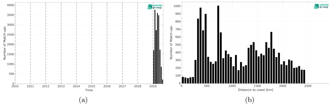
Figure 2: Number of match-ups between Saildrone and SMAP SSS L3 v6 - 8-Day running (RSS) SSS as a function of time (a) and as function of the distance to coast (b) over the Roaring Forties and Furious Fifties Pi-MEP region and for the full satellite product period.
