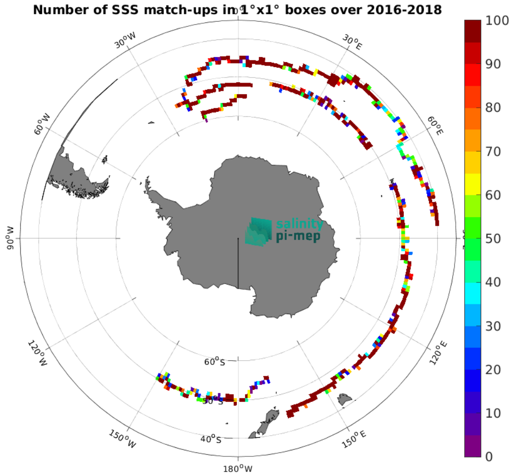
Figure 4: Number of SSS match-ups between Surface drifters SSS and the SMAP SSS L3 v6 - 8-Day running (RSS) SSS product for the Roaring Forties and Furious Fifties Pi-MEP region over 1^\circ \times 1^\circ boxes and for the full satellite product period.
