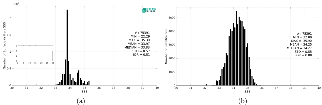
Figure 3: Histograms of SSS from Surface drifters (a) and SMAP SSS L3 v6 - 8-Day running (RSS) (b) considering all match-up pairs per bins of 0.1 over the Roaring Forties and Furious Fifties Pi-MEP region and for the full satellite product period.
