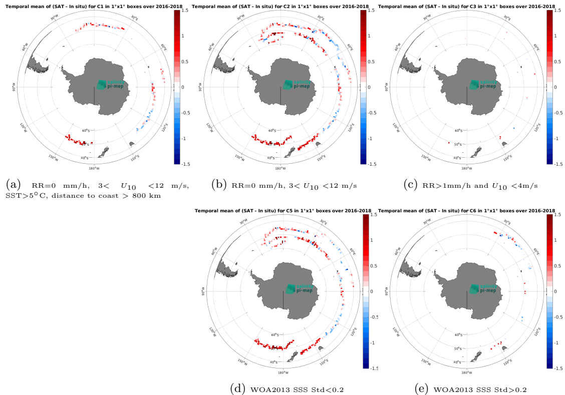
Figure 13: Temporal mean gridded over spatial boxes of size 1^\circ \times 1^\circ of \Delta SSS (SMAP SSS L3 v6 - 8-Day running (RSS) - Surface drifters) for 5 different subdatasets corresponding to:RR=0 mm/h, 3 < U_{10} < 12 m/s, SST >5^\circ\text{C} , distance to coast > 800 km (a), RR=0 mm/h, 3 < U_{10} < 12 m/s (b), RR >1 mm/h and U_{10} < 4 m/s (c), WOA2013 SSS Std <0.2 (d), WOA2013 SSS Std >0.2 (e).
