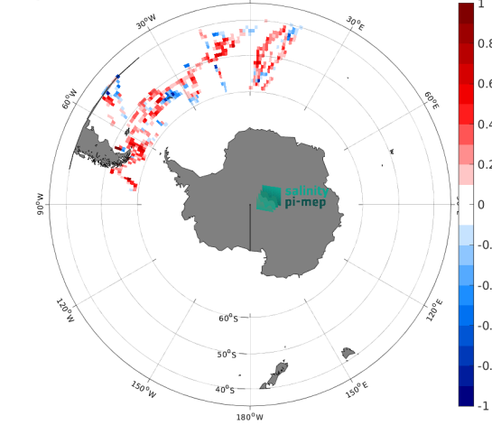
(e) MEAN( \Delta SSS) (Satellite - TSG (Polarstern)) 17
