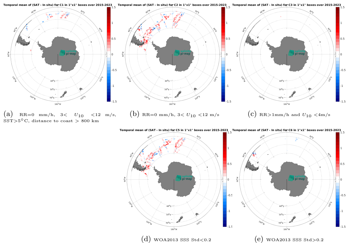
Figure 14: Temporal mean gridded over spatial boxes of size 1^\circ \times 1^\circ of \Delta SSS (SMAP SSS L3 v6 - Monthly (RSS) - TSG (Polarstern)) for 5 different subdatasets corresponding to: RR=0 mm/h, 3 < U_{10} < 12 m/s, SST > 5°C, distance to coast > 800 km (a), RR=0 mm/h, 3 < U_{10} < 12 m/s (b), RR > 1mm/h and U_{10} < 4 m/s (c), WOA2013 SSS Std < 0.2 (d), WOA2013 SSS Std > 0.2 (e).
