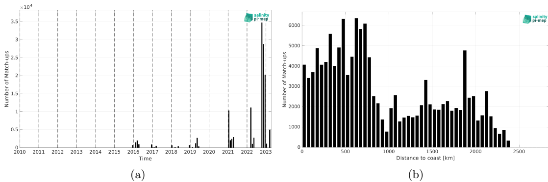
Figure 2: Number of match-ups between TSG (Polarstern) and SMAP SSS L3 v6 - Monthly (RSS) SSS as a function of time (a) and as function of the distance to coast (b) over the Roaring Forties and Furious Fifties Pi-MEP region and for the full satellite product period.
