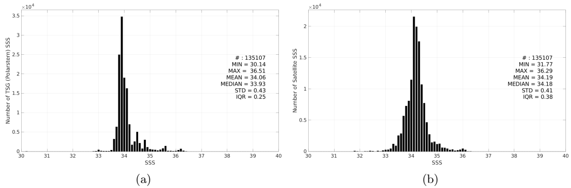
Figure 3: Histograms of SSS from TSG (Polarstern) (a) and SMAP SSS L3 v6 - Monthly (RSS) (b) considering all match-up pairs per bins of 0.1 over the Roaring Forties and Furious Fifties Pi-MEP region and for the full satellite product period.
