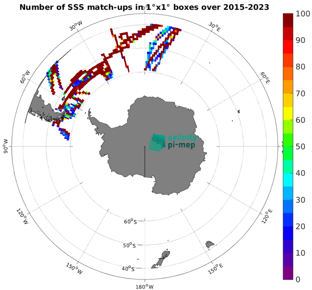
Figure 5: Number of SSS match-ups between TSG (Polarstern) SSS and the SMAP SSS L3 v6 - Monthly (RSS) SSS product for the Roaring Forties and Furious Fifties Pi-MEP region over 1^\circ \times 1^\circ boxes and for the full satellite product period.
