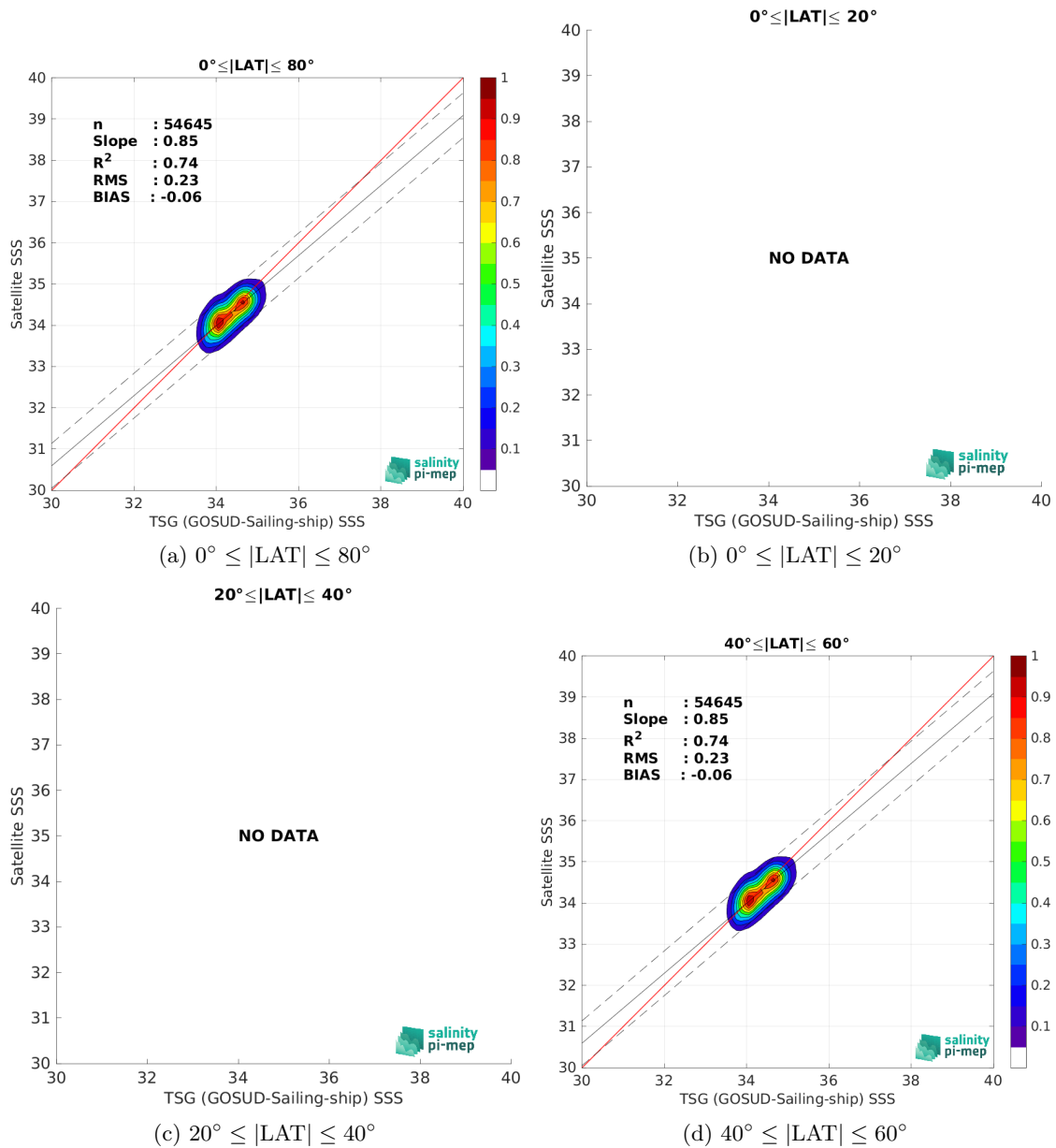
Figure 10: Contour maps of the concentration of SMAP SSS L3 v6 - Monthly (RSS) SSS (y-axis) versus TSG (GOSUD-Sailing-ship) SSS (x-axis) at match-up pairs for different latitude bands. For each plot, the red line shows x=y . The black thin and dashed lines indicate a linear fit through the data cloud and the \pm 95\% confidence levels, respectively. The number match-up pairs n , the slope and R^2 coefficient of the linear fit, the root mean square (RMS) and the mean bias between satellite and in situ data are indicated for each latitude band in each plots.
