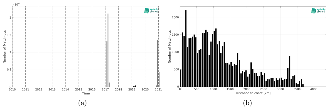
Figure 2: Number of match-ups between TSG (GOSUD-Sailing-ship) and SMAP SSS L3 v6 - Monthly (RSS) SSS as a function of time (a) and as function of the distance to coast (b) over the Roaring Forties and Furious Fifties Pi-MEP region and for the full satellite product period.
