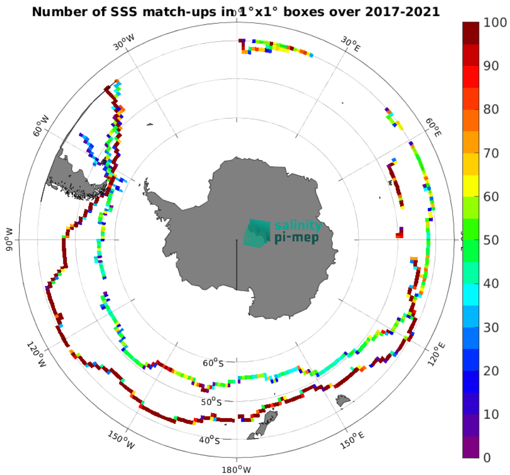
Figure 5: Number of SSS match-ups between TSG (GOSUD-Sailing-ship) SSS and the SMAP SSS L3 v6 - Monthly (RSS) SSS product for the Roaring Forties and Furious Fifties Pi-MEP region over 1^\circ \times 1^\circ boxes and for the full satellite product period.
