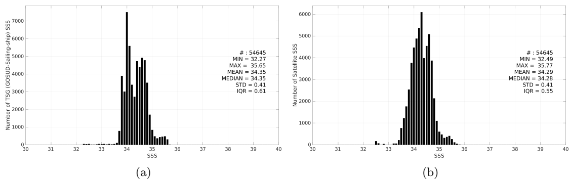
Figure 3: Histograms of SSS from TSG (GOSUD-Sailing-ship) (a) and SMAP SSS L3 v6 - Monthly (RSS) (b) considering all match-up pairs per bins of 0.1 over the Roaring Forties and Furious Fifties Pi-MEP region and for the full satellite product period.
