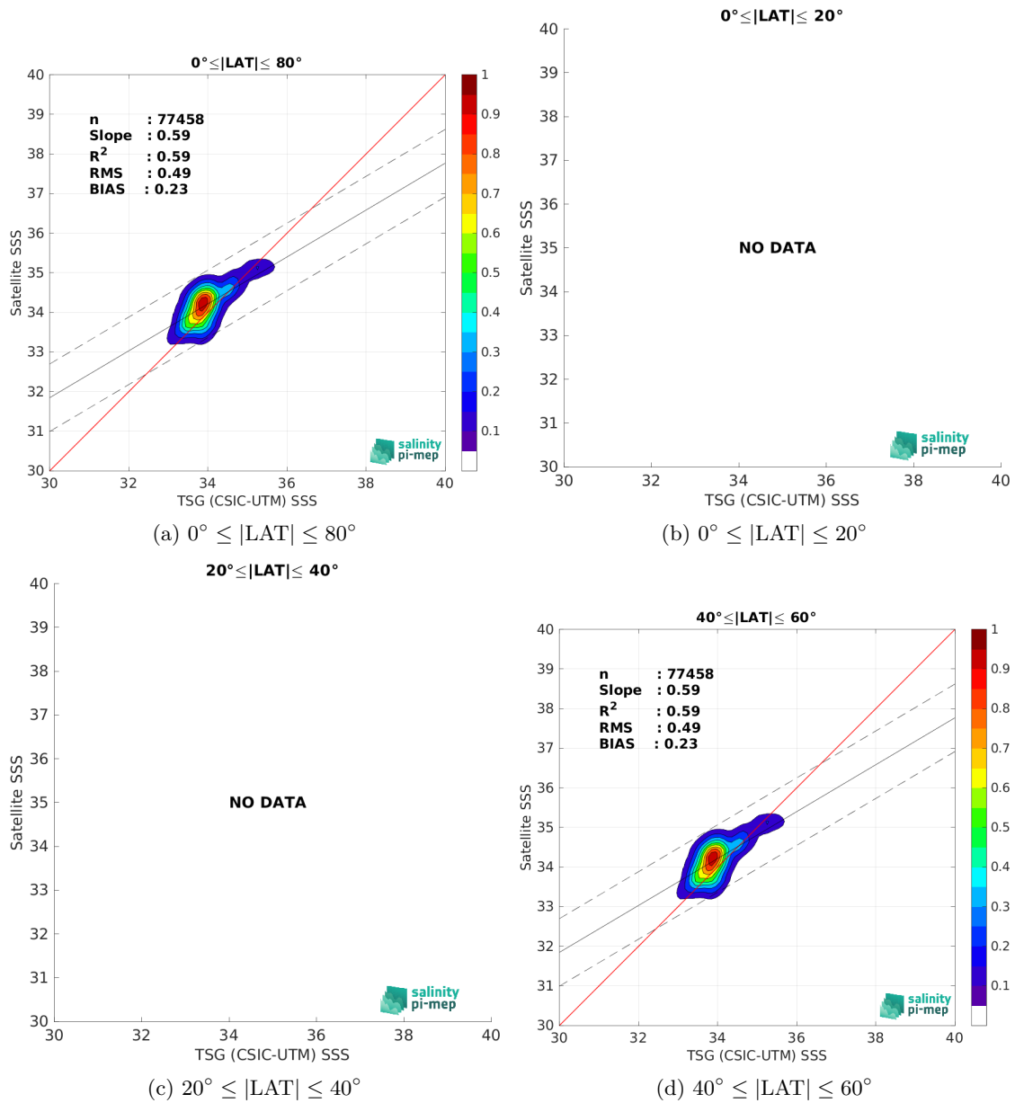
Figure 10: Contour maps of the concentration of SMAP SSS L3 v6 - Monthly (RSS) SSS (y-axis) versus TSG (CSIC-UTM) SSS (x-axis) at match-up pairs for different latitude bands. For each plot, the red line shows x=y . The black thin and dashed lines indicate a linear fit through the data cloud and the \pm 95\% confidence levels, respectively. The number match-up pairs n , the slope and R^2 coefficient of the linear fit, the root mean square (RMS) and the mean bias between satellite and in situ data are indicated for each latitude band in each plot.
