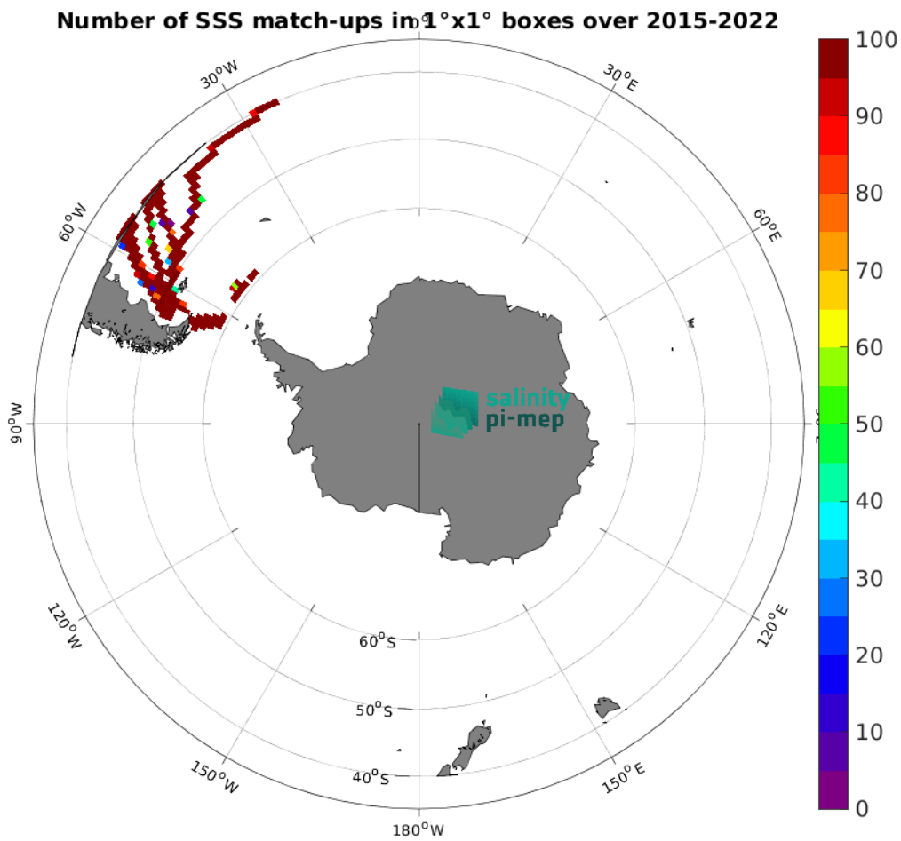
Figure 5: Number of SSS match-ups between TSG (CSIC-UTM) SSS and the SMAP SSS L3 v6 - Monthly (RSS) SSS product for the Roaring Forties and Furious Fifties Pi-MEP region over 1^\circ \times 1^\circ boxes and for the full satellite product period.
