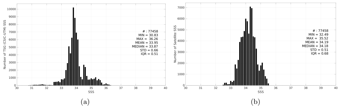
Figure 3: Histograms of SSS from TSG (CSIC-UTM) (a) and SMAP SSS L3 v6 - Monthly (RSS) (b) considering all match-up pairs per bins of 0.1 over the Roaring Forties and Furious Fifties Pi-MEP region and for the full satellite product period.
