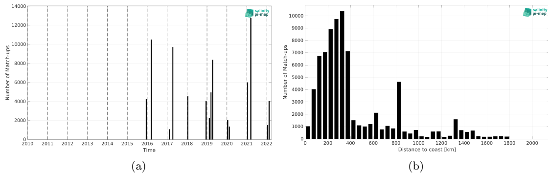
Figure 2: Number of match-ups between TSG (CSIC-UTM) and SMAP SSS L3 v6 - Monthly (RSS) SSS as a function of time (a) and as function of the distance to coast (b) over the Roaring Forties and Furious Fifties Pi-MEP region and for the full satellite product period.
