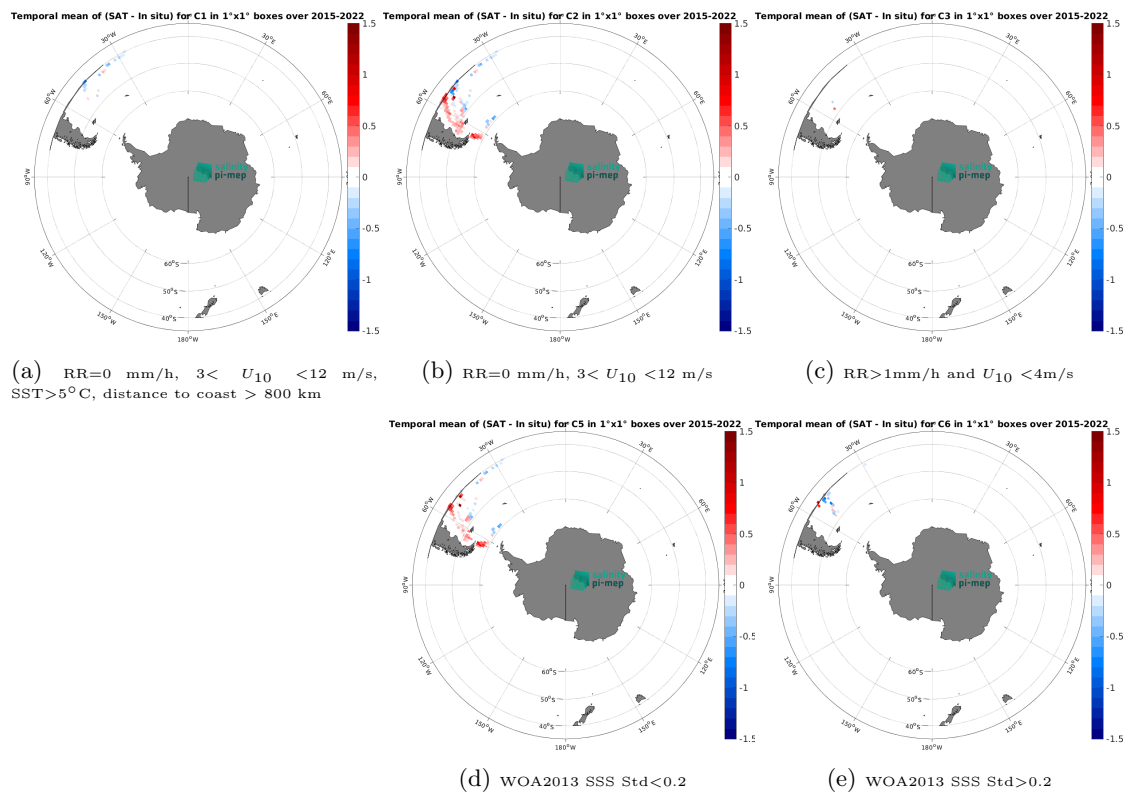
Figure 14: Temporal mean gridded over spatial boxes of size 1^\circ \times 1^\circ of \Delta SSS (SMAP SSS L3 v6 - Monthly (RSS) - TSG (CSIC-UTM)) for 5 different subdatasets corresponding to:RR=0 mm/h, 3 < U_{10} < 12 m/s, SST>5°C, distance to coast > 800 km (a), RR=0 mm/h, 3 < U_{10} < 12 m/s (b), RR>1mm/h and U_{10} < 4 m/s (c), WOA2013 SSS Std<0.2 (d), WOA2013 SSS Std>0.2 (e).
