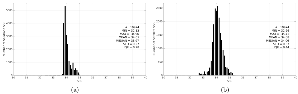
Figure 3: Histograms of SSS from Saildrone (a) and SMAP SSS L3 v6 - Monthly (RSS) (b) considering all match-up pairs per bins of 0.1 over the Roaring Forties and Furious Fifties Pi-MEP region and for the full satellite product period.
