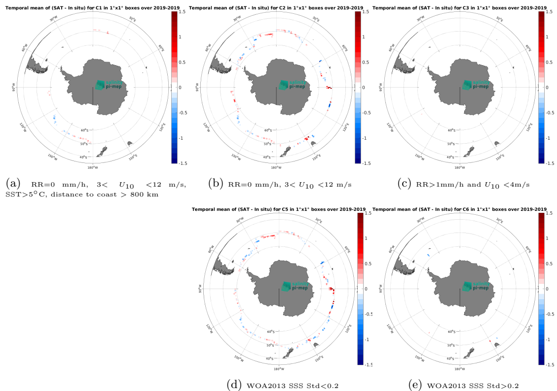
Figure 14: Temporal mean gridded over spatial boxes of size 1^\circ \times 1^\circ of \Delta SSS (SMAP SSS L3 v6 - Monthly (RSS) - Sairdrone) for 5 different subdatasets corresponding to:RR=0 mm/h, 3 < U_{10} < 12 m/s, SST>5°C, distance to coast > 800 km (a), RR=0 mm/h, 3 < U_{10} < 12 m/s (b), RR>1mm/h and U_{10} < 4 m/s (c), WOA2013 SSS Std<0.2 (d), WOA2013 SSS Std>0.2 (e).
