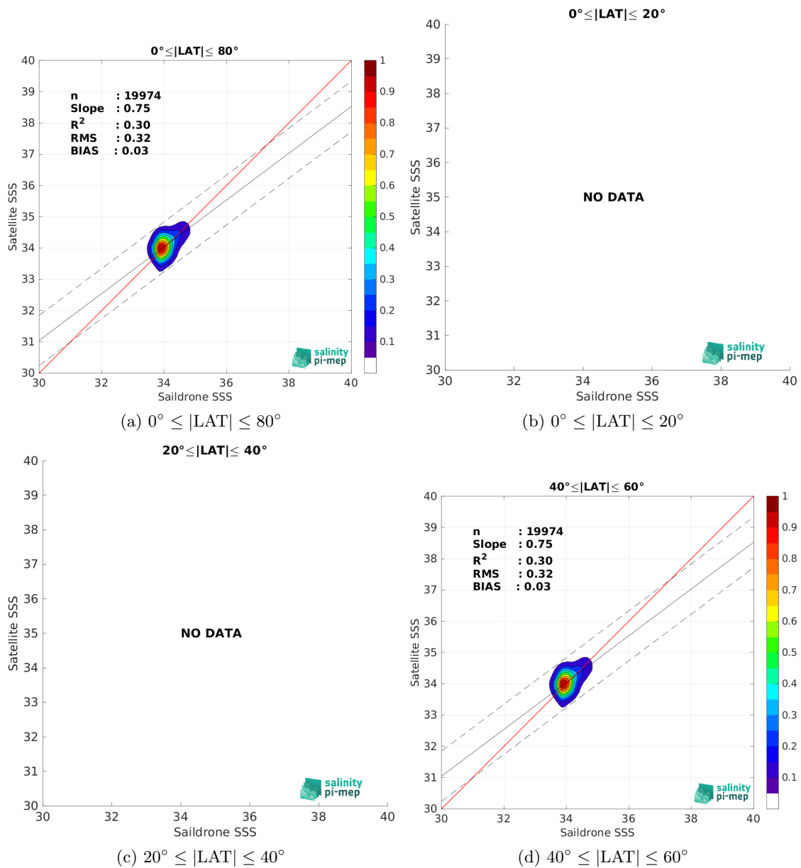
Figure 10: Contour maps of the concentration of SMAP SSS L3 v6 - Monthly (RSS) SSS (y-axis) versus Saldrone SSS (x-axis) at match-up pairs for different latitude bands. For each plot, the red line shows x=y . The black thin and dashed lines indicate a linear fit through the data cloud and the \pm 95\% confidence levels, respectively. The number match-up pairs n , the slope and R^2 coefficient of the linear fit, the root mean square (RMS) and the mean bias between satellite and in situ data are indicated for each latitude band in each plots.
