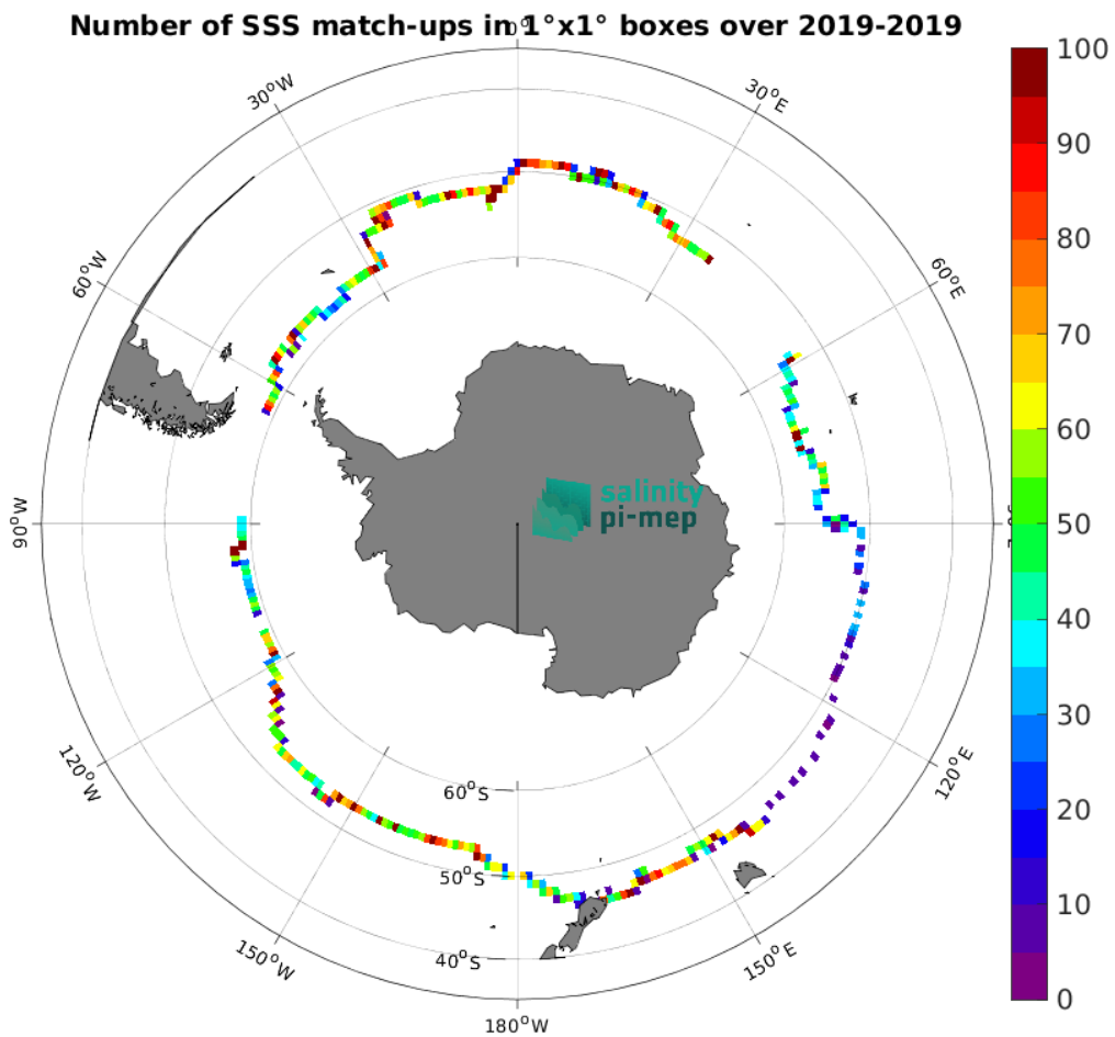
Figure 5: Number of SSS match-ups between Saildrone SSS and the SMAP SSS L3 v6 - Monthly (RSS) SSS product for the Roaring Forties and Furious Fifties Pi-MEP region over 1^\circ \times 1^\circ boxes and for the full satellite product period.
