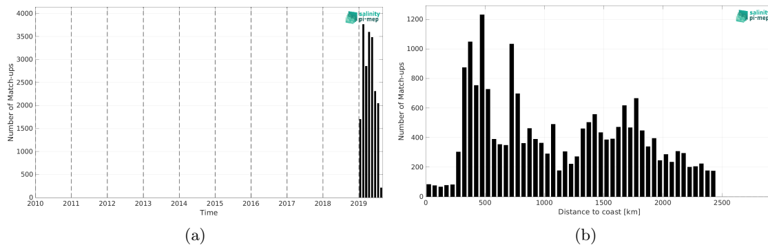
Figure 2: Number of match-ups between Saildrone and SMAP SSS L3 v6 - Monthly (RSS) SSS as a function of time (a) and as function of the distance to coast (b) over the Roaring Forties and Furious Fifties Pi-MEP region and for the full satellite product period.
