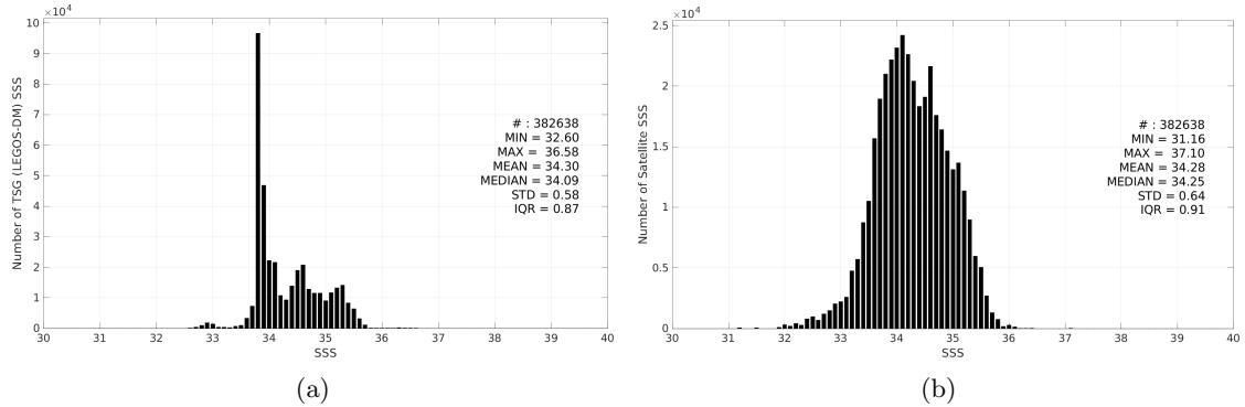
Figure 3: Histograms of SSS from TSG (LEGOS-DM) (a) and SMAP SSS L3 v5.3 - 8-Day running (RSS) (b) considering all match-up pairs per bins of 0.1 over the Roaring Forties and Furious Fifties Pi-MEP region and for the full satellite product period.
