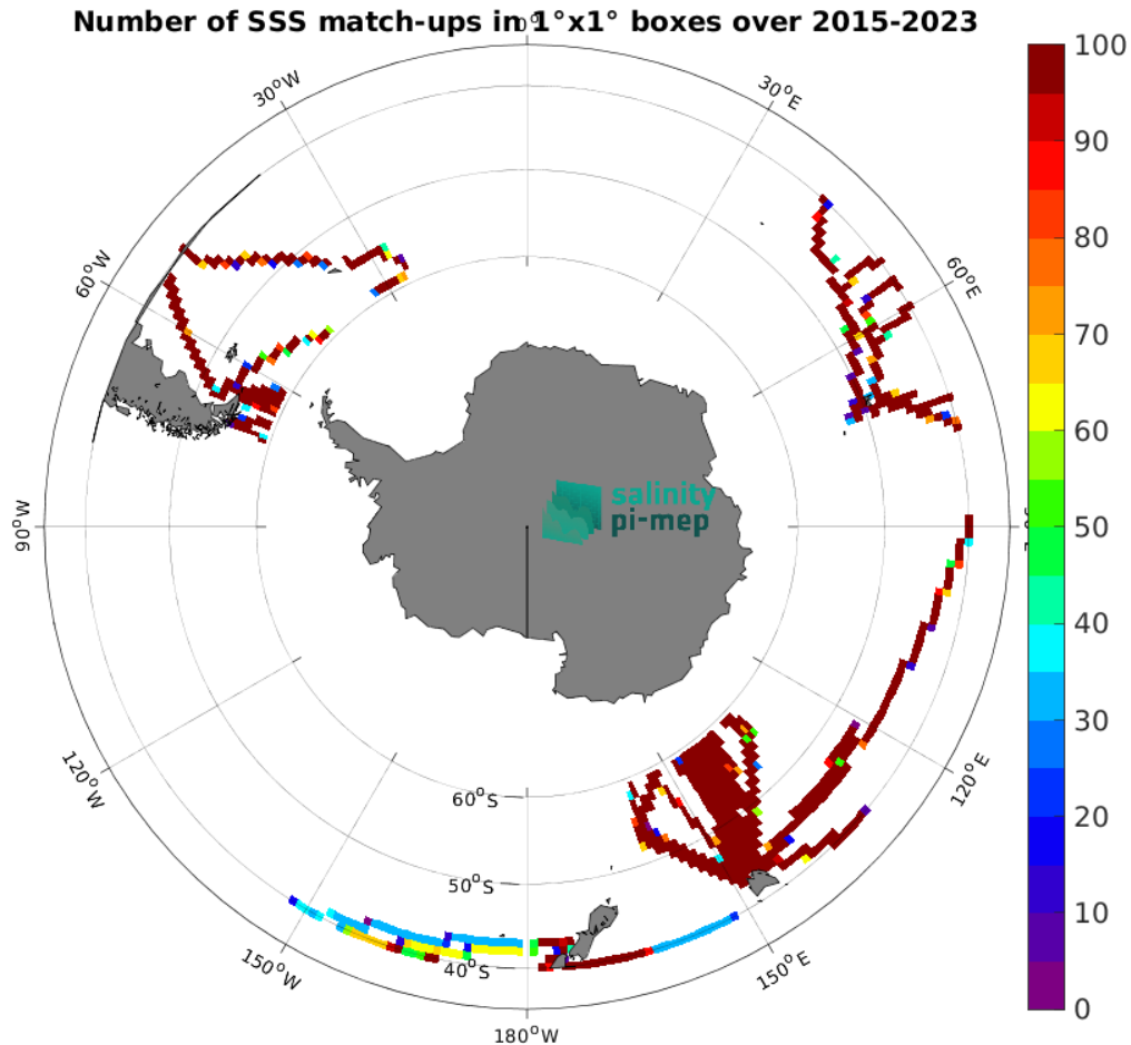
Figure 5: Number of SSS match-ups between TSG (LEGOS-DM) SSS and the SMAP SSS L3 v5.3 - 8-Day running (RSS) SSS product for the Roaring Forties and Furious Fifties Pi-MEP region over 1^\circ \times 1^\circ boxes and for the full satellite product period.
