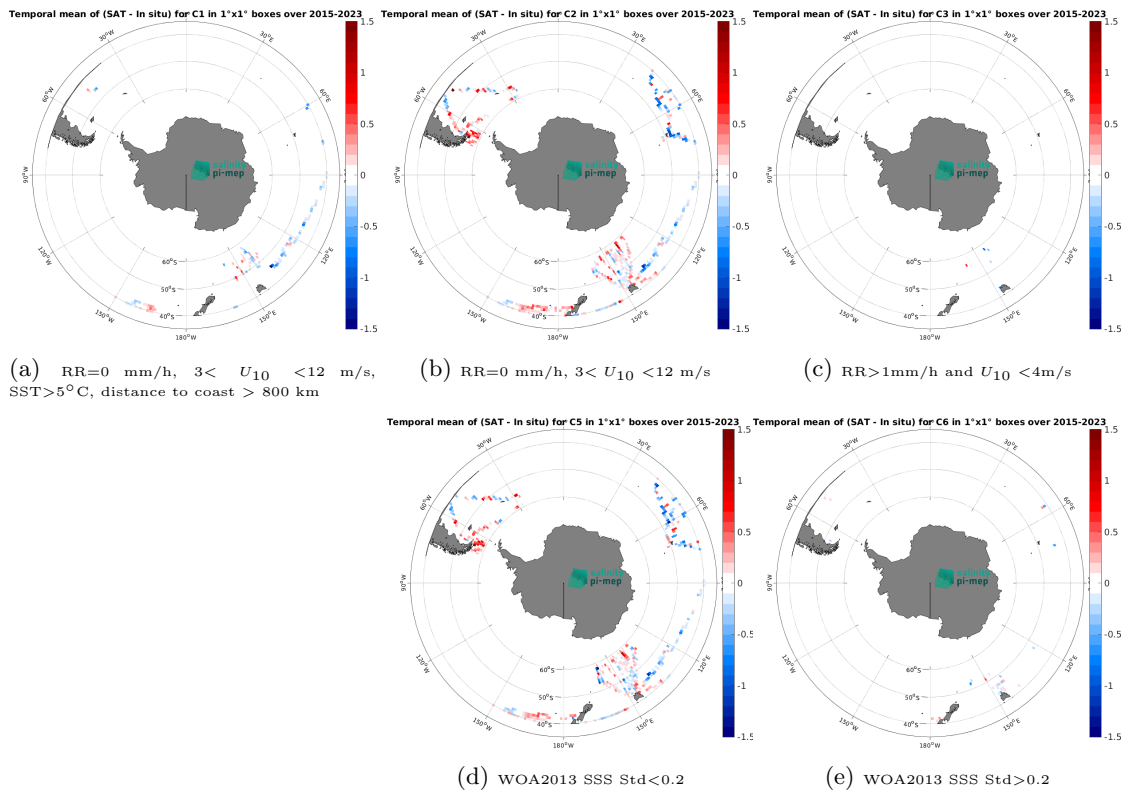
Figure 14: Temporal mean gridded over spatial boxes of size 1^\circ \times 1^\circ of \Delta SSS (SMAP SSS L3 v5.3 - 8-Day running (RSS) - TSG (LEGOS-DM)) for 5 different subdatasets corresponding to:RR=0 mm/h, 3 < U_{10} < 12 m/s, SST>5°C, distance to coast > 800 km (a), RR=0 mm/h, 3 < U_{10} < 12 m/s (b), RR>1mm/h and U_{10} < 4 m/s (c), WOA2013 SSS Std<0.2 (d), WOA2013 SSS Std>0.2 (e).
