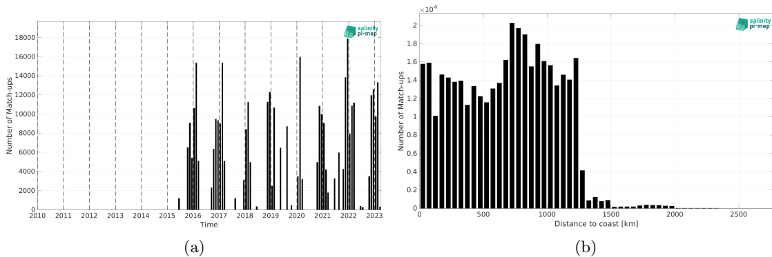
Figure 2: Number of match-ups between TSG (LEGOS-DM) and SMAP SSS L3 v5.3 - 8-Day running (RSS) SSS as a function of time (a) and as function of the distance to coast (b) over the Roaring Forties and Furious Fifties Pi-MEP region and for the full satellite product period.
