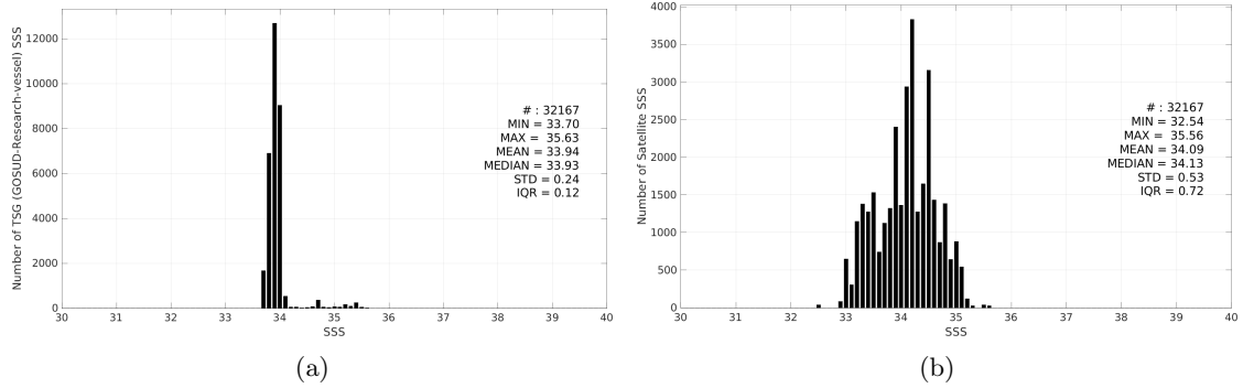
Figure 3: Histograms of SSS from TSG (GOSUD-Research-vessel) (a) and SMAP SSS L3 v5.3 - 8-Day running (RSS) (b) considering all match-up pairs per bins of 0.1 over the Roaring Forties and Furious Fifties Pi-MEP region and for the full satellite product period.
