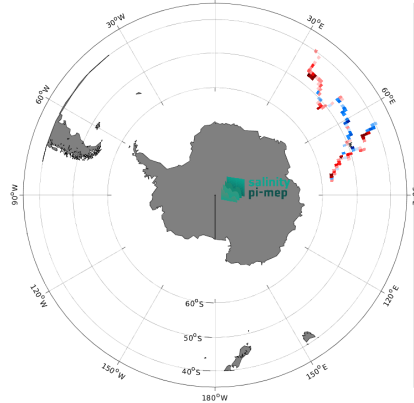
(e) MEAN( \Delta SSS) (Satellite - TSG (GOSUD-Research-vessel))
