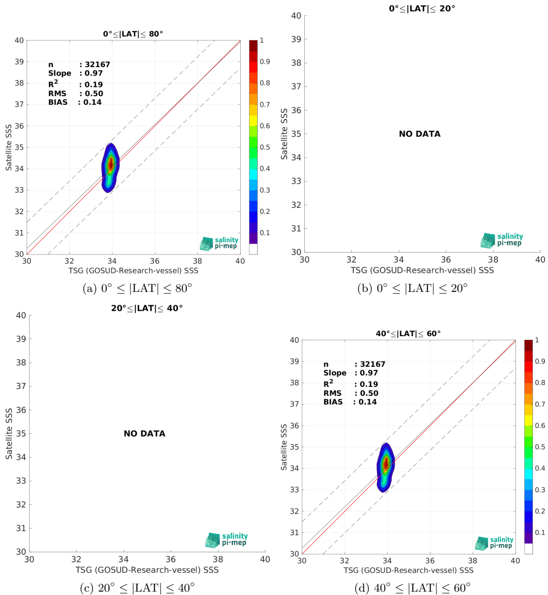
Figure 10: Contour maps of the concentration of SMAP SSS L3 v5.3 - 8-Day running (RSS) SSS (y-axis) versus TSG (GOSUD-Research-vessel) SSS (x-axis) at match-up pairs for different latitude bands. For each plot, the red line shows x=y . The black thin and dashed lines indicate a linear fit through the data cloud and the \pm 95\% confidence levels, respectively. The number match-up pairs n , the slope and R^2 coefficient of the linear fit, the root mean square (RMS) and the mean bias between satellite and in situ data are indicated for each latitude band in each plots.
