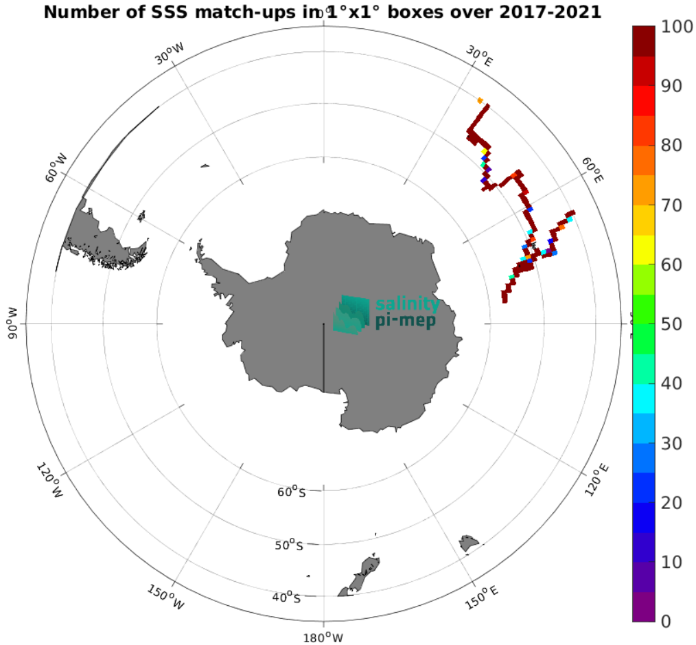
Figure 5: Number of SSS match-ups between TSG (GOSUD-Research-vessel) SSS and the SMAP SSS L3 v5.3 - 8-Day running (RSS) SSS product for the Roaring Forties and Furious Fifties Pi-MEP region over 1^\circ \times 1^\circ boxes and for the full satellite product period.
