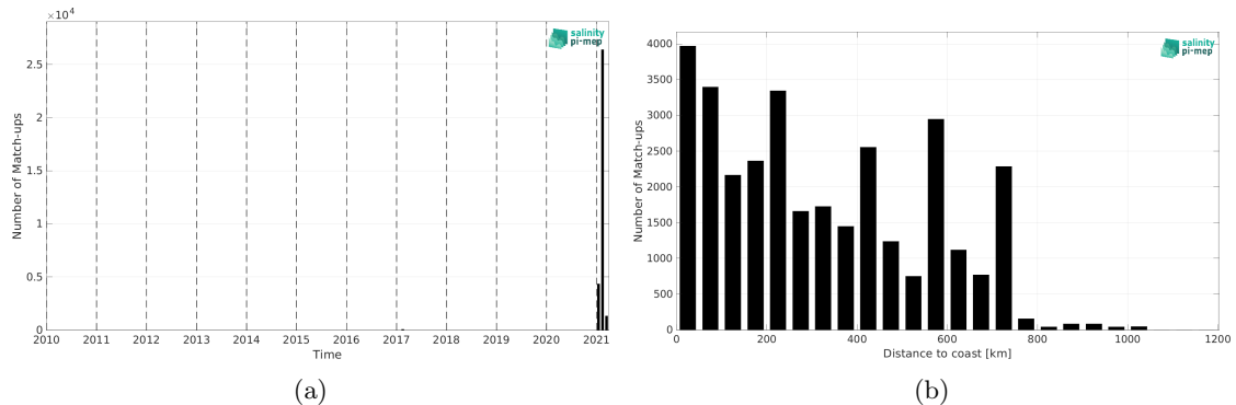
Figure 2: Number of match-ups between TSG (GOSUD-Research-vessel) and SMAP SSS L3 v5.3 - 8-Day running (RSS) SSS as a function of time (a) and as function of the distance to coast (b) over the Roaring Forties and Furious Fifties Pi-MEP region and for the full satellite product period.
