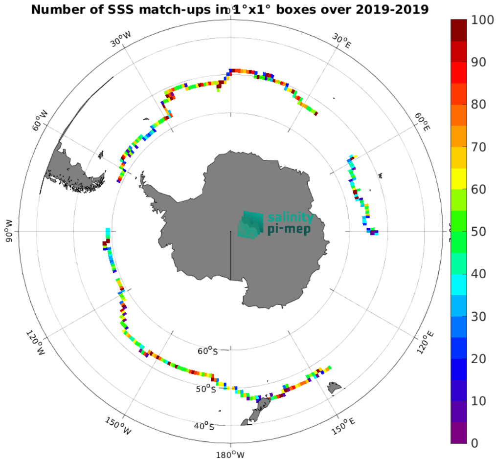
Figure 5: Number of SSS match-ups between Saildrone SSS and the SMAP SSS L3 v5.3 - 8-Day running (RSS) SSS product for the Roaring Forties and Furious Fifties Pi-MEP region over 1^\circ \times 1^\circ boxes and for the full satellite product period.
