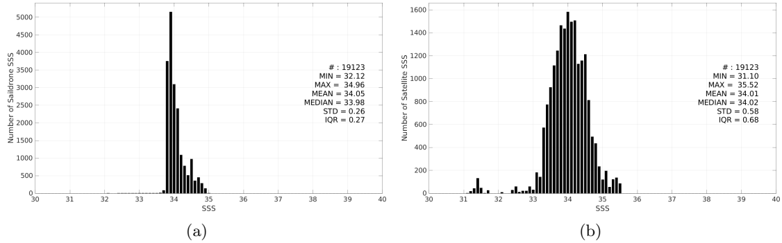
Figure 3: Histograms of SSS from Saildrone (a) and SMAP SSS L3 v5.3 - 8-Day running (RSS) (b) considering all match-up pairs per bins of 0.1 over the Roaring Forties and Furious Fifties Pi-MEP region and for the full satellite product period.
