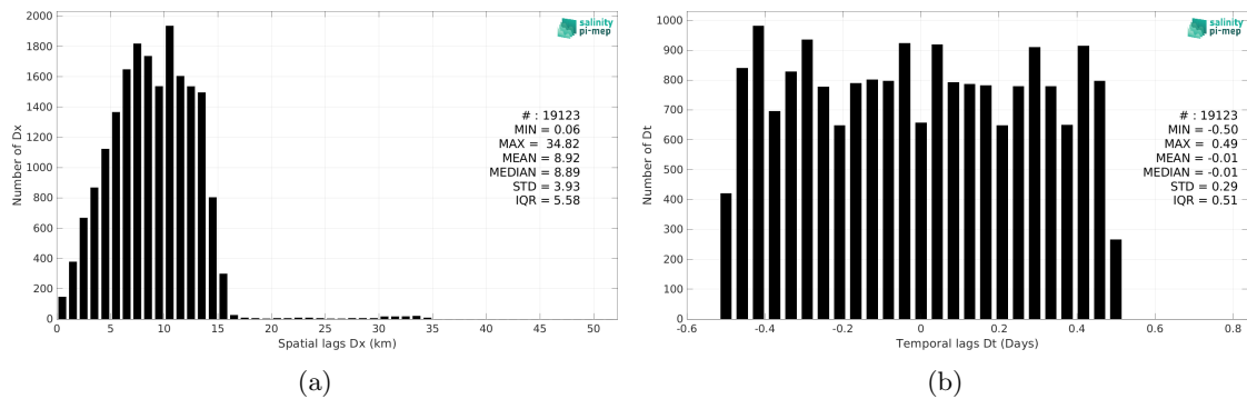
Figure 6: Histograms of the spatial (a) and temporal (b) lags between the location/time of the Sairdrone measurement and the date of the corresponding SMAP SSS L3 v5.3 - 8-Day running (RSS) SSS pixel.
