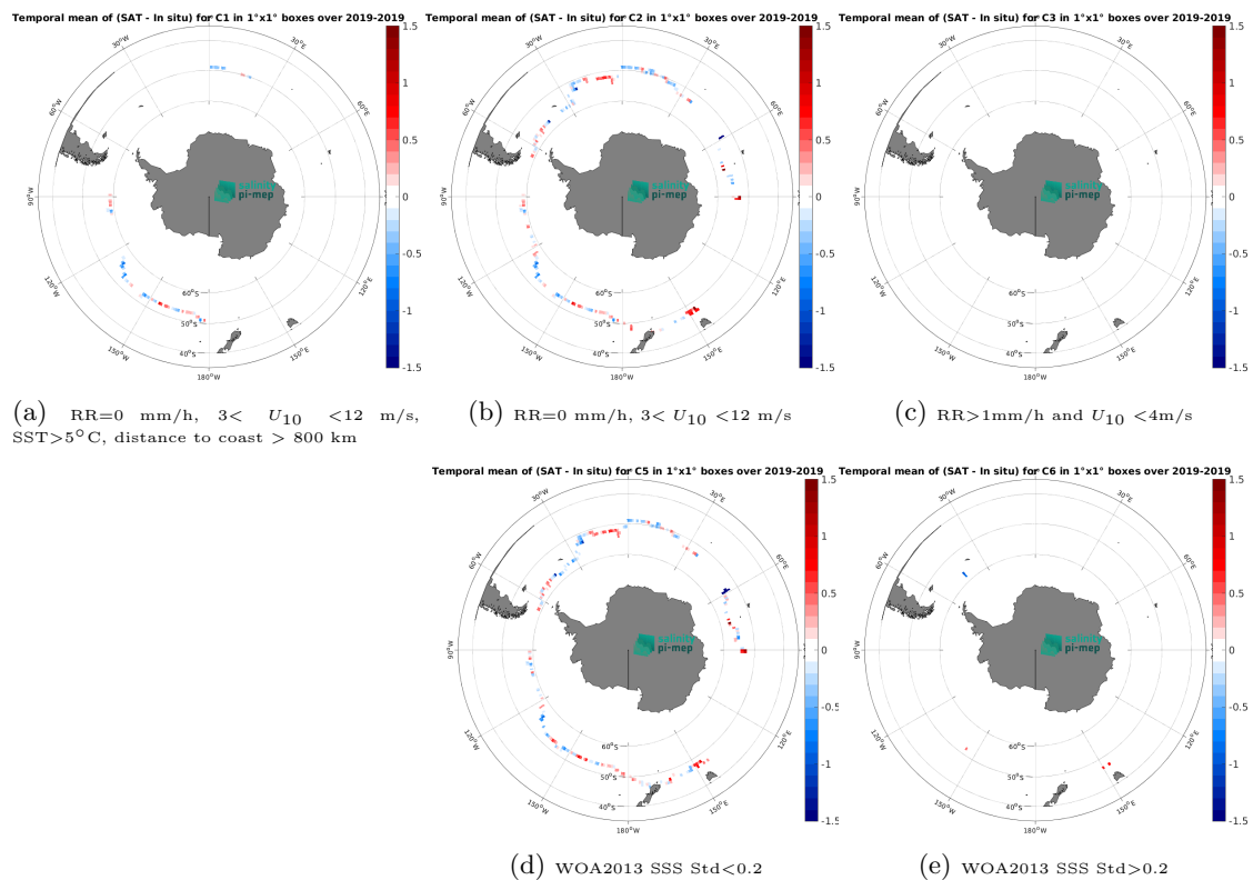
Figure 14: Temporal mean gridded over spatial boxes of size 1^\circ \times 1^\circ of \Delta SSS (SMAP SSS L3 v5.3 - 8-Day running (RSS) - Sailability) for 5 different subdatasets corresponding to:RR=0 mm/h, 3 < U_{10} < 12 m/s, SST >5^\circ\text{C} , distance to coast > 800 km (a), RR=0 mm/h, 3 < U_{10} < 12 m/s (b), RR >1 mm/h and U_{10} < 4 m/s (c), WOA2013 SSS Std <0.2 (d), WOA2013 SSS Std >0.2 (e).
