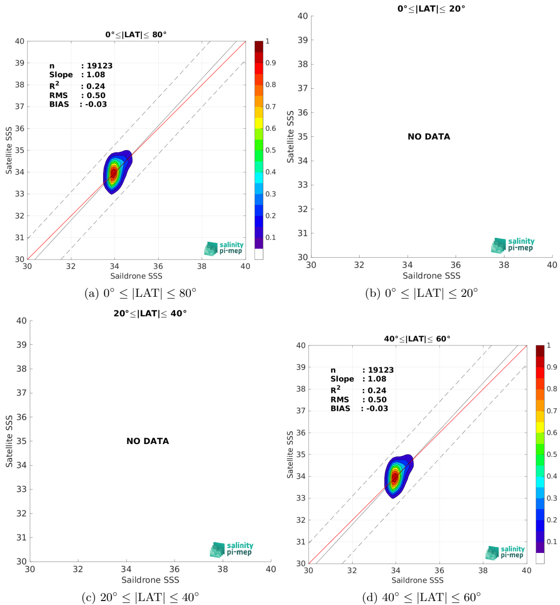
Figure 10: Contour maps of the concentration of SMAP SSS L3 v5.3 - 8-Day running (RSS) SSS (y-axis) versus Saildrone SSS (x-axis) at match-up pairs for different latitude bands. For each plot, the red line shows x=y . The black thin and dashed lines indicate a linear fit through the data cloud and the \pm 95\% confidence levels, respectively. The number match-up pairs n , the slope and R^2 coefficient of the linear fit, the root mean square (RMS) and the mean bias between satellite and in situ data are indicated for each latitude band in each plots.
