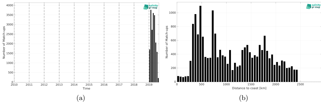
Figure 2: Number of match-ups between Saildrone and SMAP SSS L3 v5.3 - 8-Day running (RSS) SSS as a function of time (a) and as function of the distance to coast (b) over the Roaring Forties and Furious Fifties Pi-MEP region and for the full satellite product period.
