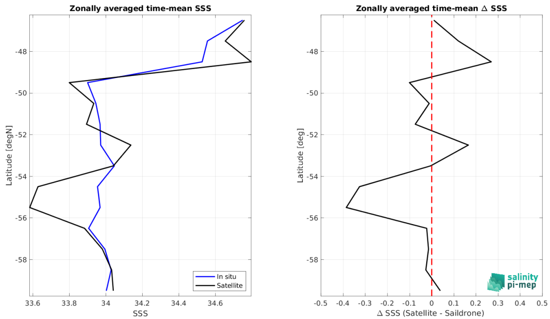
Figure 9: Left panel: Zonal mean SSS from SMAP SSS L3 v5.3 - 8-Day running (RSS) satellite product (black) and from Sairdron (blue). Right panel: Zonal mean of \Delta SSS (Satellite - Sairdron) for all the collected Pi-MEP match-up pairs estimated over the full satellite product period.
