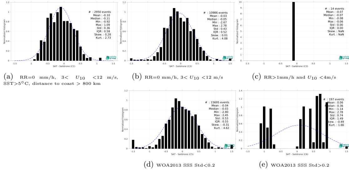
Figure 15: Normalized histogram of \Delta SSS (SMAP SSS L3 v5.3 - 8-Day running (RSS) - Saildrone) for 5 different subdatasets corresponding to: RR=0 mm/h, 3 < U_{10} < 12 m/s, SST > 5°C, distance to coast > 800 km (a), RR=0 mm/h, 3 < U_{10} < 12 m/s (b), RR > 1mm/h and U_{10} < 4 m/s (c), WOA2013 SSS Std < 0.2 (d), WOA2013 SSS Std > 0.2 (e).
