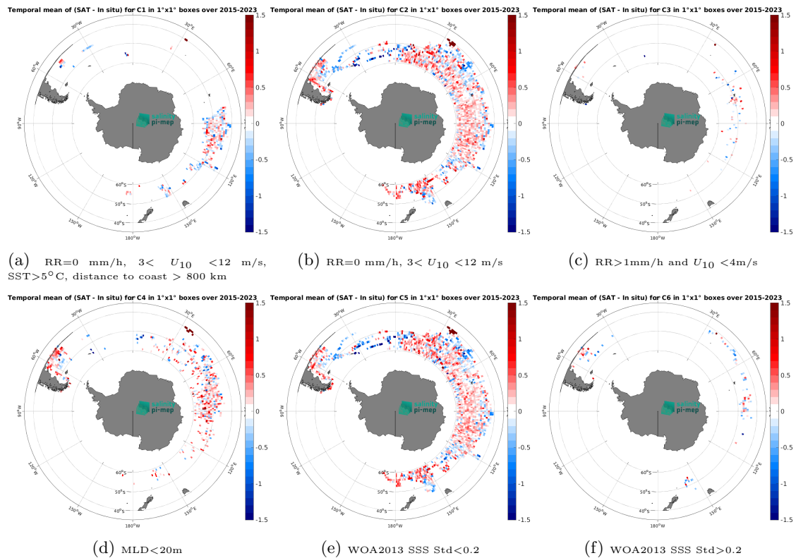
Figure 14: Temporal mean gridded over spatial boxes of size 1^\circ \times 1^\circ of \Delta SSS (SMAP SSS L3 v5.3 - 8-Day running (RSS) - Marine mammals) for 6 different subdatasets corresponding to:RR=0 mm/h, 3 < U_{10} < 12 m/s, SST > 5^\circ\text{C} , distance to coast > 800 km (a), RR=0 mm/h, 3 < U_{10} < 12 m/s (b), RR > 1 mm/h and U_{10} < 4 m/s (c),MLD < 20 m (d),WOA2013 SSS Std < 0.2 (e),WOA2013 SSS Std > 0.2 (f).
