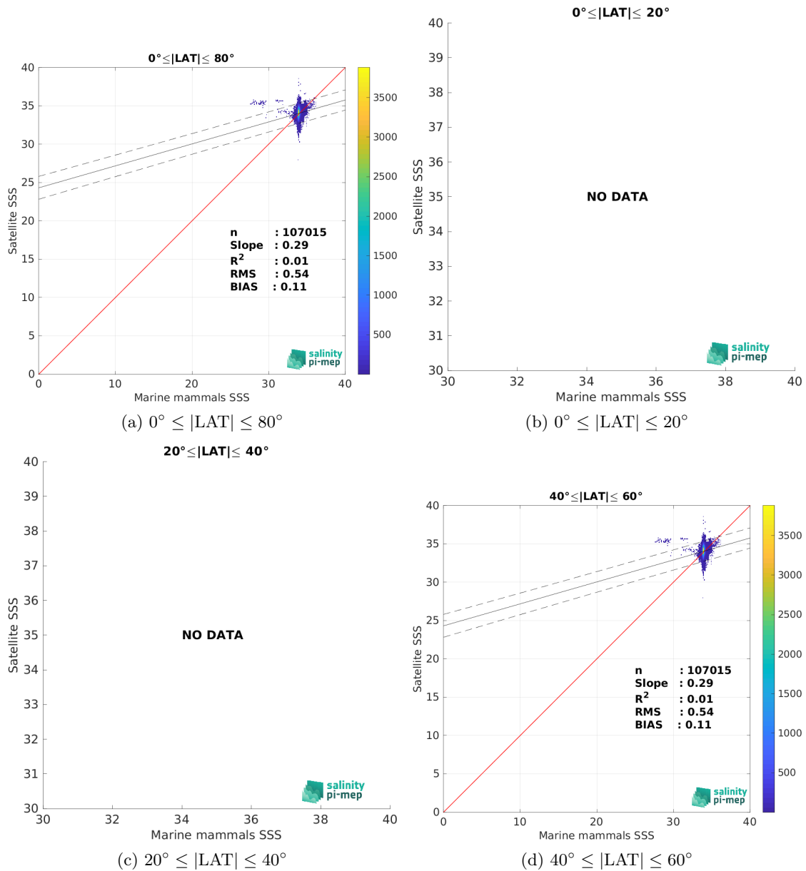
Figure 10: Contour maps of the concentration of SMAP SSS L3 v5.3 - 8-Day running (RSS) SSS (y-axis) versus Marine mammals SSS (x-axis) at match-up pairs for different latitude bands. For each plot, the red line shows x=y . The black thin and dashed lines indicate a linear fit through the data cloud and the \pm 95\% confidence levels, respectively. The number match-up pairs n , the slope and R^2 coefficient of the linear fit, the root mean square (RMS) and the mean bias between satellite and in situ data are indicated for each latitude band in each plots.
