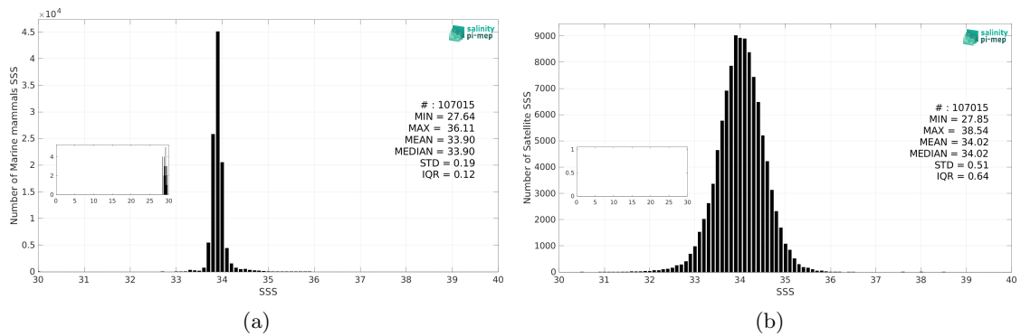
Figure 3: Histograms of SSS from Marine mammals (a) and SMAP SSS L3 v5.3 - 8-Day running (RSS) (b) considering all match-up pairs per bins of 0.1 over the Roaring Forties and Furious Fifties Pi-MEP region and for the full satellite product period.
