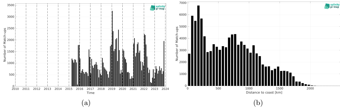
Figure 2: Number of match-ups between Marine mammals and SMAP SSS L3 v5.3 - 8-Day running (RSS) SSS as a function of time (a) and as function of the distance to coast (b) over the Roaring Forties and Furious Fifties Pi-MEP region and for the full satellite product period.
