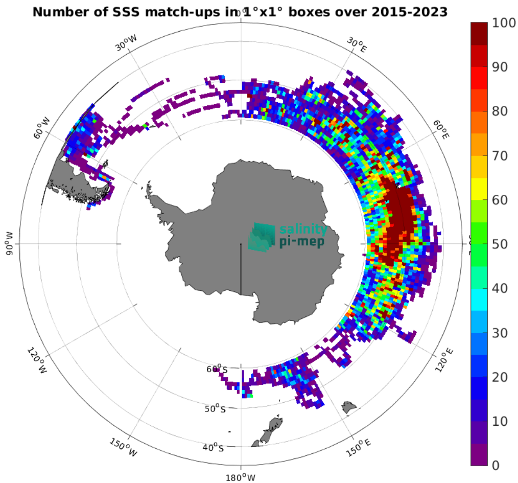
Figure 5: Number of SSS match-ups between Marine mammals SSS and the SMAP SSS L3 v5.3 - 8-Day running (RSS) SSS product for the Roaring Forties and Furious Fifties Pi-MEP region over 1^\circ \times 1^\circ boxes and for the full satellite product period.
