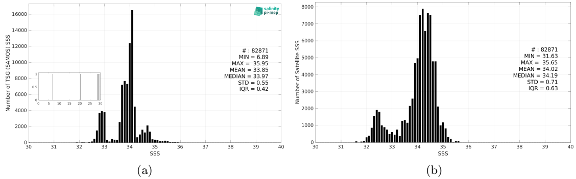
Figure 3: Histograms of SSS from TSG (SAMOS) (a) and SMAP SSS L3 v5.3 - Monthly (RSS) (b) considering all match-up pairs per bins of 0.1 over the Roaring Forties and Furious Fifties Pi-MEP region and for the full satellite product period.
