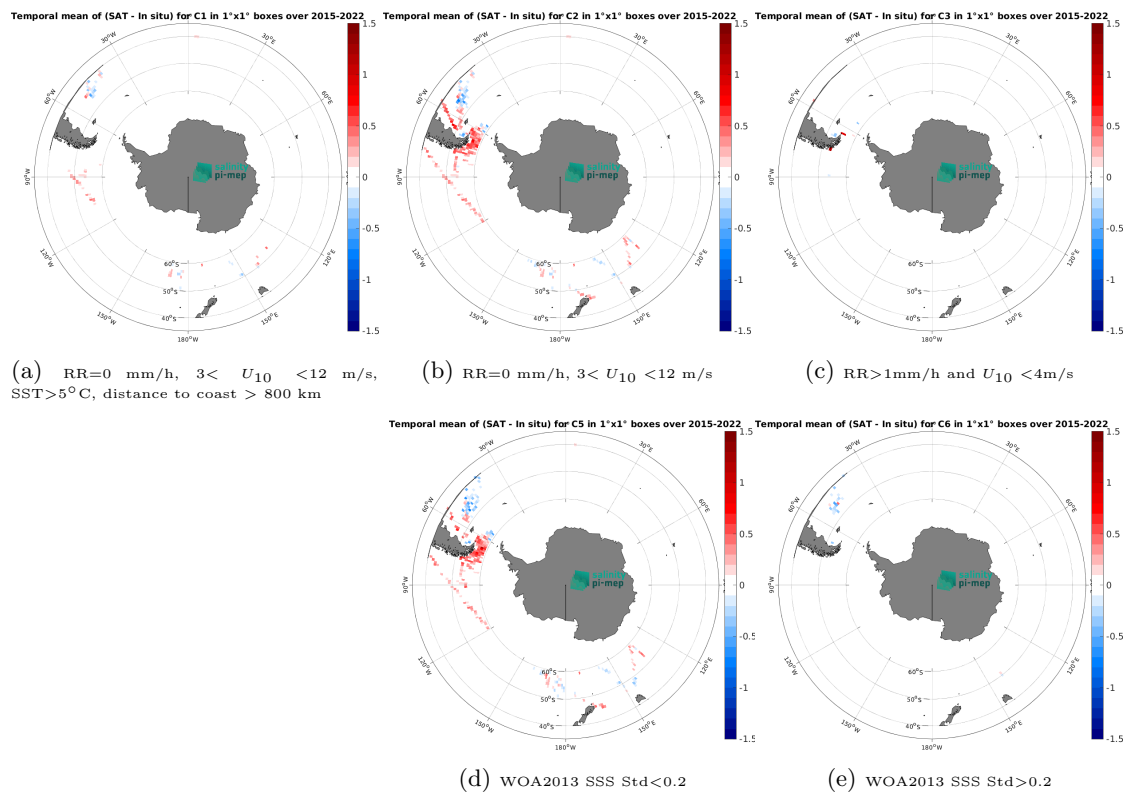
Figure 14: Temporal mean gridded over spatial boxes of size 1^\circ \times 1^\circ of \Delta SSS (SMAP SSS L3 v5.3 - Monthly (RSS) - TSG (SAMOS)) for 5 different subdatasets corresponding to:RR=0 mm/h, 3 < U_{10} < 12 m/s, SST>5°C, distance to coast > 800 km (a), RR=0 mm/h, 3 < U_{10} < 12 m/s (b), RR>1mm/h and U_{10} < 4 m/s (c), WOA2013 SSS Std<0.2 (d), WOA2013 SSS Std>0.2 (e).
