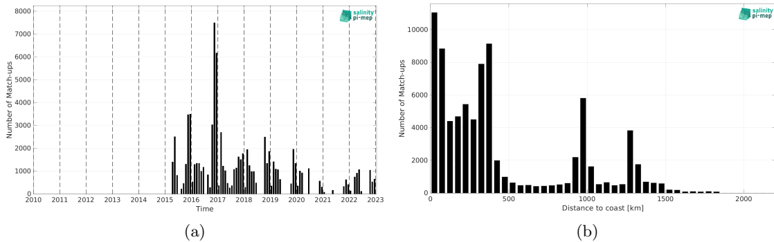
Figure 2: Number of match-ups between TSG (SAMOS) and SMAP SSS L3 v5.3 - Monthly (RSS) SSS as a function of time (a) and as function of the distance to coast (b) over the Roaring Forties and Furious Fifties Pi-MEP region and for the full satellite product period.
