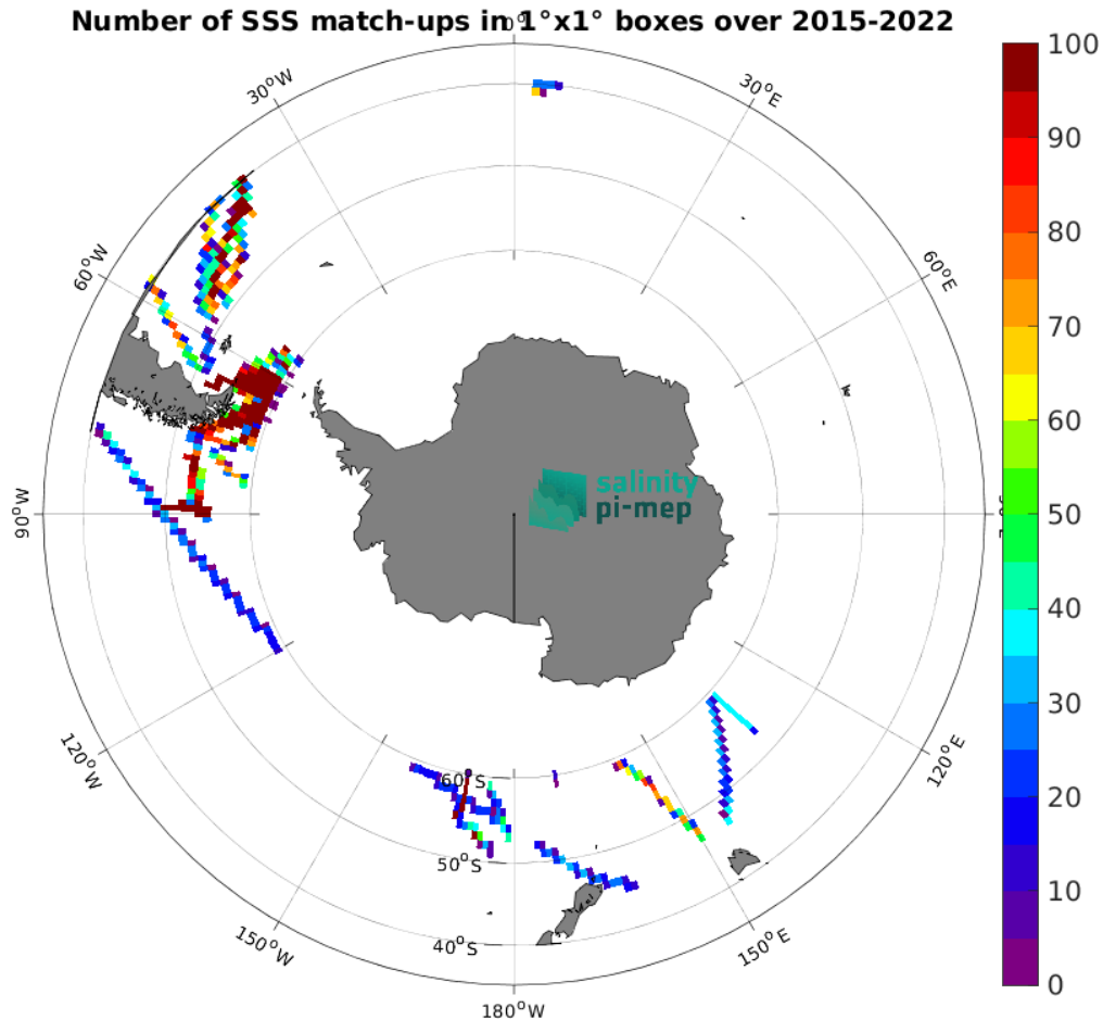
Figure 5: Number of SSS match-ups between TSG (SAMOS) SSS and the SMAP SSS L3 v5.3 - Monthly (RSS) SSS product for the Roaring Forties and Furious Fifties Pi-MEP region over 1^\circ \times 1^\circ boxes and for the full satellite product period.
