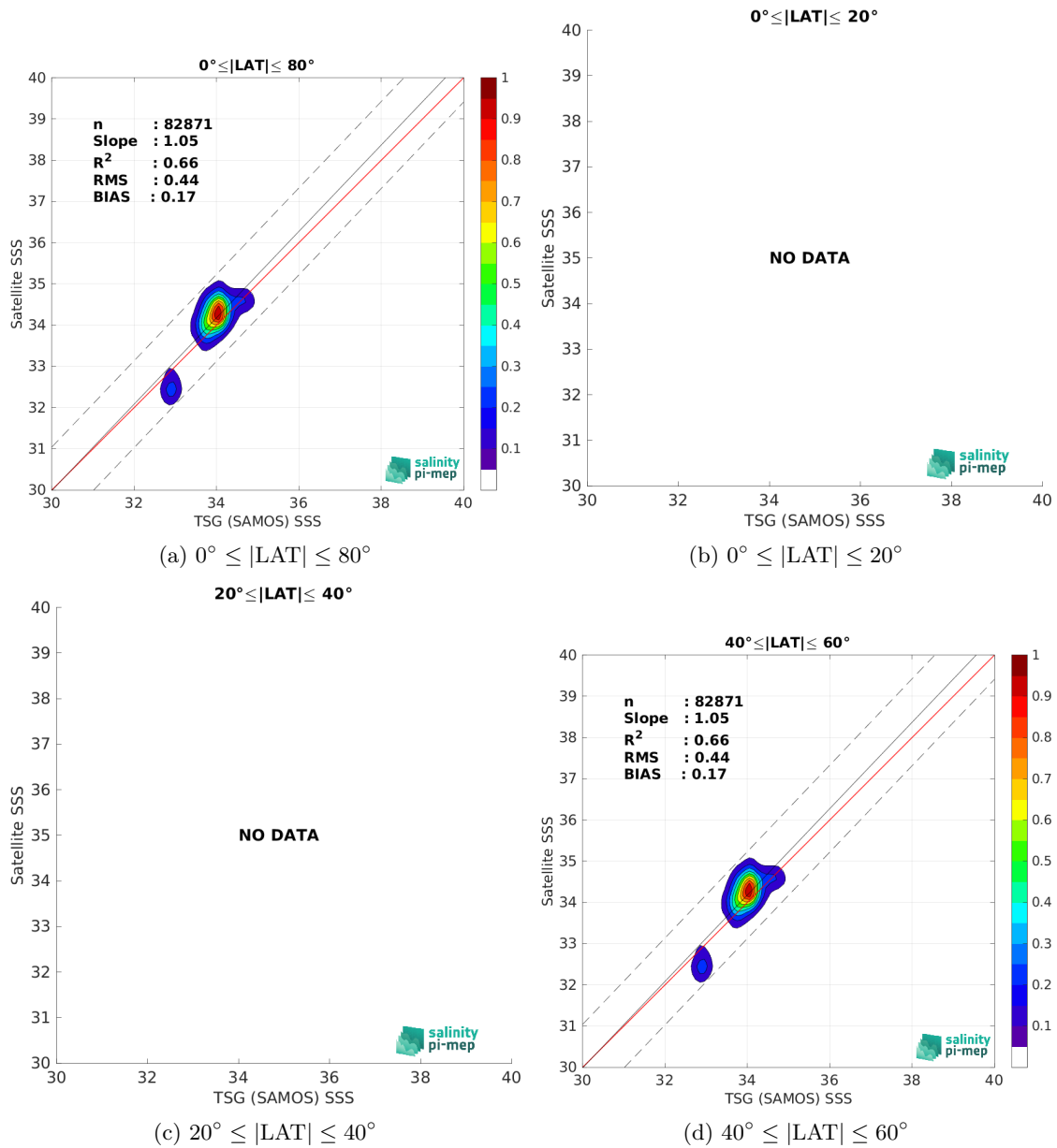
Figure 10: Contour maps of the concentration of SMAP SSS L3 v5.3 - Monthly (RSS) SSS (y-axis) versus TSG (SAMOS) SSS (x-axis) at match-up pairs for different latitude bands. For each plot, the red line shows x=y . The black thin and dashed lines indicate a linear fit through the data cloud and the \pm 95\% confidence levels, respectively. The number match-up pairs n , the slope and R^2 coefficient of the linear fit, the root mean square (RMS) and the mean bias between satellite and in situ data are indicated for each latitude band in each plot.
