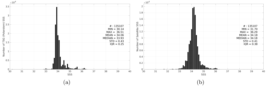
Figure 3: Histograms of SSS from TSG (Polarstern) (a) and SMAP SSS L3 v5.3 - Monthly (RSS) (b) considering all match-up pairs per bins of 0.1 over the Roaring Forties and Furious Fifties Pi-MEP region and for the full satellite product period.
