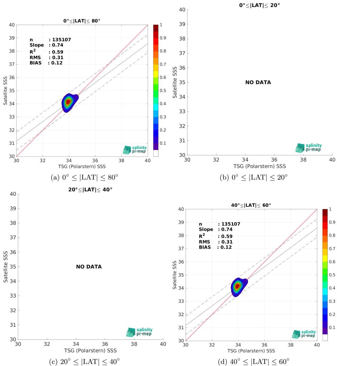
Figure 10: Contour maps of the concentration of SMAP SSS L3 v5.3 - Monthly (RSS) SSS (y-axis) versus TSG (Polarstern) SSS (x-axis) at match-up pairs for different latitude bands. For each plot, the red line shows x=y . The black thin and dashed lines indicate a linear fit through the data cloud and the \pm 95\% confidence levels, respectively. The number match-up pairs n , the slope and R^2 coefficient of the linear fit, the root mean square (RMS) and the mean bias between satellite and in situ data are indicated for each latitude band in each plots.
