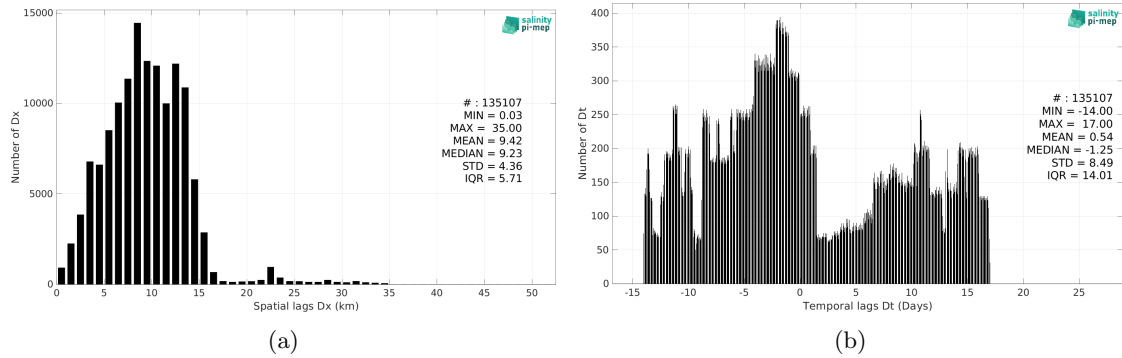
Figure 6: Histograms of the spatial (a) and temporal (b) lags between the location/time of the TSG (Polarstern) measurement and the date of the corresponding SMAP SSS L3 v5.3 - Monthly (RSS) SSS pixel.
