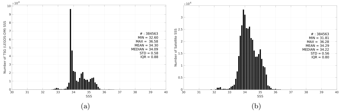
Figure 3: Histograms of SSS from TSG (LEGOS-DM) (a) and SMAP SSS L3 v5.3 - Monthly (RSS) (b) considering all match-up pairs per bins of 0.1 over the Roaring Forties and Furious Fifties Pi-MEP region and for the full satellite product period.
