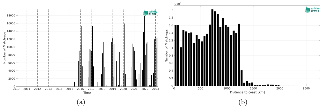
Figure 2: Number of match-ups between TSG (LEGOS-DM) and SMAP SSS L3 v5.3 - Monthly (RSS) SSS as a function of time (a) and as function of the distance to coast (b) over the Roaring Forties and Furious Fifties Pi-MEP region and for the full satellite product period.
