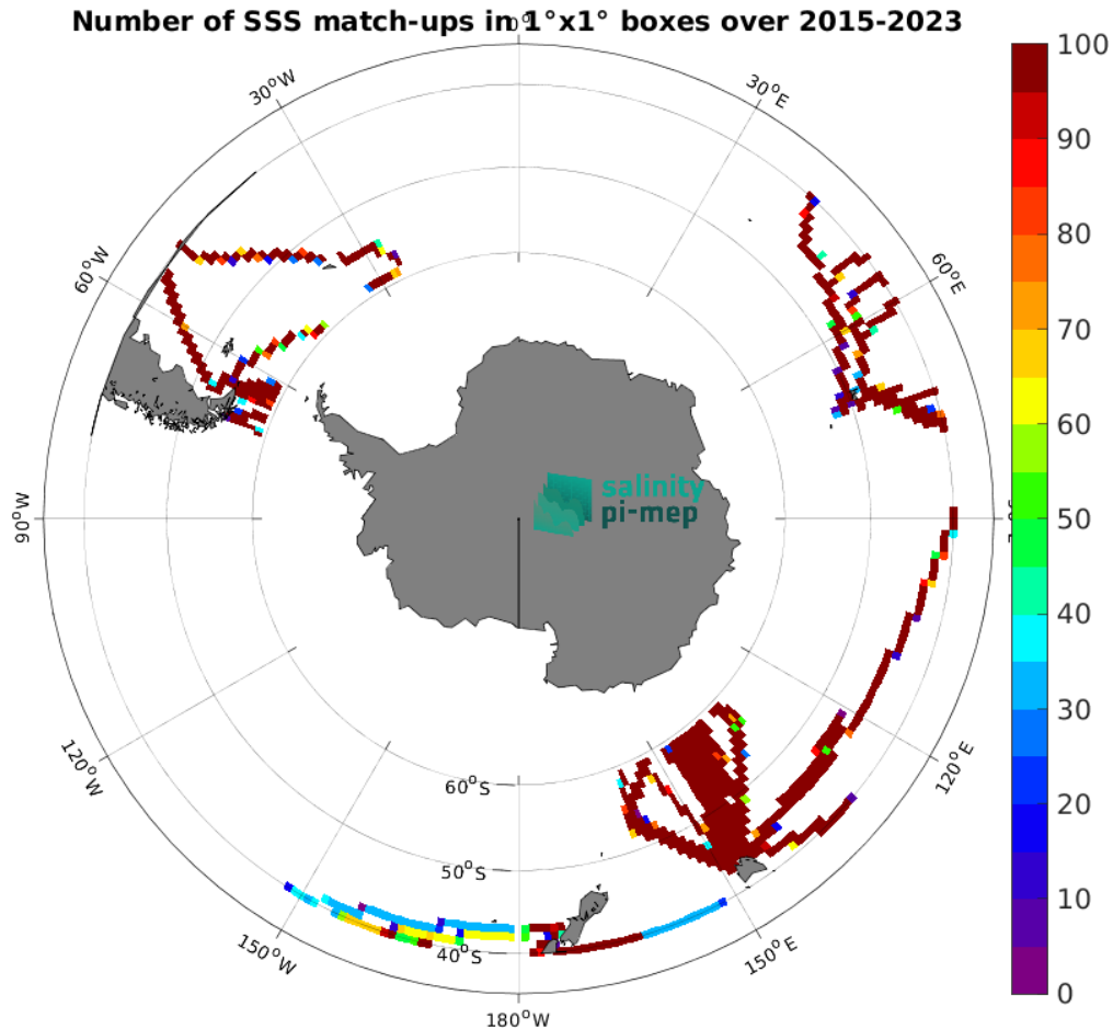
Figure 5: Number of SSS match-ups between TSG (LEGOS-DM) SSS and the SMAP SSS L3 v5.3 - Monthly (RSS) SSS product for the Roaring Forties and Furious Fifties Pi-MEP region over 1^\circ \times 1^\circ boxes and for the full satellite product period.
