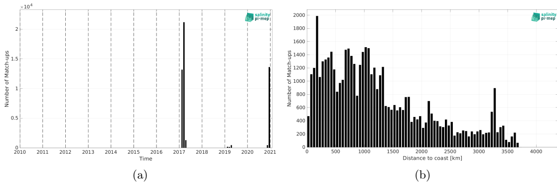
Figure 2: Number of match-ups between TSG (GOSUD-Sailing-ship) and SMAP SSS L3 v5.3 - Monthly (RSS) SSS as a function of time (a) and as function of the distance to coast (b) over the Roaring Forties and Furious Fifties Pi-MEP region and for the full satellite product period.
