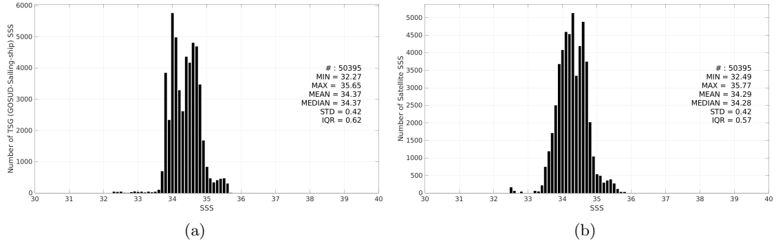
Figure 3: Histograms of SSS from TSG (GOSUD-Sailing-ship) (a) and SMAP SSS L3 v5.3 - Monthly (RSS) (b) considering all match-up pairs per bins of 0.1 over the Roaring Forties and Furious Fifties Pi-MEP region and for the full satellite product period.
