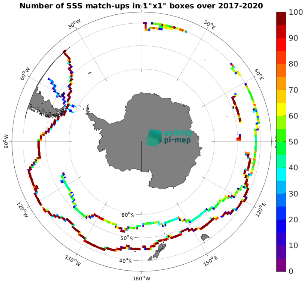
Figure 5: Number of SSS match-ups between TSG (GOSUD-Sailing-ship) SSS and the SMAP SSS L3 v5.3 - Monthly (RSS) SSS product for the Roaring Forties and Furious Fifties Pi-MEP region over 1^\circ \times 1^\circ boxes and for the full satellite product period.
