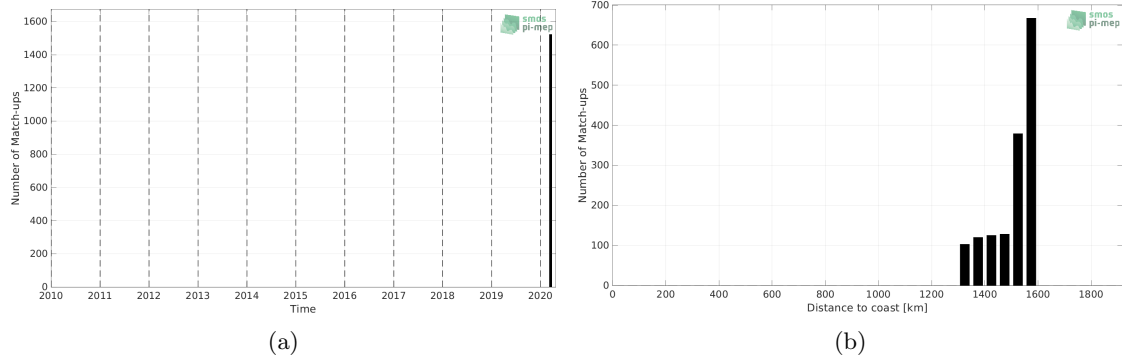
Figure 1: Number of match-ups between TSG (SAMOS) and SMAP SSS L3 v5 - 8-Day running (RSS) SSS as a function of time (a) and as function of the distance to coast (b) over the Roaring Forties and Furious Fifties Pi-MEP region and for the full satellite product period.
