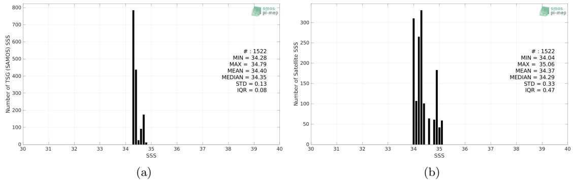
Figure 2: Histograms of SSS from TSG (SAMOS) (a) and SMAP SSS L3 v5 - 8-Day running (RSS) (b) considering all match-up pairs per bins of 0.1 over the Roaring Forties and Furious Fifties Pi-MEP region and for the full satellite product period.
